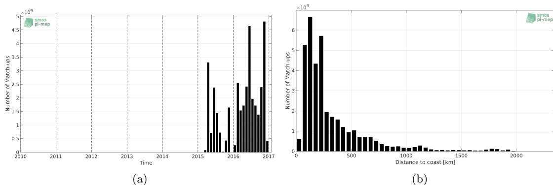
Figure 1: Number of match-ups between TSG-GOSUD-Research-vessel and SMAP-L3-RSS-V3-8DAY-RUNNING-70KM SSS as a function of time (a) and as function of the distance to coast (b) over the North Atlantic Ocean Pi-MEP region and for the full satellite product period.
