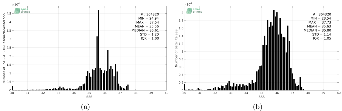
Figure 2: Histograms of SSS from TSG-GOSUD-Research-vessel (a) and SMAP-L3-RSS-V3-8DAY-RUNNING-70KM (b) considering all match-up pairs per bins of 0.1 over the North Atlantic Ocean Pi-MEP region and for the full satellite product period.
