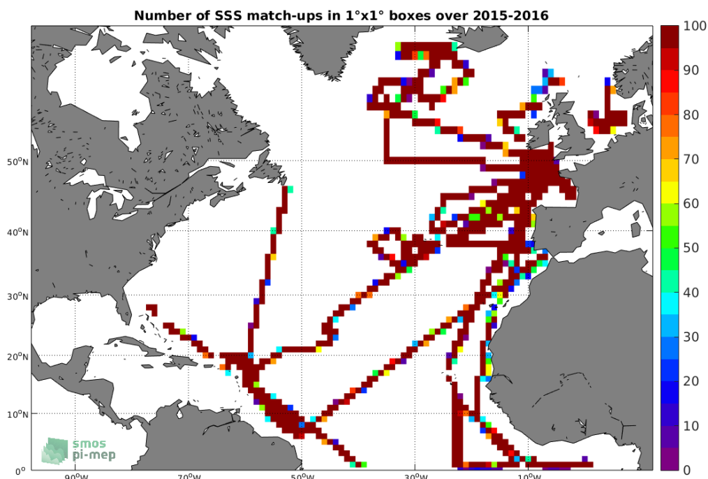
Figure 4: Number of SSS match-ups between TSG-GOSUD-Research-vessel SSS and the SMAP-L3-RSS-V3-8DAY-RUNNING-70KM SSS product for the North Atlantic Ocean Pi-MEP region over 1°x1° boxes and for the full satellite product period.
