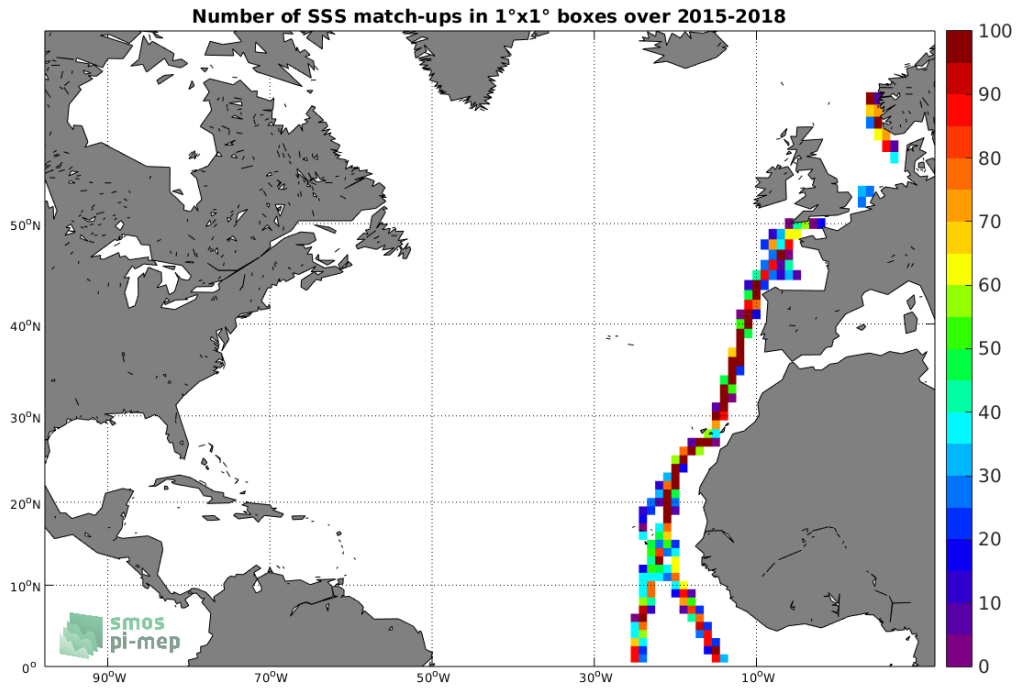
Figure 4: Number of SSS match-ups between TSG-POLARSTERN SSS and the SMAP-L3-RSS-V3-8DAY-RUNNING-40KM SSS product for the North Atlantic Ocean Pi-MEP region over 1^\circ \times 1^\circ boxes and for the full satellite product period.
