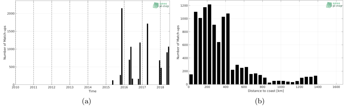
Figure 1: Number of match-ups between TSG-POLARSTERN and SMAP-L3-RSS-V3-8DAY-RUNNING-40KM SSS as a function of time (a) and as function of the distance to coast (b) over the North Atlantic Ocean Pi-MEP region and for the full satellite product period.
