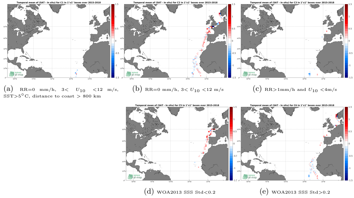
Figure 12: Temporal mean gridded over spatial boxes of size 1^\circ \times 1^\circ of \Delta SSS (SMAP-L3-RSS-V3-8DAY-RUNNING-40KM - TSG-POLARSTERN) for 5 different subdatasets corresponding to:RR=0 mm/h, 3 < U_{10} < 12 m/s, SST >5^\circ C, distance to coast > 800 km (a), RR=0 mm/h, 3 < U_{10} < 12 m/s (b), RR >1 mm/h and U_{10} < 4 m/s (c), WOA2013 SSS Std <0.2 (d), WOA2013 SSS Std >0.2 (e).
