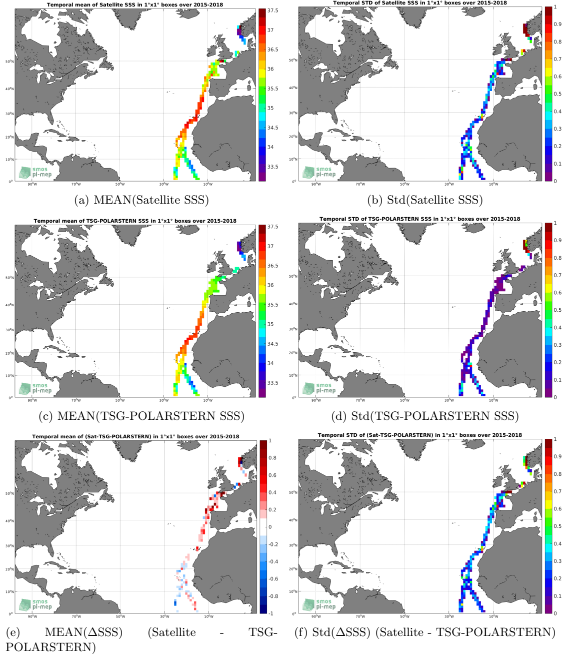
Figure 6: Temporal mean (left) and Std (right) of SSS from SMAP-L3-RSS-V3-8DAY-RUNNING-40KM (top), TSG-POLARSTERN (middle), and of \Delta SSS (Satellite - TSG-POLARSTERN). Only match-up pairs are used to generate these maps.
