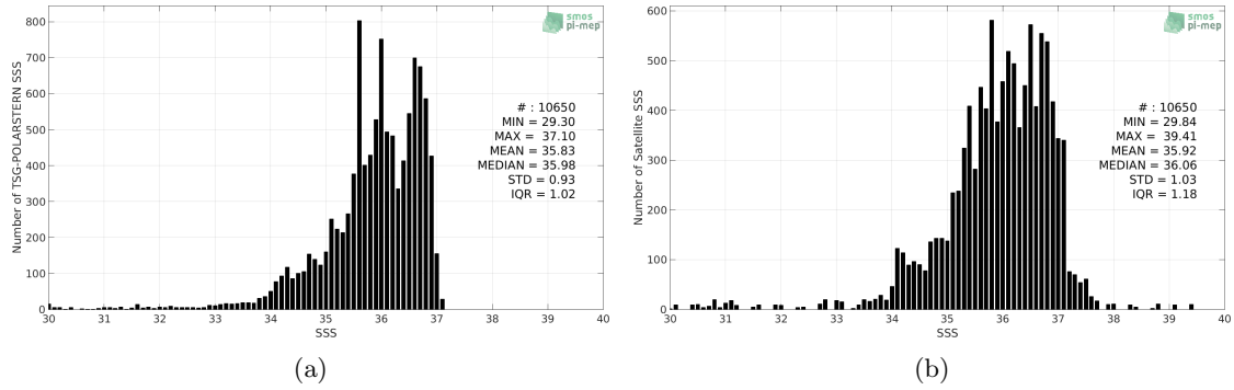
Figure 2: Histograms of SSS from TSG-POLARSTERN (a) and SMAP-L3-RSS-V3-8DAY-RUNNING-40KM (b) considering all match-up pairs per bins of 0.1 over the North Atlantic Ocean Pi-MEP region and for the full satellite product period.
