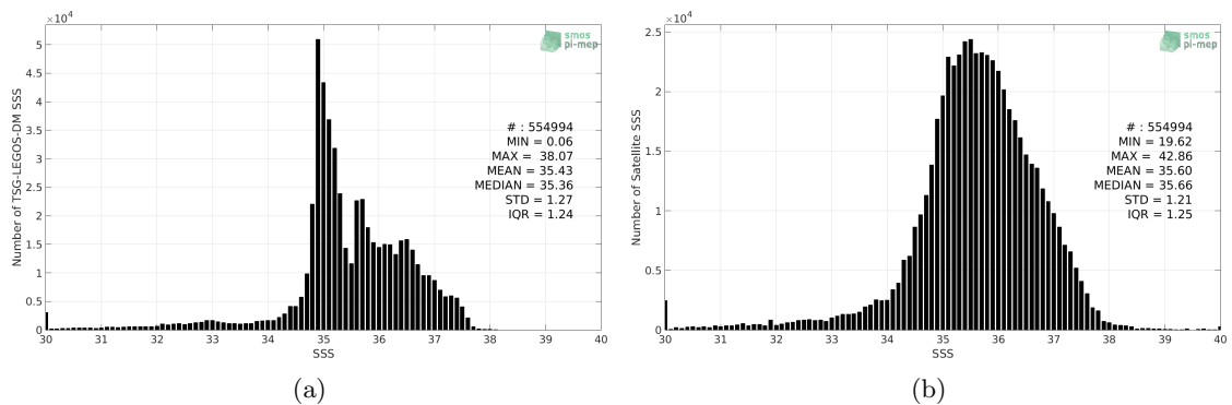
Figure 2: Histograms of SSS from TSG-LEGOS-DM (a) and SMAP-L3-RSS-V3-8DAY-RUNNING-40KM (b) considering all match-up pairs per bins of 0.1 over the North Atlantic Ocean Pi-MEP region and for the full satellite product period.
