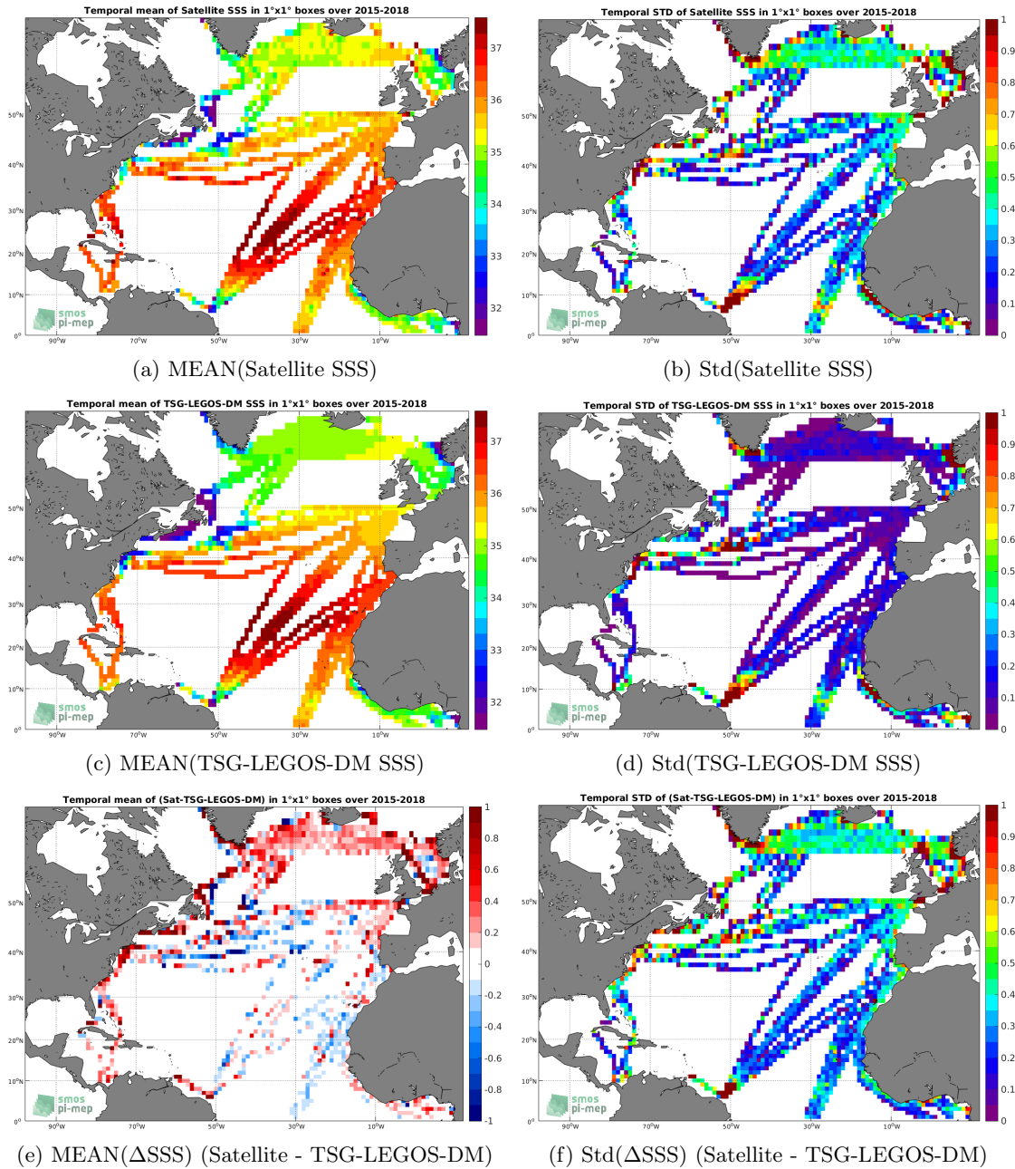
Figure 6: Temporal mean (left) and Std (right) of SSS from SMAP-L3-RSS-V3-8DAY-RUNNING-40KM (top), TSG-LEGOS-DM (middle), and of \Delta SSS (Satellite - TSG-LEGOS-DM). Only match-up pairs are used to generate these maps.
