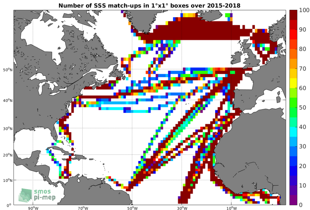
Figure 4: Number of SSS match-ups between TSG-LEGOS-DM SSS and the SMAP-L3-RSS-V3-8DAY-RUNNING-40KM SSS product for the North Atlantic Ocean Pi-MEP region over 1^\circ \times 1^\circ boxes and for the full satellite product period.
