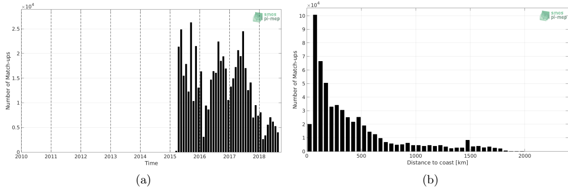
Figure 1: Number of match-ups between TSG-LEGOS-DM and SMAP-L3-RSS-V3-8DAY-RUNNING-40KM SSS as a function of time (a) and as function of the distance to coast (b) over the North Atlantic Ocean Pi-MEP region and for the full satellite product period.
