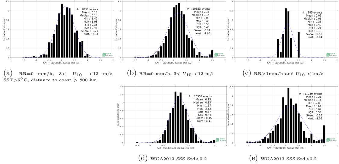
Figure 13: Normalized histogram of \Delta SSS (SMAP-L3-RSS-V3-8DAY-RUNNING-40KM - TSG-GOSUD-Sailing-ship) for 5 different subdatasets corresponding to: RR=0 mm/h, 3 < U_{10} < 12 m/s, SST > 5^\circ C , distance to coast > 800 km (a), RR=0 mm/h, 3 < U_{10} < 12 m/s (b), RR > 1 mm/h and U_{10} < 4 m/s (c), WOA2013 SSS Std < 0.2 (d), WOA2013 SSS Std > 0.2 (e).
