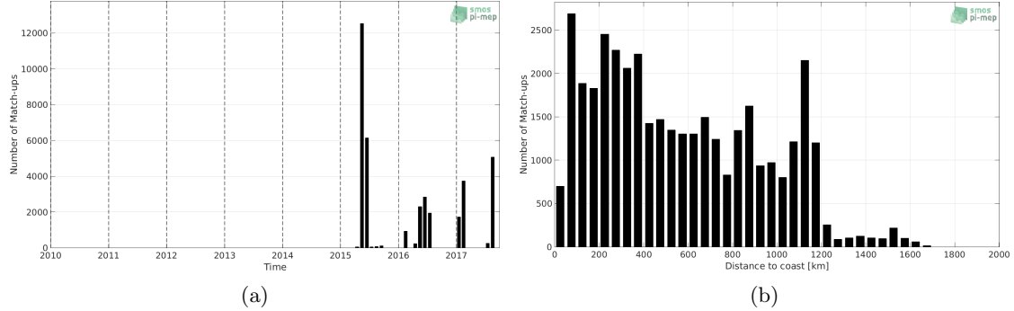
Figure 1: Number of match-ups between TSG-GOSUD-Sailing-ship and SMAP-L3-RSS-V3-8DAY-RUNNING-40KM SSS as a function of time (a) and as function of the distance to coast (b) over the North Atlantic Ocean Pi-MEP region and for the full satellite product period.
