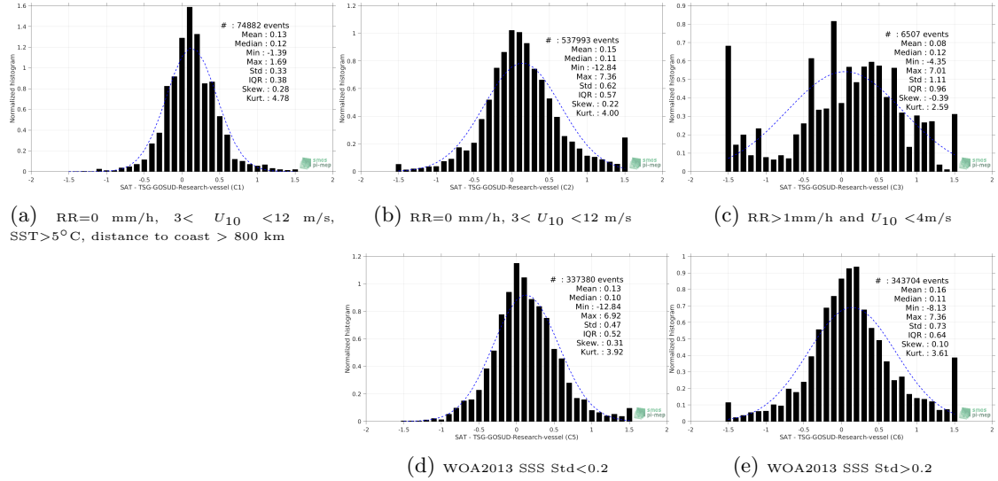
Figure 13: Normalized histogram of \Delta SSS (SMAP-L3-RSS-V3-8DAY-RUNNING-40KM - TSG-GOSUD-Research-vessel) for 5 different subdatasets corresponding to: RR=0 mm/h, 3 < U_{10} < 12 m/s, SST > 5°C, distance to coast > 800 km (a), RR=0 mm/h, 3 < U_{10} < 12 m/s (b), RR > 1mm/h and U_{10} < 4 m/s (c), WOA2013 SSS Std < 0.2 (d), WOA2013 SSS Std > 0.2 (e).
