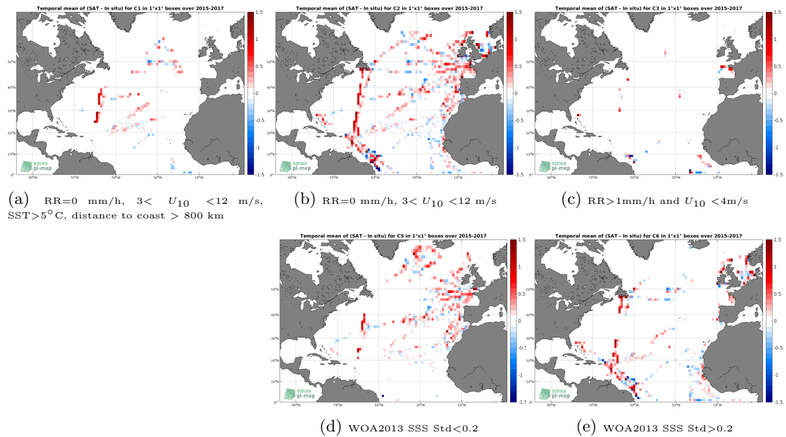
Figure 12: Temporal mean gridded over spatial boxes of size 1^\circ \times 1^\circ of \Delta SSS (SMAP-L3-RSS-V3-8DAY-RUNNING-40KM - TSG-GOSUD-Research-vessel) for 5 different subdatasets corresponding to:RR=0 mm/h, 3 < U_{10} < 12 m/s, SST >5^\circ C, distance to coast > 800 km (a), RR=0 mm/h, 3 < U_{10} < 12 m/s (b), RR >1 mm/h and U_{10} < 4 m/s (c), WOA2013 SSS Std <0.2 (d), WOA2013 SSS Std >0.2 (e).
