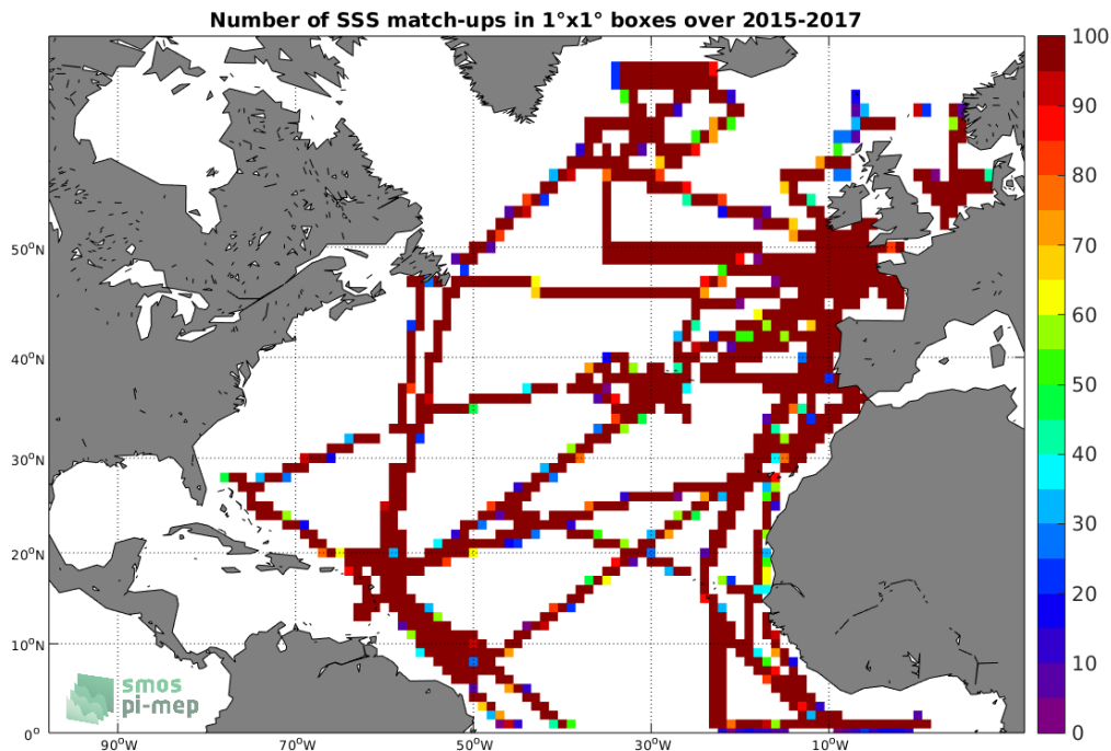
Figure 4: Number of SSS match-ups between TSG-GOSUD-Research-vessel SSS and the SMAP-L3-RSS-V3-8DAY-RUNNING-40KM SSS product for the North Atlantic Ocean Pi-MEP region over 1^\circ \times 1^\circ boxes and for the full satellite product period.
