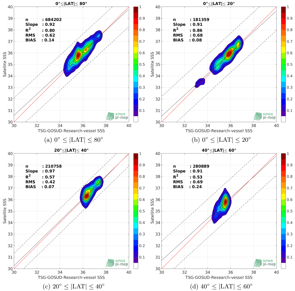
Figure 9: Contour maps of the concentration of SMAP-L3-RSS-V3-8DAY-RUNNING-40KM SSS (y-axis) versus TSG-GOSUD-Research-vessel SSS (x-axis) at match-up pairs for different latitude bands. For each plot, the red line shows x=y . The black thin and dashed lines indicate a linear fit through the data cloud and the \pm 95\% confidence levels, respectively. The number match-up pairs n , the slope and R^2 coefficient of the linear fit, the root mean square (RMS) and the mean bias between satellite and in situ data are indicated for each latitude band in each plots.
