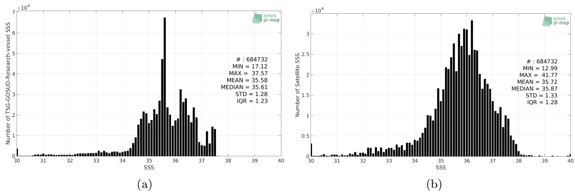
Figure 2: Histograms of SSS from TSG-GOSUD-Research-vessel (a) and SMAP-L3-RSS-V3-8DAY-RUNNING-40KM (b) considering all match-up pairs per bins of 0.1 over the North Atlantic Ocean Pi-MEP region and for the full satellite product period.
