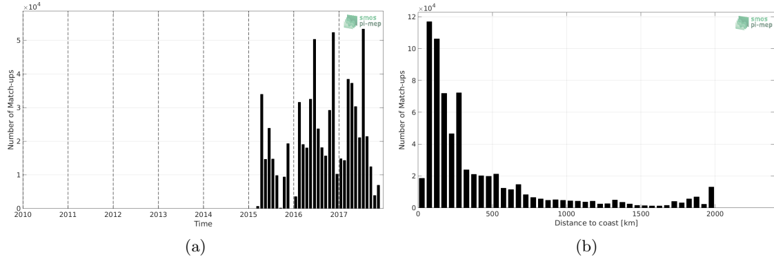
Figure 1: Number of match-ups between TSG-GOSUD-Research-vessel and SMAP-L3-RSS-V3-8DAY-RUNNING-40KM SSS as a function of time (a) and as function of the distance to coast (b) over the North Atlantic Ocean Pi-MEP region and for the full satellite product period.
