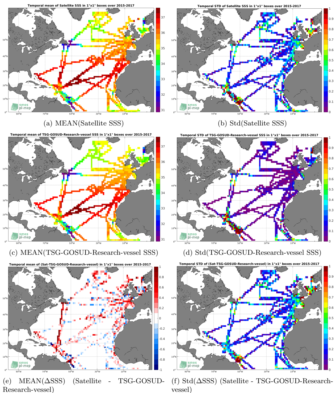
Figure 6: Temporal mean (left) and Std (right) of SSS from SMAP-L3-RSS-V3-8DAY-RUNNING-40KM (top), TSG-GOSUD-Research-vessel (middle), and of \Delta SSS (Satellite - TSG-GOSUD-Research-vessel). Only match-up pairs are used to generate these maps.
