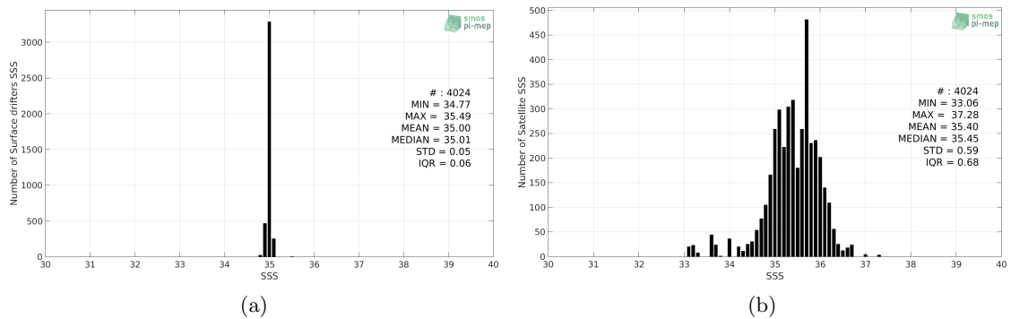
Figure 2: Histograms of SSS from Surface drifters (a) and SMAP-L3-RSS-V3-8DAY-RUNNING-40KM (b) considering all match-up pairs per bins of 0.1 over the North Atlantic Ocean Pi-MEP region and for the full satellite product period.
