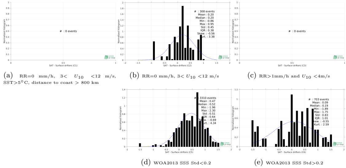
Figure 12: Normalized histogram of \Delta SSS (SMAP-L3-RSS-V3-8DAY-RUNNING-40KM - Surface drifters) for 5 different subdatasets corresponding to: RR=0 mm/h, 3 < U_{10} < 12 m/s, SST > 5°C, distance to coast > 800 km (a), RR=0 mm/h, 3 < U_{10} < 12 m/s (b), RR > 1mm/h and U_{10} < 4 m/s (c), WOA2013 SSS Std < 0.2 (d), WOA2013 SSS Std > 0.2 (e).
