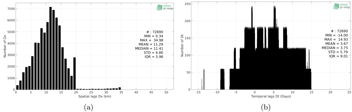
Figure 5: Histograms of the spatial (a) and temporal (b) lags between the time of the TSG-SAMOS measurements and the date of the corresponding SMAP-L3-RSS-V3-MONTHLY-70KM SSS product.
