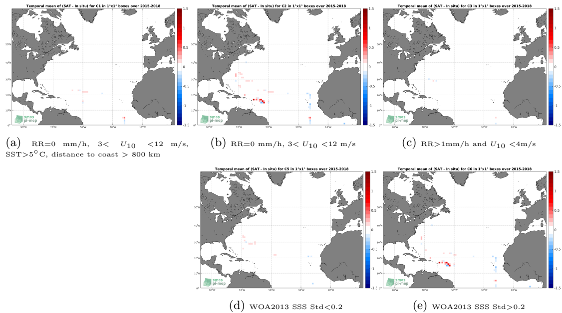
Figure 12: Temporal mean gridded over spatial boxes of size 1^\circ \times 1^\circ of \Delta SSS (SMAP-L3-RSS-V3-MONTHLY-70KM - TSG-SAMOS) for 5 different subdatasets corresponding to:RR=0 mm/h, 3 < U_{10} < 12 m/s, SST >5^\circ C, distance to coast > 800 km (a), RR=0 mm/h, 3 < U_{10} < 12 m/s (b), RR >1 mm/h and U_{10} < 4 m/s (c), WOA2013 SSS Std <0.2 (d), WOA2013 SSS Std >0.2 (e).
