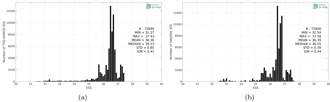
Figure 2: Histograms of SSS from TSG-SAMOS (a) and SMAP-L3-RSS-V3-MONTHLY-70KM (b) considering all match-up pairs per bins of 0.1 over the North Atlantic Ocean Pi-MEP region and for the full satellite product period.
