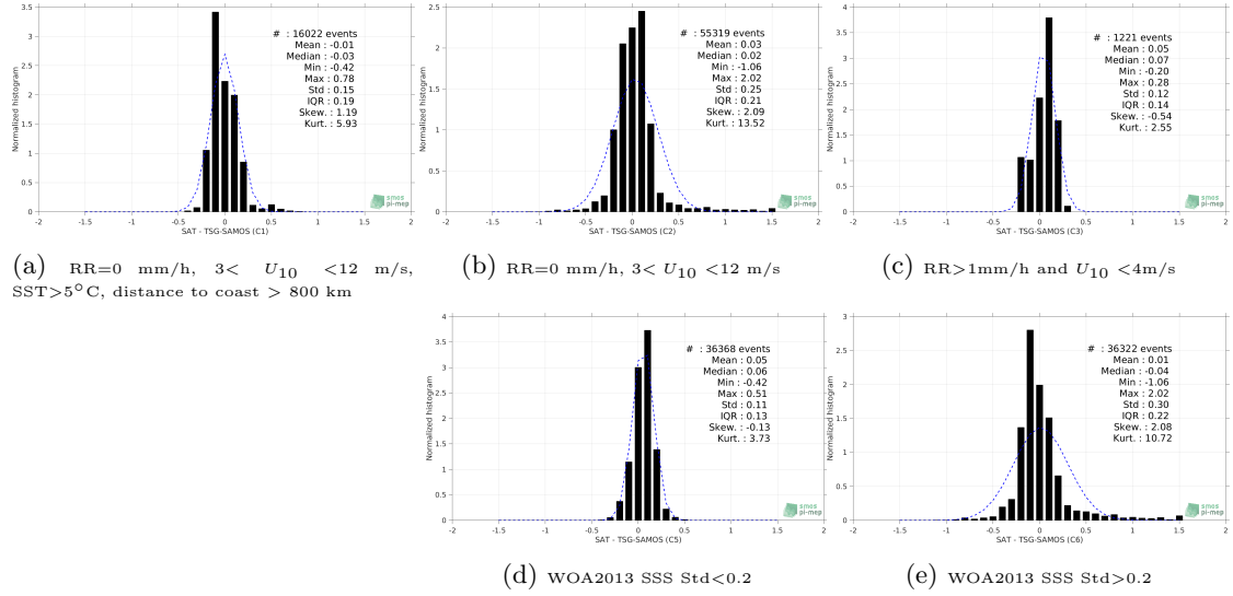
Figure 13: Normalized histogram of \Delta SSS (SMAP-L3-RSS-V3-MONTHLY-70KM - TSG-SAMOS) for 5 different subdatasets corresponding to: RR=0 mm/h, 3 < U_{10} < 12 m/s, SST > 5°C, distance to coast > 800 km (a), RR=0 mm/h, 3 < U_{10} < 12 m/s (b), RR > 1mm/h and U_{10} < 4 m/s (c), WOA2013 SSS Std < 0.2 (d), WOA2013 SSS Std > 0.2 (e).
