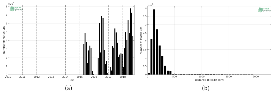
Figure 1: Number of match-ups between TSG-SAMOS and SMAP-L3-RSS-V3-MONTHLY-70KM SSS as a function of time (a) and as function of the distance to coast (b) over the North Atlantic Ocean Pi-MEP region and for the full satellite product period.
