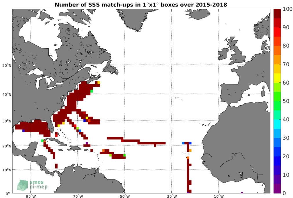
Figure 4: Number of SSS match-ups between TSG-SAMOS SSS and the SMAP-L3-RSS-V3-MONTHLY-70KM SSS product for the North Atlantic Ocean Pi-MEP region over 1^\circ \times 1^\circ boxes and for the full satellite product period.
