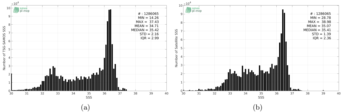
Figure 2: Histograms of SSS from TSG-SAMOS (a) and SMAP-L3-RSS-V3-MONTHLY-70KM (b) considering all match-up pairs per bins of 0.1 over the North Atlantic Ocean Pi-MEP region and for the full satellite product period.
