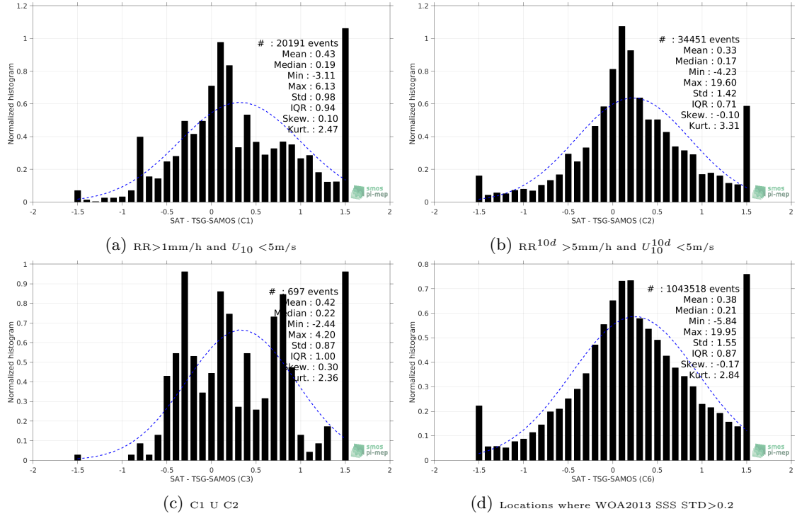
Figure 13: Normalized histogram of \Delta SSS (SMAP-L3-RSS-V3-MONTHLY-70KM - TSG-SAMOS) for 6 different subdatasets corresponding to: RR > 1mm/h and U_{10} < 5 m/s (a), RR^{10d} > 5 mm/h and U_{10}^{10d} < 5 m/s (b), C1 U C2 (c), Locations where WOA2013 SSS STD > 0.2 (d).
