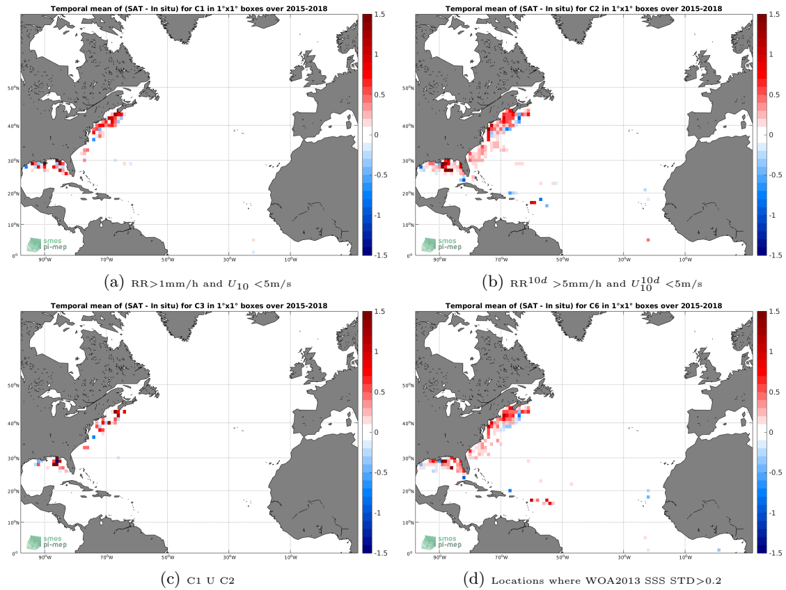
Figure 12: Temporal mean gridded over spatial boxes of size 1^\circ \times 1^\circ of \Delta SSS (SMAP-L3-RSS-V3-MONTHLY-70KM - TSG-SAMOS) for 4 different subdatasets corresponding to: RR > 1mm/h and U_{10} < 5 m/s (a), RR^{10d} > 5 mm/h and U_{10}^{10d} < 5 m/s (b), C1 U C2 (c), Locations where WOA2013 SSS STD > 0.2 (d).
