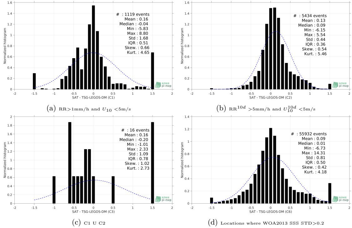
Figure 13: Normalized histogram of \Delta\text{SSS} (SMAP-L3-RSS-V3-MONTHLY-70KM - TSG-LEGOS-DM) for 6 different subdatasets corresponding to: RR > 1mm/h and U_{10} < 5\text{m/s} (a), \text{RR}^{10d} > 5\text{mm/h} and U_{10}^{10d} < 5\text{m/s} (b), C1 U C2 (c), Locations where WOA2013 SSS STD > 0.2 (d).
