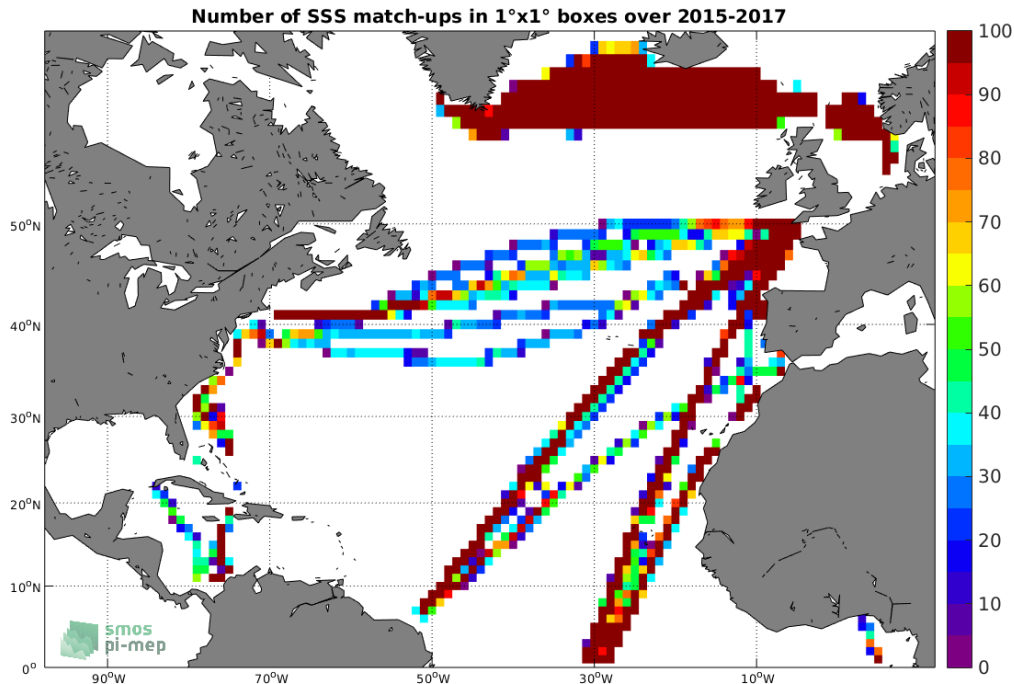
Figure 4: Number of SSS match-ups between TSG-LEGOS-DM SSS and the SMAP-L3-RSS-V3-MONTHLY-70KM SSS product for the North Atlantic Ocean Pi-MEP region over 1^\circ \times 1^\circ boxes and for the full satellite product period.
