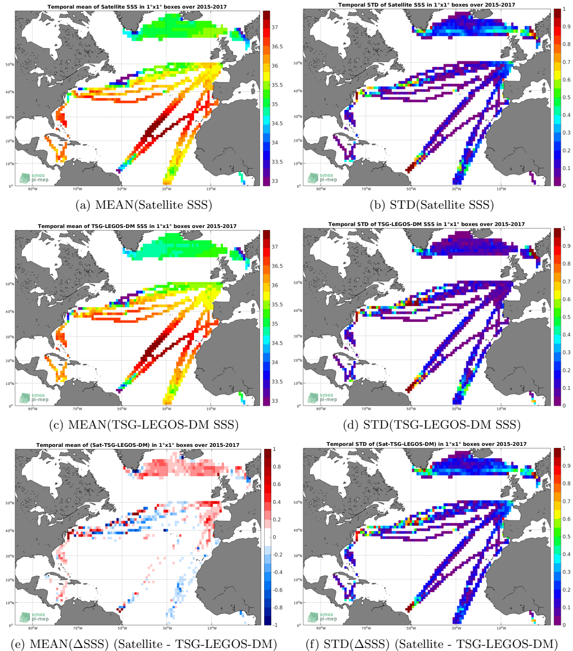
Figure 6: Temporal mean (left) and STD (right) of SSS from SMAP-L3-RSS-V3-MONTHLY-70KM (top), TSG-LEGOS-DM (middle), and of \Delta SSS (Satellite - TSG-LEGOS-DM). Only match-up pairs are used to generate these maps.
