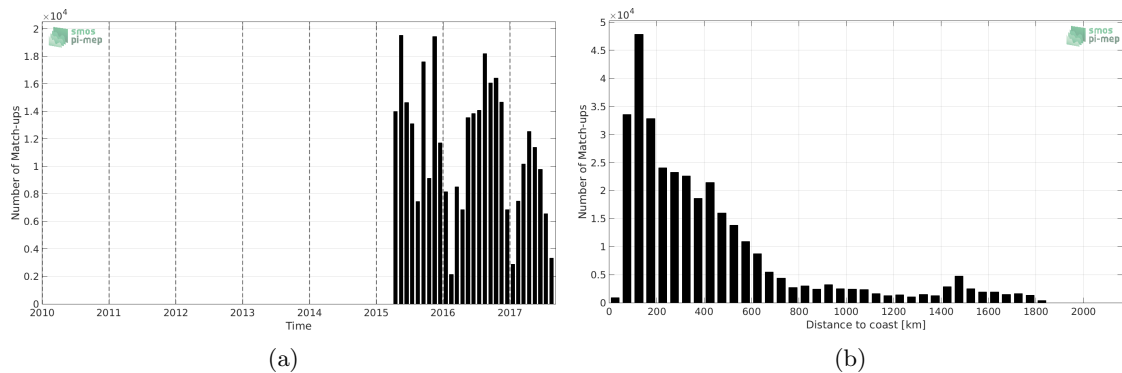
Figure 1: Number of match-ups between TSG-LEGOS-DM and SMAP-L3-RSS-V3-MONTHLY-70KM SSS as a function of time (a) and as function of the distance to coast (b) over the North Atlantic Ocean Pi-MEP region and for the full satellite product period.
