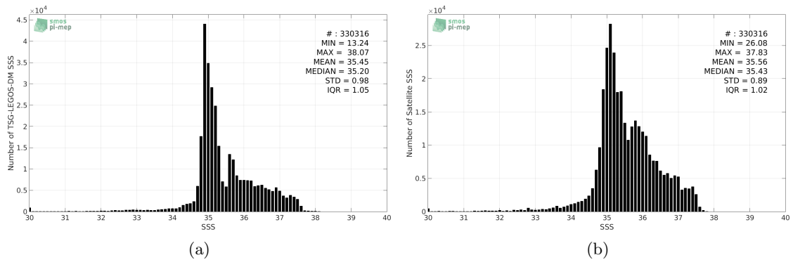
Figure 2: Histograms of SSS from TSG-LEGOS-DM (a) and SMAP-L3-RSS-V3-MONTHLY-70KM (b) considering all match-up pairs per bins of 0.1 over the North Atlantic Ocean Pi-MEP region and for the full satellite product period.
