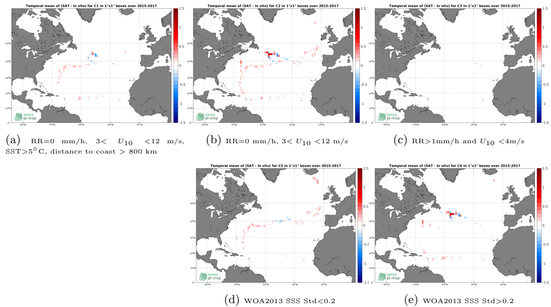
Figure 12: Temporal mean gridded over spatial boxes of size 1^\circ \times 1^\circ of \Delta SSS (SMAP-L3-RSS-V3-MONTHLY-70KM - TSG-GOSUD-Sailing-ship) for 5 different subdatasets corresponding to:RR=0 mm/h, 3 < U_{10} < 12 m/s, SST > 5^\circ\text{C} , distance to coast > 800 km (a), RR=0 mm/h, 3 < U_{10} < 12 m/s (b), RR > 1 mm/h and U_{10} < 4 m/s (c), WOA2013 SSS Std < 0.2 (d), WOA2013 SSS Std > 0.2 (e).
