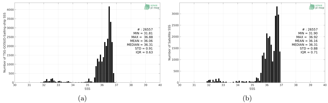
Figure 2: Histograms of SSS from TSG-GOSUD-Sailing-ship (a) and SMAP-L3-RSS-V3-MONTHLY-70KM (b) considering all match-up pairs per bins of 0.1 over the North Atlantic Ocean Pi-MEP region and for the full satellite product period.
