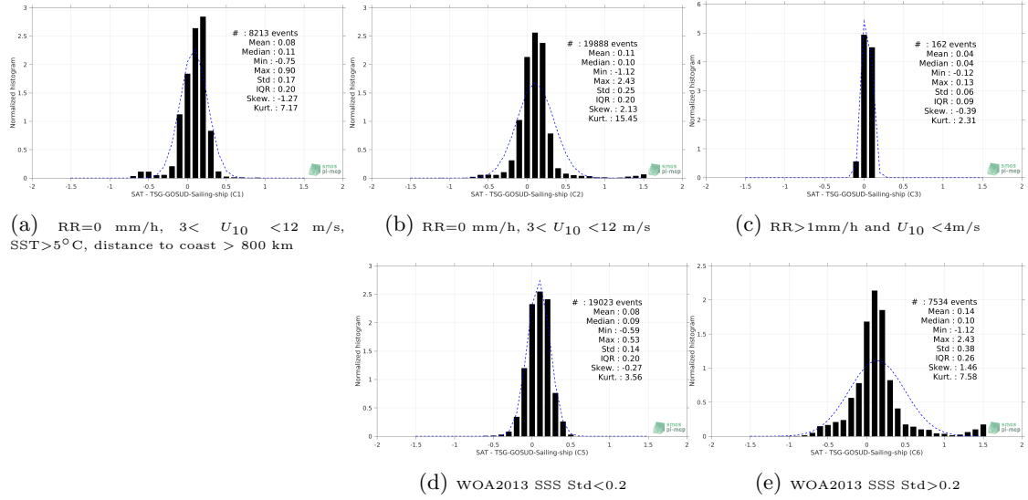
Figure 13: Normalized histogram of \Delta SSS (SMAP-L3-RSS-V3-MONTHLY-70KM - TSG-GOSUD-Sailing-ship) for 5 different subdatasets corresponding to: RR=0 mm/h, 3 < U_{10} < 12 m/s, SST > 5^\circ C , distance to coast > 800 km (a), RR=0 mm/h, 3 < U_{10} < 12 m/s (b), RR > 1 mm/h and U_{10} < 4 m/s (c), WOA2013 SSS Std < 0.2 (d), WOA2013 SSS Std > 0.2 (e).
