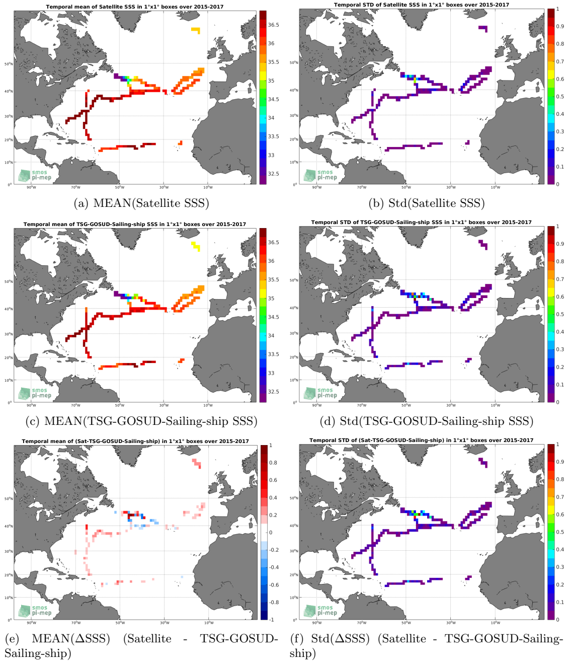
Figure 6: Temporal mean (left) and Std (right) of SSS from SMAP-L3-RSS-V3-MONTHLY-70KM (top), TSG-GOSUD-Sailing-ship (middle), and of \Delta SSS (Satellite - TSG-GOSUD-Sailing-ship). Only match-up pairs are used to generate these maps.
