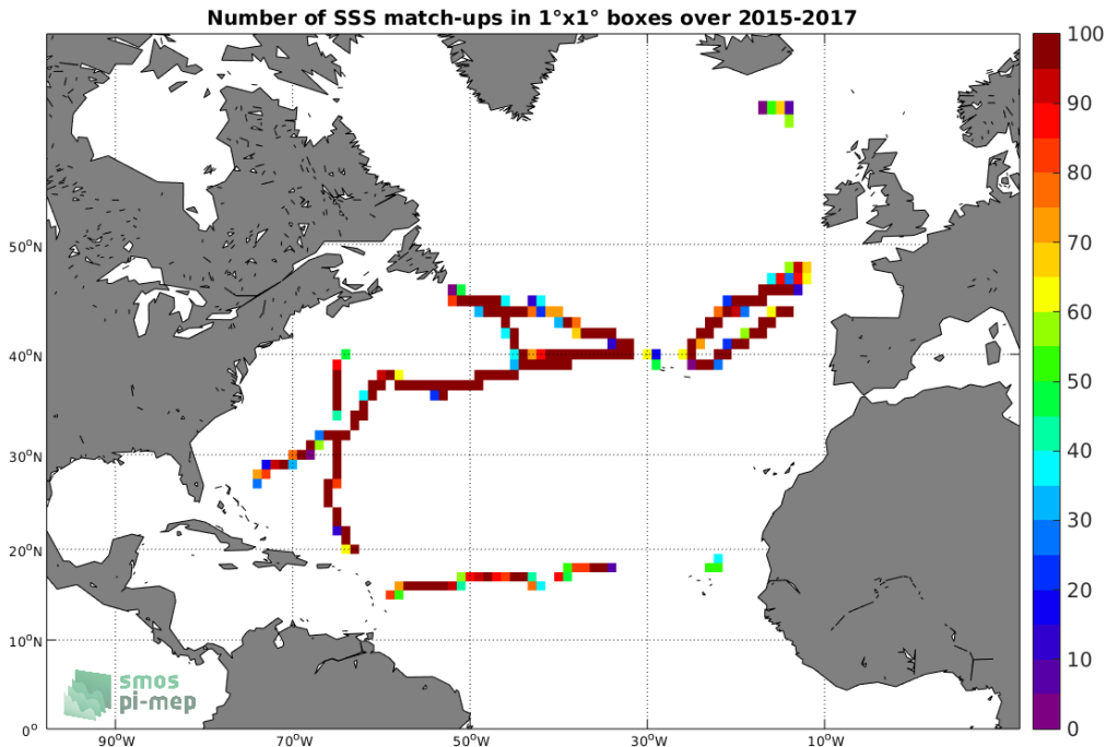
Figure 4: Number of SSS match-ups between TSG-GOSUD-Sailing-ship SSS and the SMAP-L3-RSS-V3-MONTHLY-70KM SSS product for the North Atlantic Ocean Pi-MEP region over 1°x1° boxes and for the full satellite product period.
