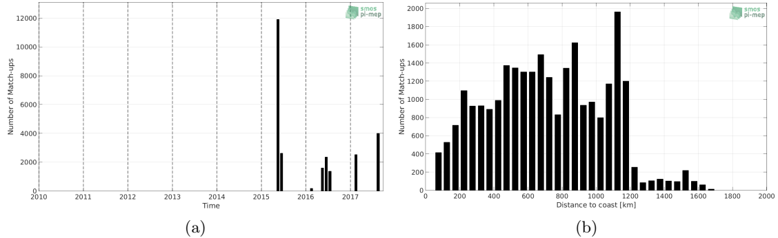
Figure 1: Number of match-ups between TSG-GOSUD-Sailing-ship and SMAP-L3-RSS-V3-MONTHLY-70KM SSS as a function of time (a) and as function of the distance to coast (b) over the North Atlantic Ocean Pi-MEP region and for the full satellite product period.
