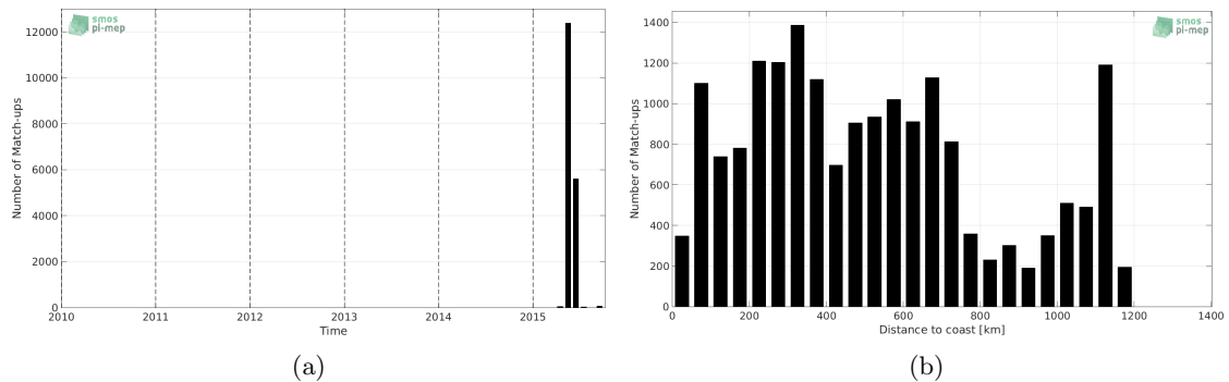
Figure 1: Number of match-ups between TSG-GOSUD-Sailing-ship and SMAP-L3-RSS-V3-MONTHLY-70KM SSS as a function of time (a) and as function of the distance to coast (b) over the North Atlantic Ocean Pi-MEP region and for the full satellite product period.
