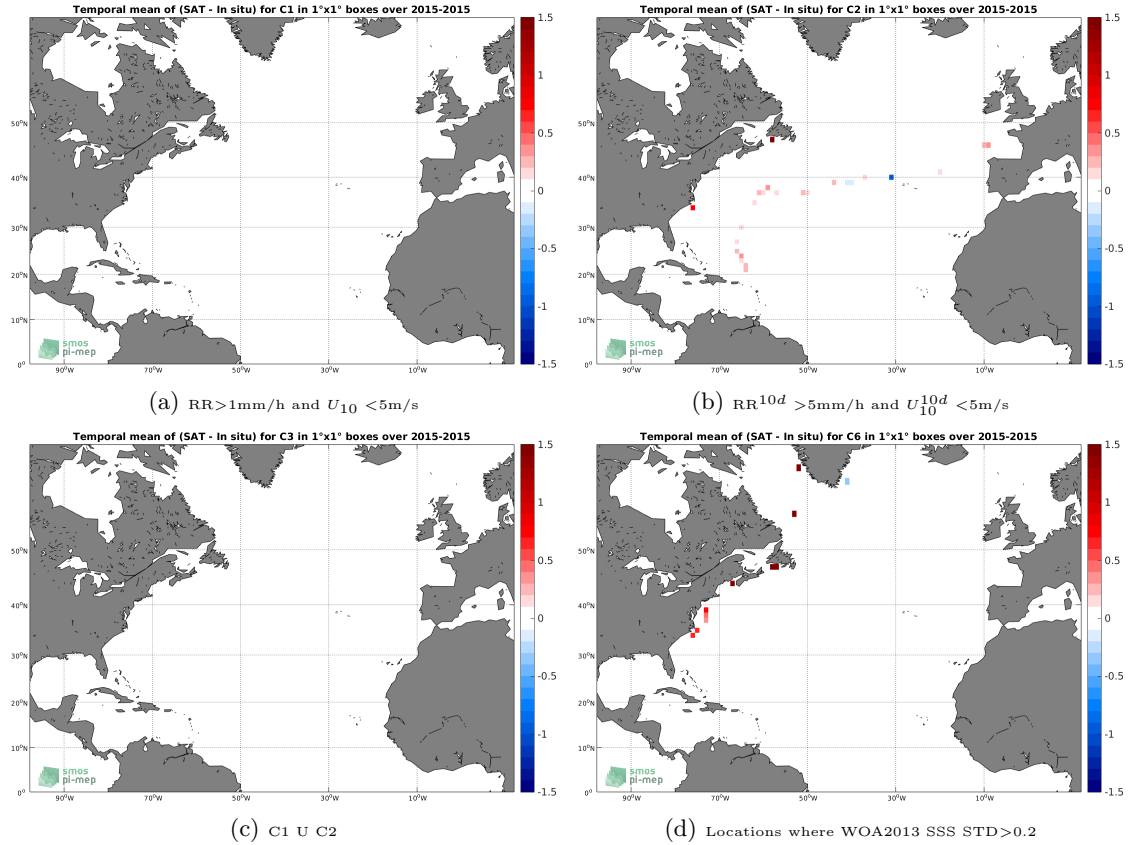
Figure 12: Temporal mean gridded over spatial boxes of size 1^\circ \times 1^\circ of \Delta SSS (SMAP-L3-RSS-V3-MONTHLY-70KM - TSG-GOSUD-Sailing-ship) for 4 different subdatasets corresponding to: RR > 1\text{mm/h} and U_{10} < 5\text{m/s} (a), RR^{10d} > 5\text{mm/h} and U_{10}^{10d} < 5\text{m/s} (b), C1 U C2 (c), Locations where WOA2013 SSS STD > 0.2 (d).
