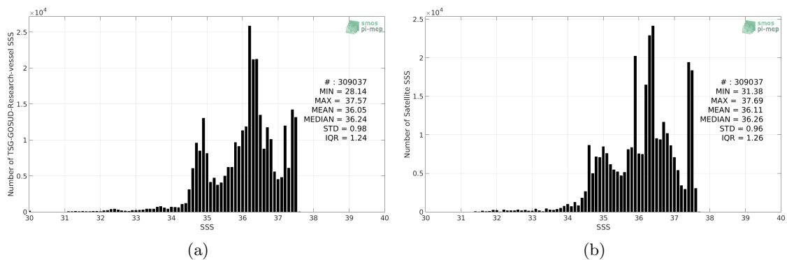
Figure 2: Histograms of SSS from TSG-GOSUD-Research-vessel (a) and SMAP-L3-RSS-V3-MONTHLY-70KM (b) considering all match-up pairs per bins of 0.1 over the North Atlantic Ocean Pi-MEP region and for the full satellite product period.
