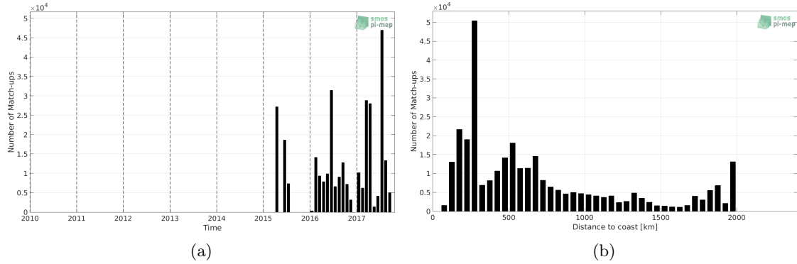
Figure 1: Number of match-ups between TSG-GOSUD-Research-vessel and SMAP-L3-RSS-V3-MONTHLY-70KM SSS as a function of time (a) and as function of the distance to coast (b) over the North Atlantic Ocean Pi-MEP region and for the full satellite product period.
