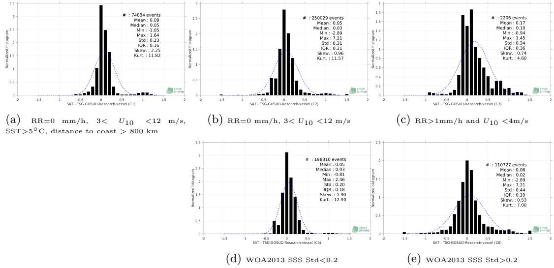
Figure 13: Normalized histogram of \Delta SSS (SMAP-L3-RSS-V3-MONTHLY-70KM - TSG-GOSUD-Research-vessel) for 5 different subdatasets corresponding to: RR=0 mm/h, 3 < U_{10} < 12 m/s, SST > 5°C, distance to coast > 800 km (a), RR=0 mm/h, 3 < U_{10} < 12 m/s (b), RR > 1mm/h and U_{10} < 4 m/s (c), WOA2013 SSS Std < 0.2 (d), WOA2013 SSS Std > 0.2 (e).
