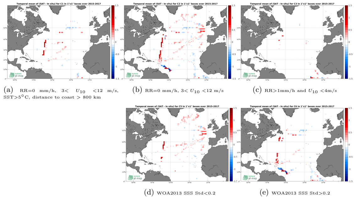
Figure 12: Temporal mean gridded over spatial boxes of size 1^\circ \times 1^\circ of \Delta SSS (SMAP-L3-RSS-V3-MONTHLY-70KM - TSG-GOSUD-Research-vessel) for 5 different subdatasets corresponding to:RR=0 mm/h, 3 < U_{10} < 12 m/s, SST > 5^\circ\text{C} , distance to coast > 800 km (a), RR=0 mm/h, 3 < U_{10} < 12 m/s (b), RR > 1 mm/h and U_{10} < 4 m/s (c), WOA2013 SSS Std < 0.2 (d), WOA2013 SSS Std > 0.2 (e).
