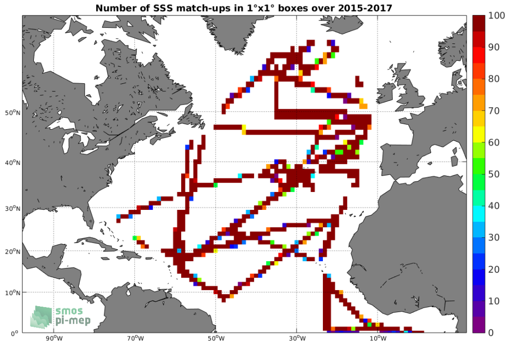
Figure 4: Number of SSS match-ups between TSG-GOSUD-Research-vessel SSS and the SMAP-L3-RSS-V3-MONTHLY-70KM SSS product for the North Atlantic Ocean Pi-MEP region over 1^\circ \times 1^\circ boxes and for the full satellite product period.
