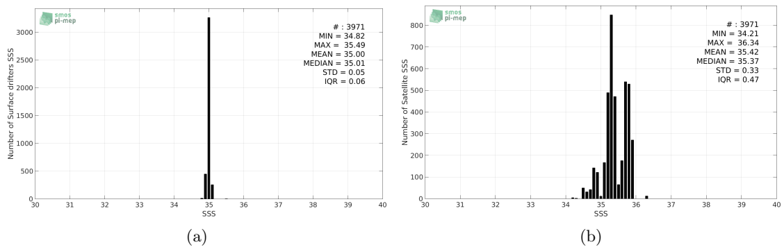
Figure 2: Histograms of SSS from Surface drifters (a) and SMAP-L3-RSS-V3-MONTHLY-70KM (b) considering all match-up pairs per bins of 0.1 over the North Atlantic Ocean Pi-MEP region and for the full satellite product period.
