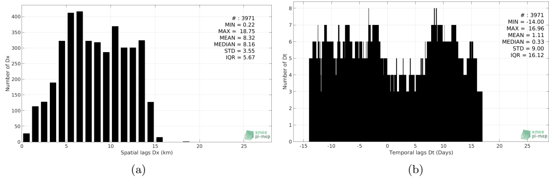
Figure 4: Histograms of the spatial (a) and temporal (b) lags between the time of the Surface drifters measurements and the date of the corresponding SMAP-L3-RSS-V3-MONTHLY-70KM SSS product.
