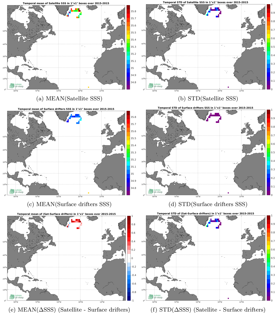
Figure 5: Temporal mean (left) and STD (right) of SSS from SMAP-L3-RSS-V3-MONTHLY-70KM (top), Surface drifters (middle), and of \Delta SSS (Satellite - Surface drifters). Only match-up pairs are used to generate these maps.
