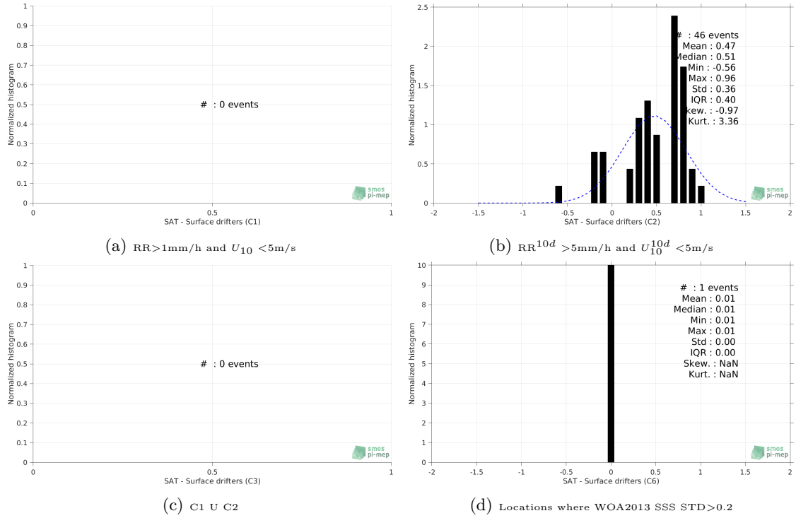
Figure 12: Normalized histogram of \Delta\text{SSS} (SMAP-L3-RSS-V3-MONTHLY-70KM - Surface drifters) for 6 different subdatasets corresponding to: RR > 1\text{mm/h} and U_{10} < 5\text{m/s} (a), RR^{10d} > 5\text{mm/h} and U_{10}^{10d} < 5\text{m/s} (b), C1 \cup C2 (c), Locations where WOA2013 SSS STD > 0.2 (d).
