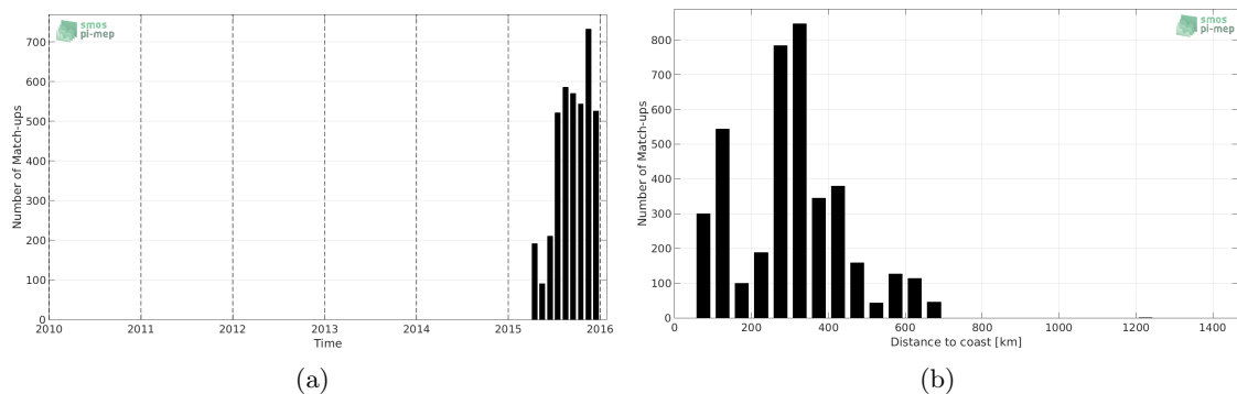
Figure 1: Number of match-ups between Surface drifters and SMAP-L3-RSS-V3-MONTHLY-70KM SSS as a function of time (a) and as function of the distance to coast (b) over the North Atlantic Ocean Pi-MEP region and for the full satellite product period.
