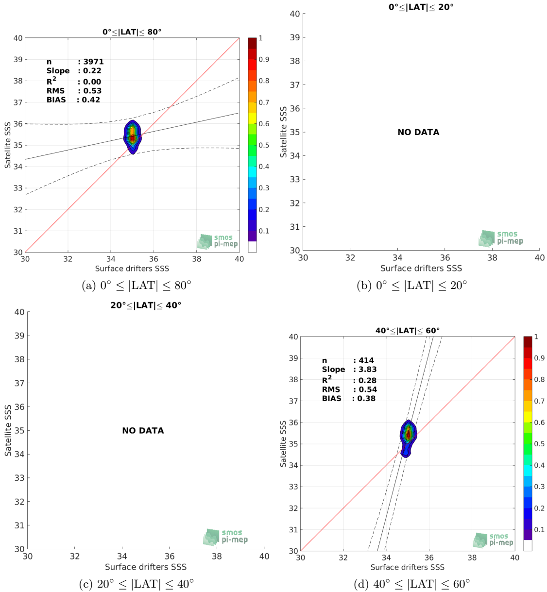
Figure 8: Contour maps of the concentration of SMAP-L3-RSS-V3-MONTHLY-70KM SSS (y-axis) versus Surface drifters SSS (x-axis) at match-up pairs for different latitude bands. For each plot, the red line shows x=y . The black thin and dashed lines indicate a linear fit through the data cloud and the \pm 95\% confidence levels, respectively. The number match-up pairs n , the slope and R^2 coefficient of the linear fit, the root mean square (RMS) and the mean bias between satellite and in situ data are indicated for each latitude band in each plots.
