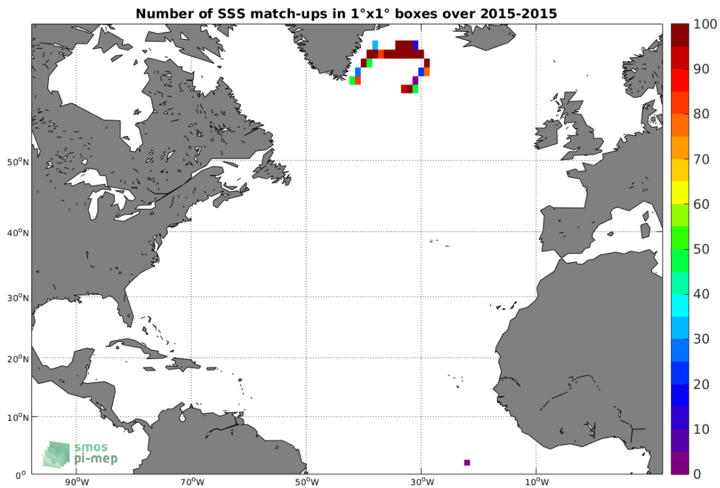
Figure 3: Number of SSS match-ups between Surface drifters SSS and the SMAP-L3-RSS-V3-MONTHLY-70KM SSS product for the North Atlantic Ocean Pi-MEP region over 1°x1° boxes and for the full satellite product period.
