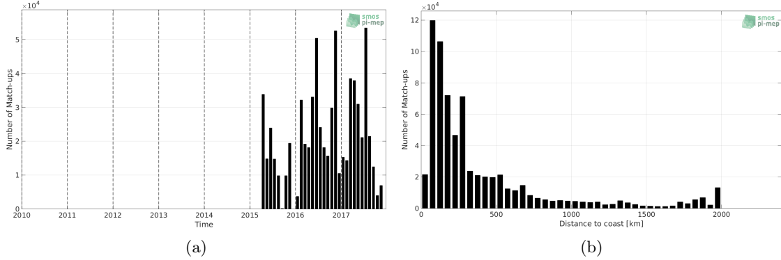
Figure 1: Number of match-ups between TSG-GOSUD-Research-vessel and SMAP-L3-RSS-V3-MONTHLY-0.25DEG-40KM SSS as a function of time (a) and as function of the distance to coast (b) over the North Atlantic Ocean Pi-MEP region and for the full satellite product period.
