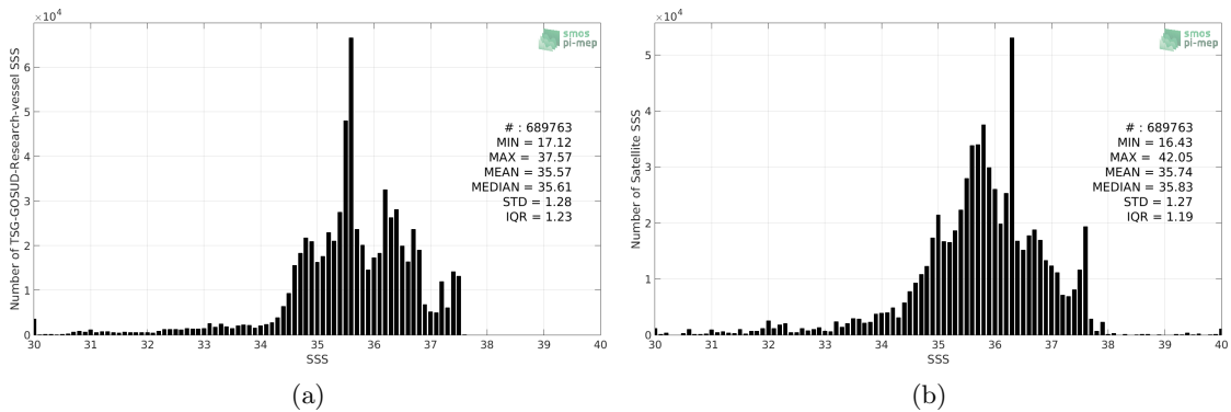
Figure 2: Histograms of SSS from TSG-GOSUD-Research-vessel (a) and SMAP-L3-RSS-V3-MONTHLY-0.25DEG-40KM (b) considering all match-up pairs per bins of 0.1 over the North Atlantic Ocean Pi-MEP region and for the full satellite product period.
