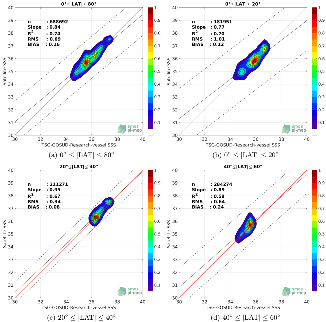
Figure 9: Contour maps of the concentration of SMAP-L3-RSS-V3-MONTHLY-0.25DEG-40KM SSS (y-axis) versus TSG-GOSUD-Research-vessel SSS (x-axis) at match-up pairs for different latitude bands. For each plot, the red line shows x=y . The black thin and dashed lines indicate a linear fit through the data cloud and the \pm 95\% confidence levels, respectively. The number match-up pairs n , the slope and R^2 coefficient of the linear fit, the root mean square (RMS) and the mean bias between satellite and in situ data are indicated for each latitude band in each plots.
