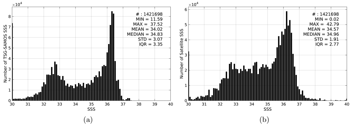
Figure 2: Histograms of SSS from TSG-SAMOS (a) and SMAP-L3-RSS-V2-8DAY-RUNNING-40KM (b) considering all match-up pairs per bins of 0.1 over the North Atlantic Ocean Pi-MEP region and for the full satellite product period.
