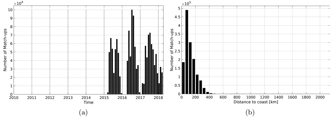
Figure 1: Number of match-ups between TSG-SAMOS and SMAP-L3-RSS-V2-8DAY-RUNNING-40KM SSS as a function of time (a) and as function of the distance to coast (b) over the North Atlantic Ocean Pi-MEP region and for the full satellite product period.
