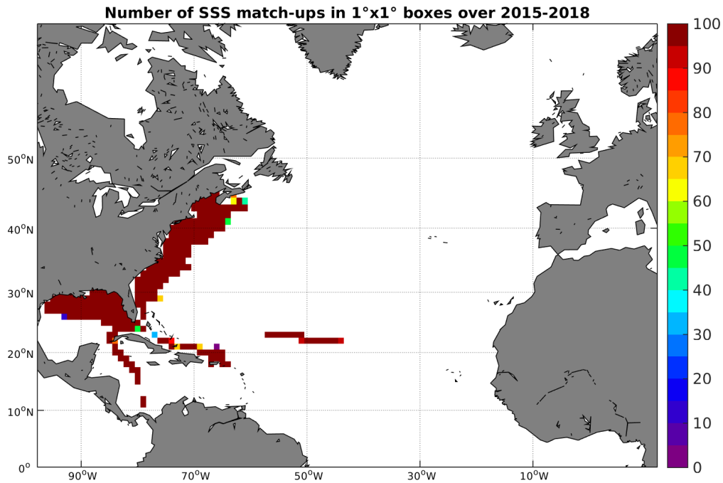
Figure 4: Number of SSS match-ups between TSG-SAMOS SSS and the SMAP-L3-RSS-V2-8DAY-RUNNING-40KM SSS product for the North Atlantic Ocean Pi-MEP region over 1^\circ \times 1^\circ boxes and for the full satellite product period.
