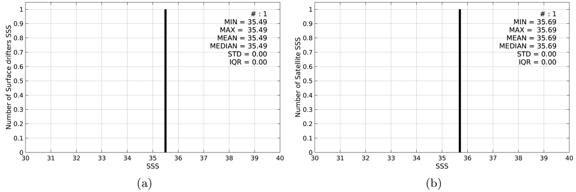
Figure 2: Histograms of SSS from Surface drifters (a) and SMAP-L3-RSS-V2-8DAY-RUNNING-40KM (b) considering all match-up pairs per bins of 0.1 over the North Atlantic Ocean Pi-MEP region and for the full satellite product period.
