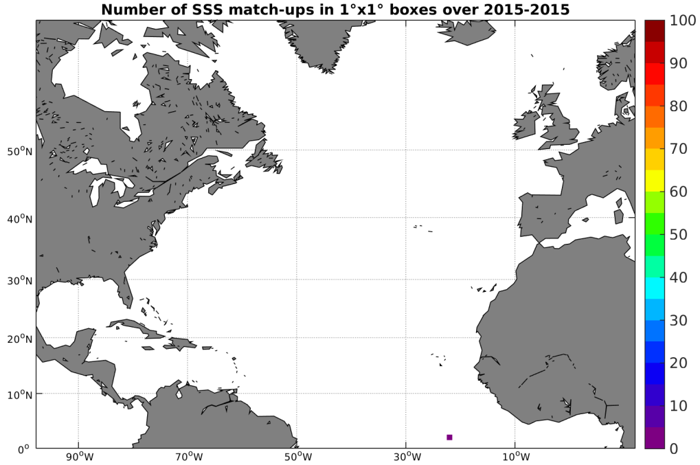
Figure 3: Number of SSS match-ups between Surface drifters SSS and the SMAP-L3-RSS-V2-8DAY-RUNNING-40KM SSS product for the North Atlantic Ocean Pi-MEP region over 1^\circ \times 1^\circ boxes and for the full satellite product period.
