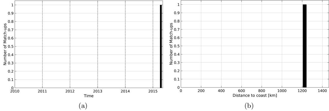
Figure 1: Number of match-ups between Surface drifters and SMAP-L3-RSS-V2-8DAY-RUNNING-40KM SSS as a function of time (a) and as function of the distance to coast (b) over the North Atlantic Ocean Pi-MEP region and for the full satellite product period.
