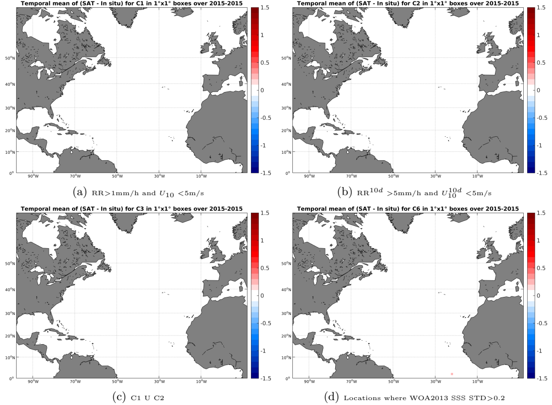
Figure 11: Temporal mean gridded over spatial boxes of size 1^\circ \times 1^\circ of \Delta SSS (SMAP-L3-RSS-V2-8DAY-RUNNING-40KM - Surface drifters) for 4 different subdatasets corresponding to: RR > 1 mm/h and U_{10} < 5 m/s (a), RR^{10d} > 5 mm/h and U_{10}^{10d} < 5 m/s (b), C1 U C2 (c), Locations where WOA2013 SSS STD > 0.2 (d).
