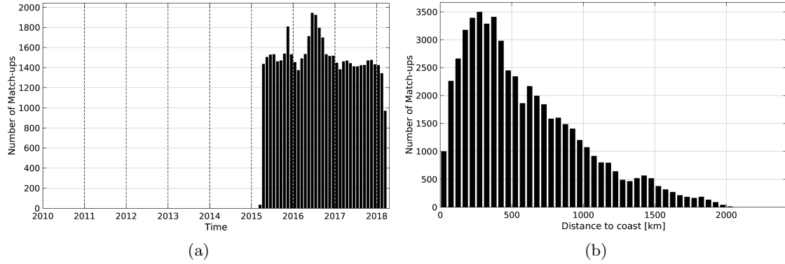
Figure 1: Number of match-ups between Argo and SMAP-L3-RSS-V2-8DAY-RUNNING-40KM SSS as a function of time (a) and as function of the distance to coast (b) over the North Atlantic Ocean Pi-MEP region and for the full satellite product period.
