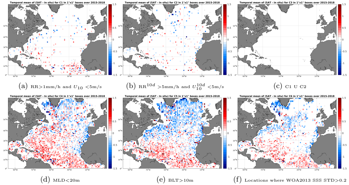
Figure 12: Temporal mean gridded over spatial boxes of size 1^\circ \times 1^\circ of \Delta SSS (SMAP-L3-RSS-V2-8DAY-RUNNING-40KM - Argo) for 6 different subdatasets corresponding to: RR > 1\text{mm/h} and U_{10} < 5\text{m/s} (a), RR^{10d} > 5\text{mm/h} and U_{10}^{10d} < 5\text{m/s} (b), C1 \cup C2 (c), MLD < 20\text{m} (d), BLT > 10\text{m} (e), Locations where WOA2013 SSS STD > 0.2 (f).
