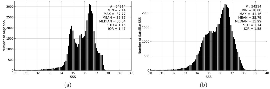
Figure 2: Histograms of SSS from Argo (a) and SMAP-L3-RSS-V2-8DAY-RUNNING-40KM (b) considering all match-up pairs per bins of 0.1 over the North Atlantic Ocean Pi-MEP region and for the full satellite product period.
