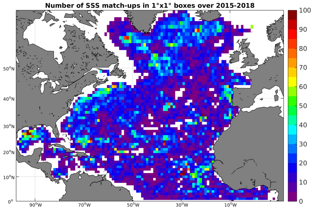
Figure 4: Number of SSS match-ups between Argo SSS and the SMAP-L3-RSS-V2-8DAY-RUNNING-40KM SSS product for the North Atlantic Ocean Pi-MEP region over 1^\circ \times 1^\circ boxes and for the full satellite product period.
