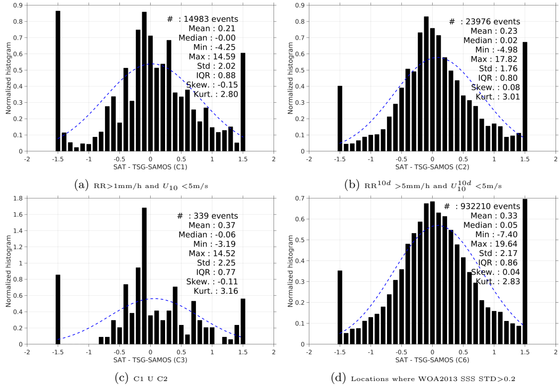
Figure 13: Normalized histogram of \Delta\text{SSS} (SMAP-L3-RSS-V2-8DAY-RUNNING-70KM - TSG-SAMOS) for 6 different subdatasets corresponding to: RR > 1mm/h and U_{10} < 5\text{m/s} (a), RR^{10d} > 5\text{mm/h} and U_{10}^{10d} < 5\text{m/s} (b), C1 U C2 (c), Locations where WOA2013 SSS STD > 0.2 (d).
