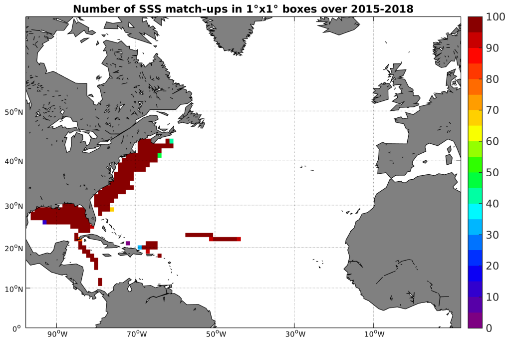
Figure 4: Number of SSS match-ups between TSG-SAMOS SSS and the SMAP-L3-RSS-V2-8DAY-RUNNING-70KM SSS product for the North Atlantic Ocean Pi-MEP region over 1^\circ \times 1^\circ boxes and for the full satellite product period.
