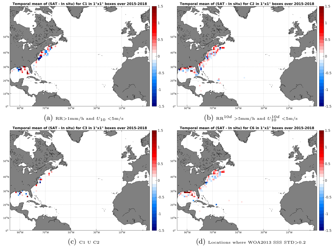
Figure 12: Temporal mean gridded over spatial boxes of size 1^\circ \times 1^\circ of \Delta SSS (SMAP-L3-RSS-V2-8DAY-RUNNING-70KM - TSG-SAMOS) for 4 different subdatasets corresponding to: RR > 1 mm/h and U_{10} < 5 m/s (a), RR 10d > 5 mm/h and U_{10}^{10d} < 5 m/s (b), C1 U C2 (c), Locations where WOA2013 SSS STD > 0.2 (d).
