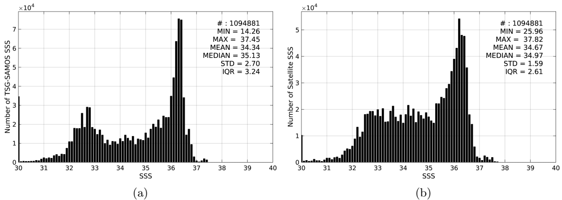
Figure 2: Histograms of SSS from TSG-SAMOS (a) and SMAP-L3-RSS-V2-8DAY-RUNNING-70KM (b) considering all match-up pairs per bins of 0.1 over the North Atlantic Ocean Pi-MEP region and for the full satellite product period.
