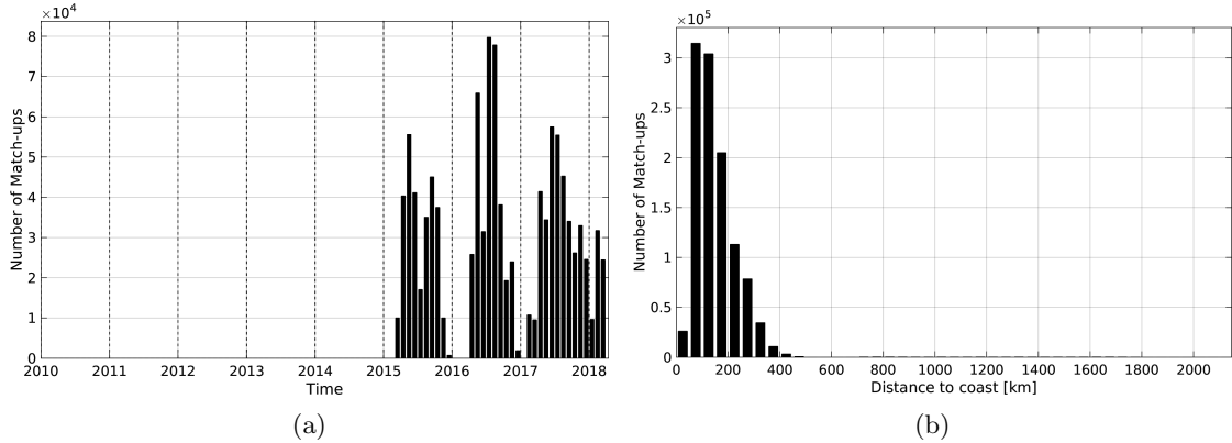
Figure 1: Number of match-ups between TSG-SAMOS and SMAP-L3-RSS-V2-8DAY-RUNNING-70KM SSS as a function of time (a) and as function of the distance to coast (b) over the North Atlantic Ocean Pi-MEP region and for the full satellite product period.
