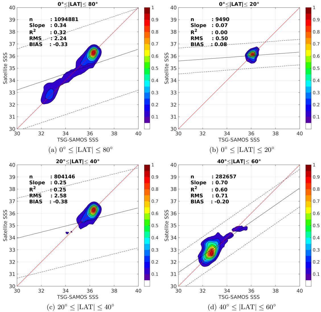
Figure 9: Contour maps of the concentration of SMAP-L3-RSS-V2-8DAY-RUNNING-70KM SSS (y-axis) versus TSG-SAMOS SSS (x-axis) at match-up pairs for different latitude bands. For each plot, the red line shows x=y . The black thin and dashed lines indicate a linear fit through the data cloud and the \pm 95\% confidence levels, respectively. The number match-up pairs n , the slope and R^2 coefficient of the linear fit, the root mean square (RMS) and the mean bias between satellite and in situ data are indicated for each latitude band in each plots.
