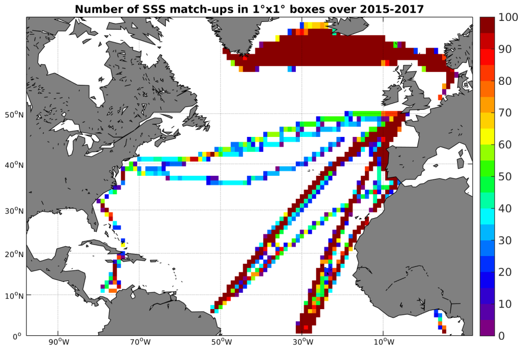
Figure 4: Number of SSS match-ups between TSG-LEGOS-DM SSS and the SMAP-L3-RSS-V2-8DAY-RUNNING-70KM SSS product for the North Atlantic Ocean Pi-MEP region over 1^\circ \times 1^\circ boxes and for the full satellite product period.
