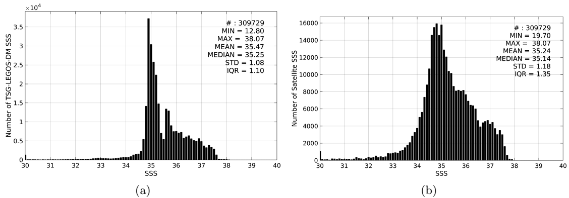
Figure 2: Histograms of SSS from TSG-LEGOS-DM (a) and SMAP-L3-RSS-V2-8DAY-RUNNING-70KM (b) considering all match-up pairs per bins of 0.1 over the North Atlantic Ocean Pi-MEP region and for the full satellite product period.
