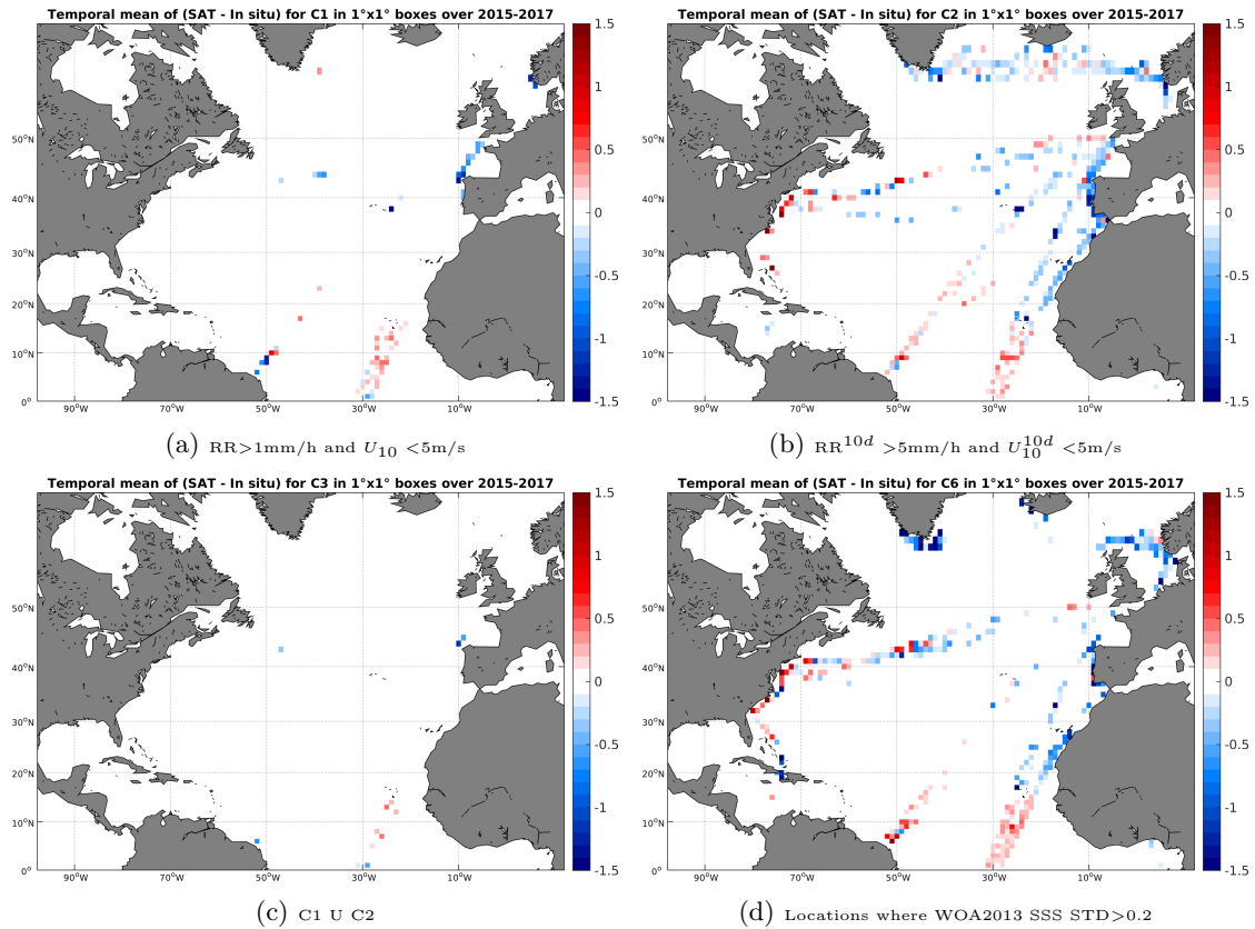
Figure 12: Temporal mean gridded over spatial boxes of size 1^\circ \times 1^\circ of \Delta SSS (SMAP-L3-RSS-V2-8DAY-RUNNING-70KM - TSG-LEGOS-DM) for 4 different subdatasets corresponding to: RR > 1\text{mm/h} and U_{10} < 5\text{m/s} (a), RR^{10d} > 5\text{mm/h} and U_{10}^{10d} < 5\text{m/s} (b), C1 U C2 (c), Locations where WOA2013 SSS STD > 0.2 (d).
