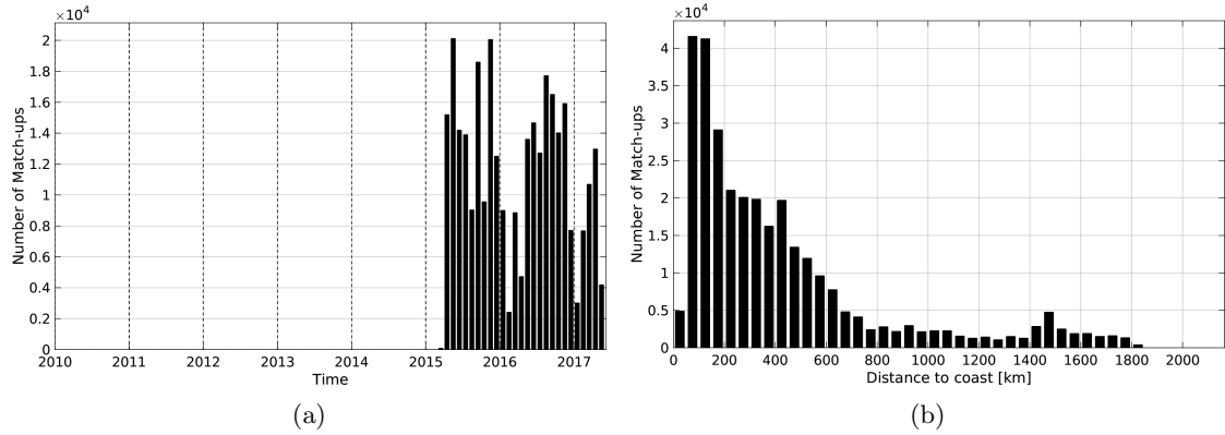
Figure 1: Number of match-ups between TSG-LEGOS-DM and SMAP-L3-RSS-V2-8DAY-RUNNING-70KM SSS as a function of time (a) and as function of the distance to coast (b) over the North Atlantic Ocean Pi-MEP region and for the full satellite product period.
