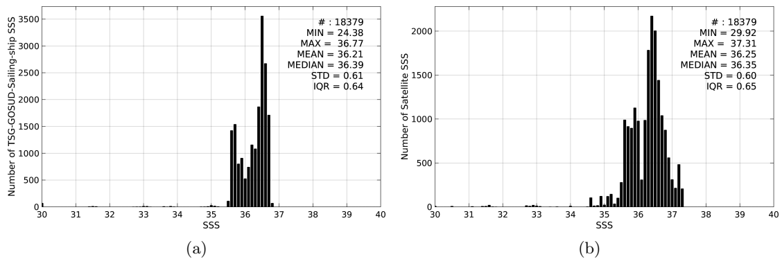
Figure 2: Histograms of SSS from TSG-GOSUD-Sailing-ship (a) and SMAP-L3-RSS-V2-8DAY-RUNNING-70KM (b) considering all match-up pairs per bins of 0.1 over the North Atlantic Ocean Pi-MEP region and for the full satellite product period.
