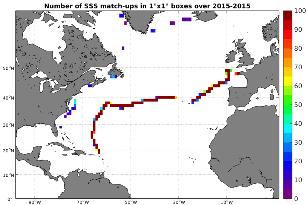
Figure 4: Number of SSS match-ups between TSG-GOSUD-Sailing-ship SSS and the SMAP-L3-RSS-V2-8DAY-RUNNING-70KM SSS product for the North Atlantic Ocean Pi-MEP region over 1^\circ \times 1^\circ boxes and for the full satellite product period.
