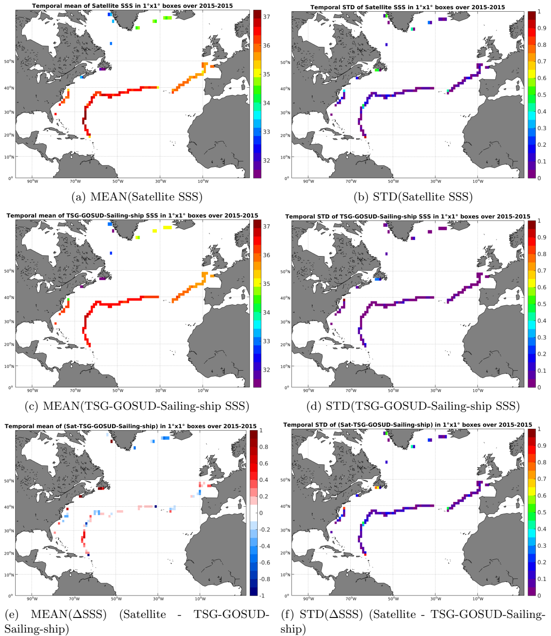
Figure 6: Temporal mean (left) and STD (right) of SSS from SMAP-L3-RSS-V2-8DAY-RUNNING-70KM (top), TSG-GOSUD-Sailing-ship (middle), and of \Delta SSS (Satellite - TSG-GOSUD-Sailing-ship). Only match-up pairs are used to generate these maps.
