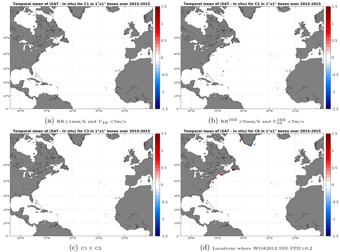
Figure 12: Temporal mean gridded over spatial boxes of size 1^\circ \times 1^\circ of \Delta SSS (SMAP-L3-RSS-V2-8DAY-RUNNING-70KM - TSG-GOSUD-Sailing-ship) for 4 different subdatasets corresponding to: RR > 1\text{mm/h} and U_{10} < 5\text{m/s} (a), RR^{10d} > 5\text{mm/h} and U_{10}^{10d} < 5\text{m/s} (b), C1 U C2 (c), Locations where WOA2013 SSS STD > 0.2 (d).
