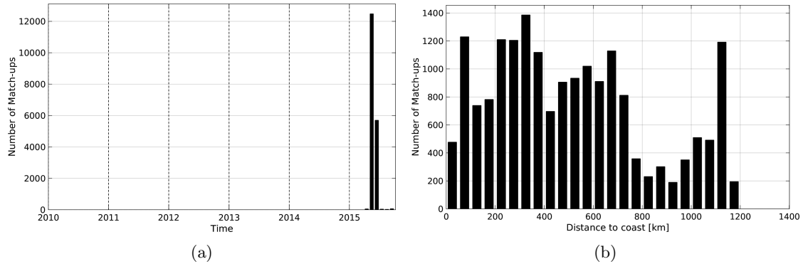
Figure 1: Number of match-ups between TSG-GOSUD-Sailing-ship and SMAP-L3-RSS-V2-8DAY-RUNNING-70KM SSS as a function of time (a) and as function of the distance to coast (b) over the North Atlantic Ocean Pi-MEP region and for the full satellite product period.
