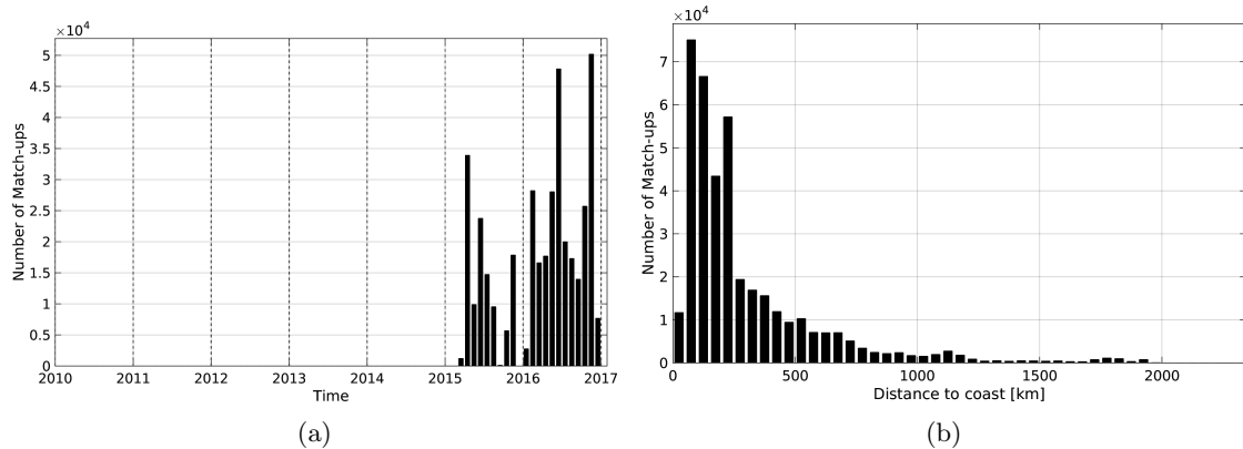
Figure 1: Number of match-ups between TSG-GOSUD-Research-vessel and SMAP-L3-RSS-V2-8DAY-RUNNING-70KM SSS as a function of time (a) and as function of the distance to coast (b) over the North Atlantic Ocean Pi-MEP region and for the full satellite product period.
