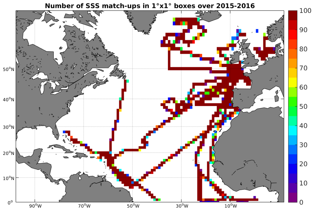
Figure 4: Number of SSS match-ups between TSG-GOSUD-Research-vessel SSS and the SMAP-L3-RSS-V2-8DAY-RUNNING-70KM SSS product for the North Atlantic Ocean Pi-MEP region over 1^\circ \times 1^\circ boxes and for the full satellite product period.
