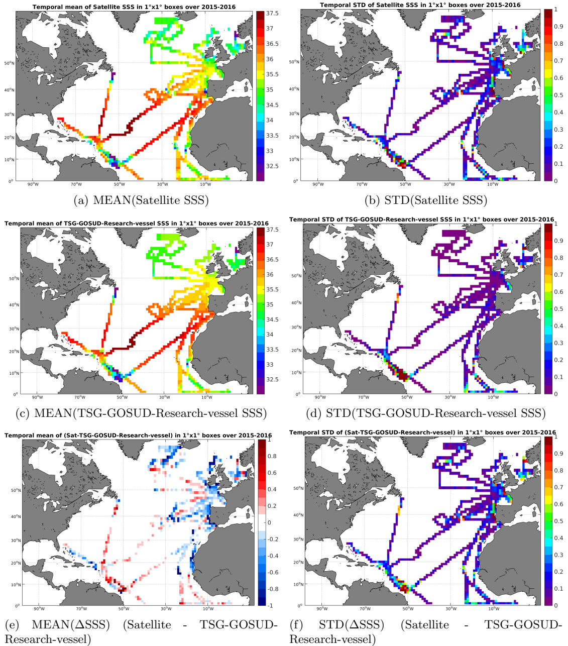
Figure 6: Temporal mean (left) and STD (right) of SSS from SMAP-L3-RSS-V2-8DAY-RUNNING-70KM (top), TSG-GOSUD-Research-vessel (middle), and of \Delta SSS (Satellite - TSG-GOSUD-Research-vessel). Only match-up pairs are used to generate these maps.
