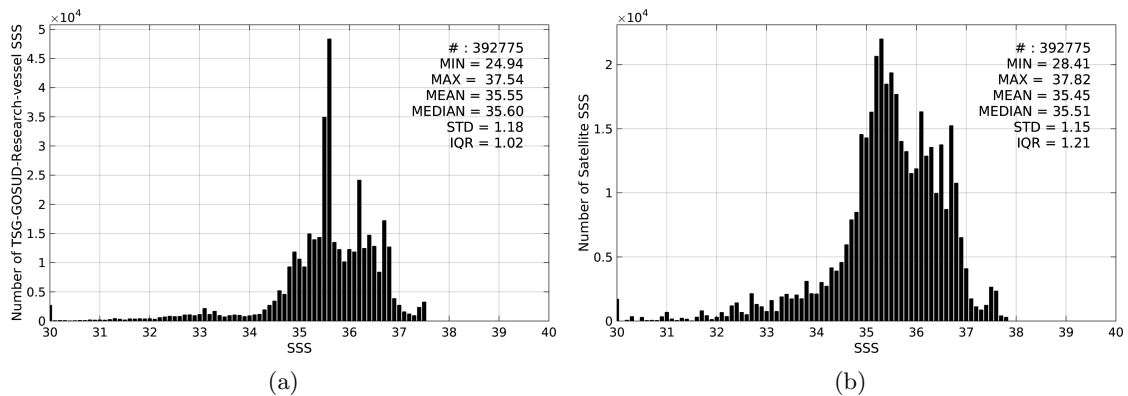
Figure 2: Histograms of SSS from TSG-GOSUD-Research-vessel (a) and SMAP-L3-RSS-V2-8DAY-RUNNING-70KM (b) considering all match-up pairs per bins of 0.1 over the North Atlantic Ocean Pi-MEP region and for the full satellite product period.
