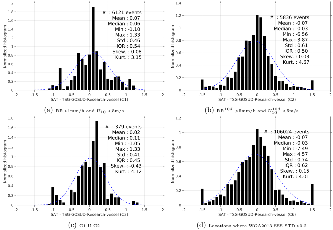
Figure 13: Normalized histogram of \Delta\text{SSS} (SMAP-L3-RSS-V2-8DAY-RUNNING-70KM - TSG-GOSUD-Research-vessel) for 6 different subdatasets corresponding to: \text{RR} > 1\text{mm/h} and U_{10} < 5\text{m/s} (a), \text{RR}^{10d} > 5\text{mm/h} and U_{10}^{10d} < 5\text{m/s} (b), C1 \cup C2 (c), Locations where WOA2013 SSS STD > 0.2 (d).
