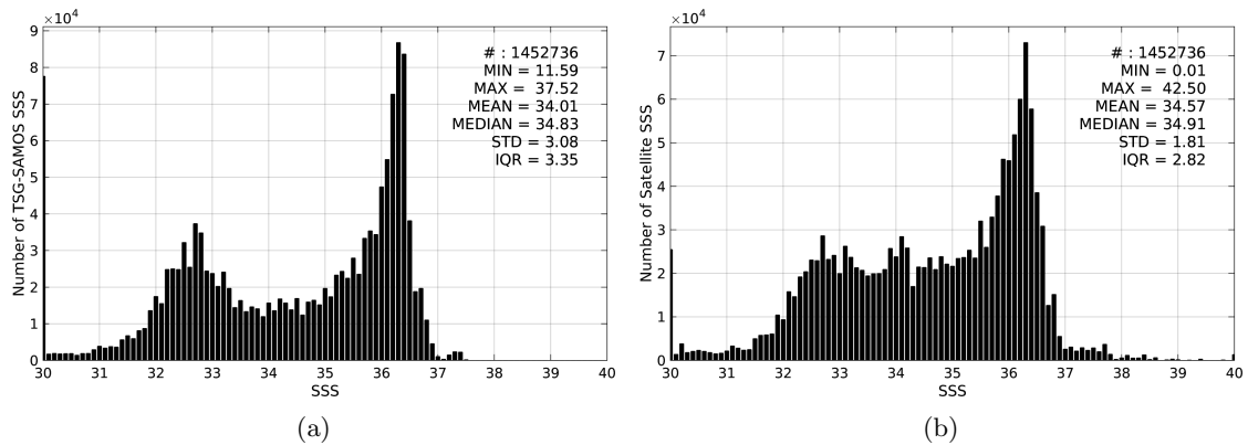
Figure 2: Histograms of SSS from TSG-SAMOS (a) and SMAP-L3-RSS-V2-MONTHLY-0.25DEG-40KM (b) considering all match-up pairs per bins of 0.1 over the North Atlantic Ocean Pi-MEP region and for the full satellite product period.
