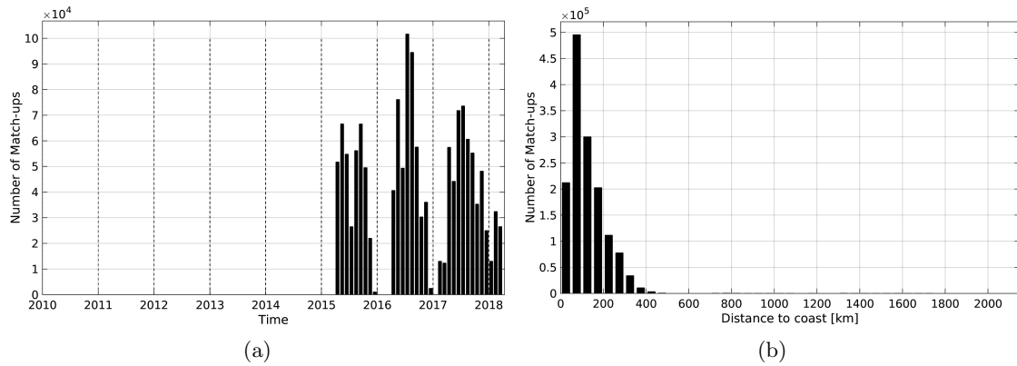
Figure 1: Number of match-ups between TSG-SAMOS and SMAP-L3-RSS-V2-MONTHLY-0.25DEG-40KM SSS as a function of time (a) and as function of the distance to coast (b) over the North Atlantic Ocean Pi-MEP region and for the full satellite product period.
