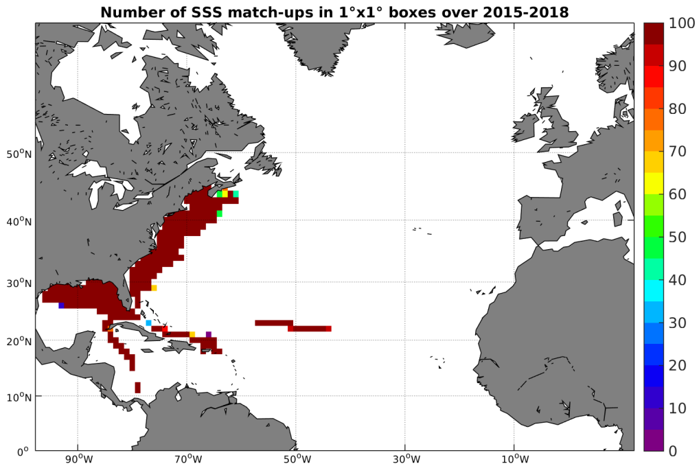
Figure 4: Number of SSS match-ups between TSG-SAMOS SSS and the SMAP-L3-RSS-V2-MONTHLY-0.25DEG-40KM SSS product for the North Atlantic Ocean Pi-MEP region over 1^{\circ} \times 1^{\circ} boxes and for the full satellite product period.
