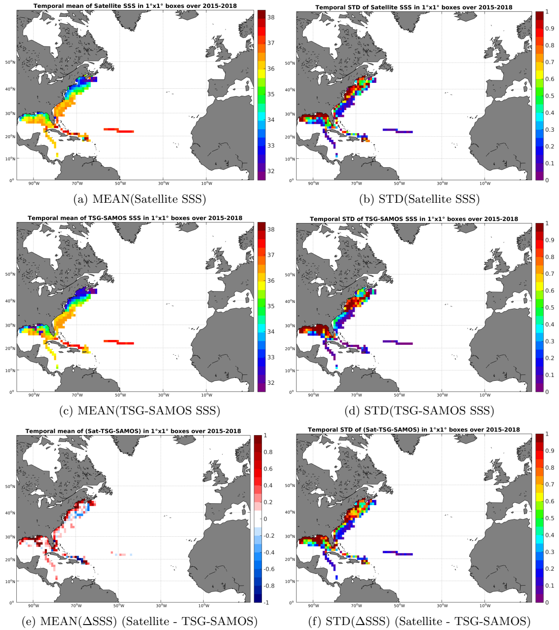
Figure 6: Temporal mean (left) and STD (right) of SSS from SMAP-L3-RSS-V2-MONTHLY-0.25DEG-40KM (top), TSG-SAMOS (middle), and of \Delta SSS (Satellite - TSG-SAMOS). Only match-up pairs are used to generate these maps.
