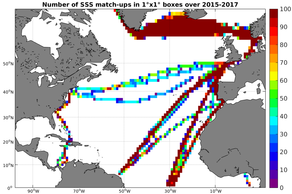
Figure 4: Number of SSS match-ups between TSG-LEGOS-DM SSS and the SMAP-L3-RSS-V2-MONTHLY-0.25DEG-40KM SSS product for the North Atlantic Ocean Pi-MEP region over 1^\circ \times 1^\circ boxes and for the full satellite product period.
