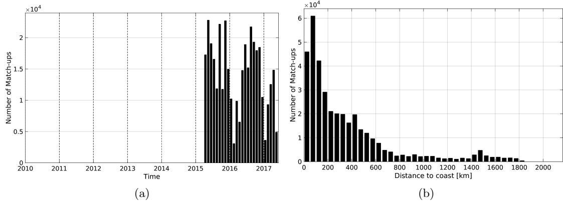
Figure 1: Number of match-ups between TSG-LEGOS-DM and SMAP-L3-RSS-V2-MONTHLY-0.25DEG-40KM SSS as a function of time (a) and as function of the distance to coast (b) over the North Atlantic Ocean Pi-MEP region and for the full satellite product period.
