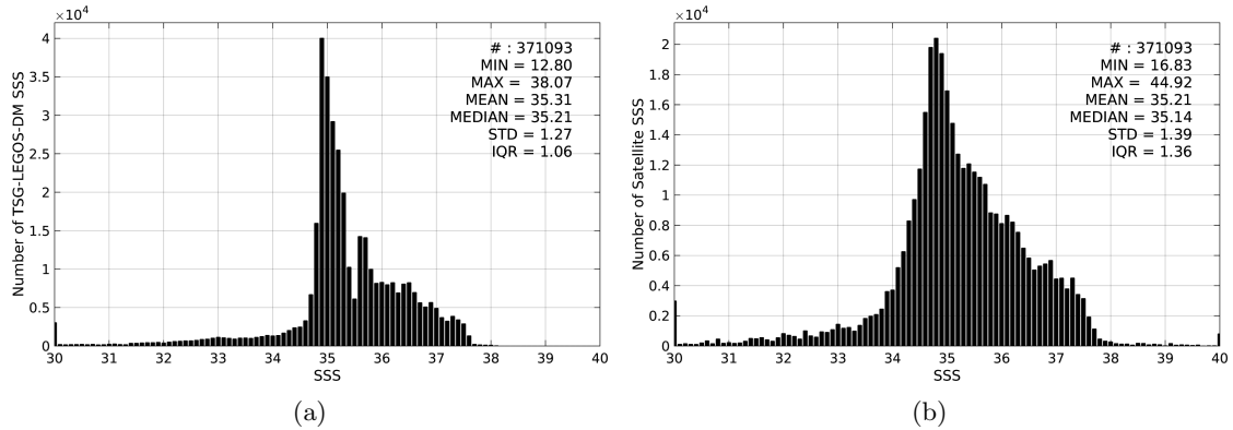
Figure 2: Histograms of SSS from TSG-LEGOS-DM (a) and SMAP-L3-RSS-V2-MONTHLY-0.25DEG-40KM (b) considering all match-up pairs per bins of 0.1 over the North Atlantic Ocean Pi-MEP region and for the full satellite product period.
