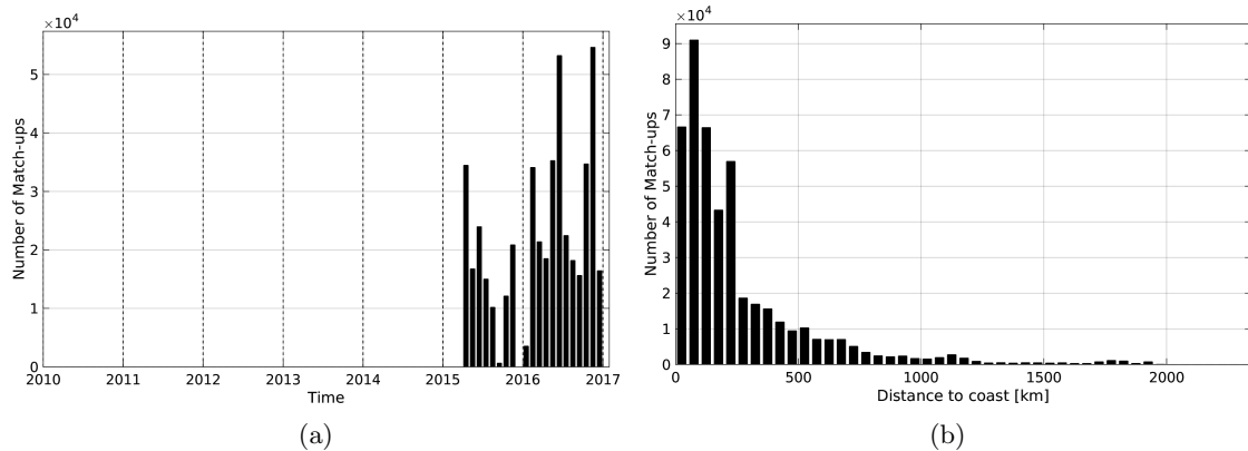
Figure 1: Number of match-ups between TSG-GOSUD-Research-vessel and SMAP-L3-RSS-V2-MONTHLY-0.25DEG-40KM SSS as a function of time (a) and as function of the distance to coast (b) over the North Atlantic Ocean Pi-MEP region and for the full satellite product period.
