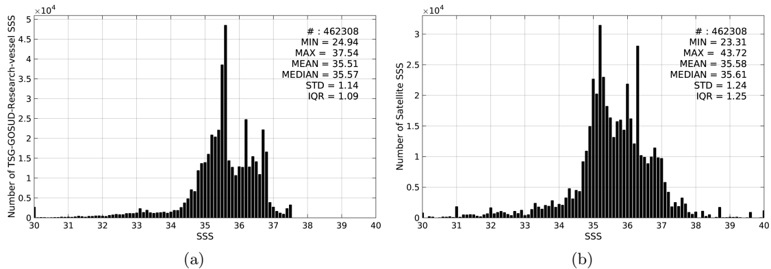
Figure 2: Histograms of SSS from TSG-GOSUD-Research-vessel (a) and SMAP-L3-RSS-V2-MONTHLY-0.25DEG-40KM (b) considering all match-up pairs per bins of 0.1 over the North Atlantic Ocean Pi-MEP region and for the full satellite product period.
