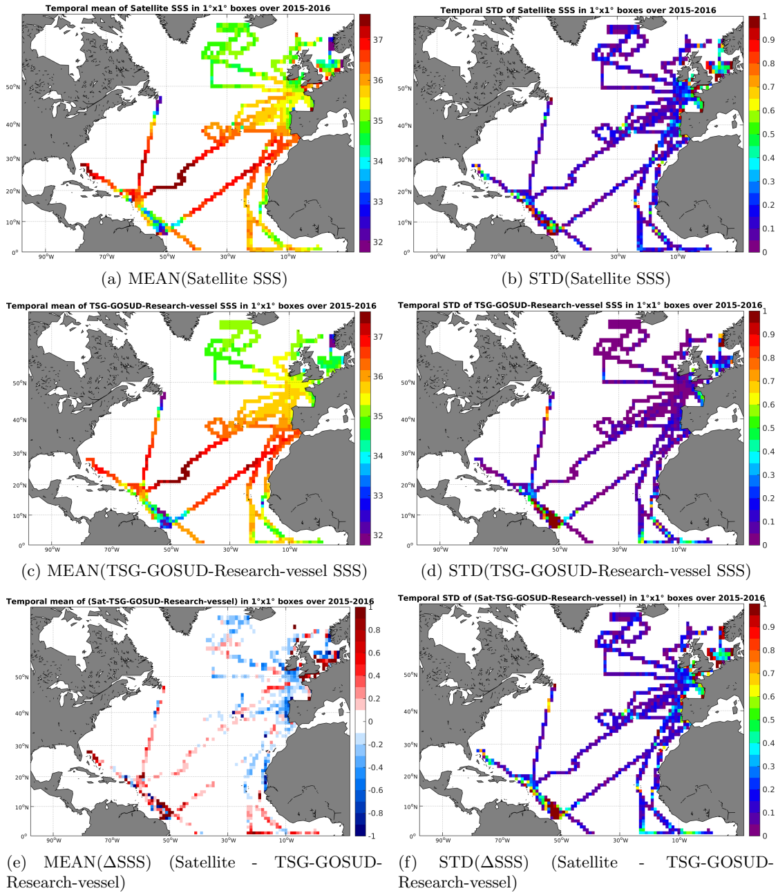
Figure 6: Temporal mean (left) and STD (right) of SSS from SMAP-L3-RSS-V2-MONTHLY-0.25DEG-40KM (top), TSG-GOSUD-Research-vessel (middle), and of \Delta SSS (Satellite - TSG-GOSUD-Research-vessel). Only match-up pairs are used to generate these maps.
