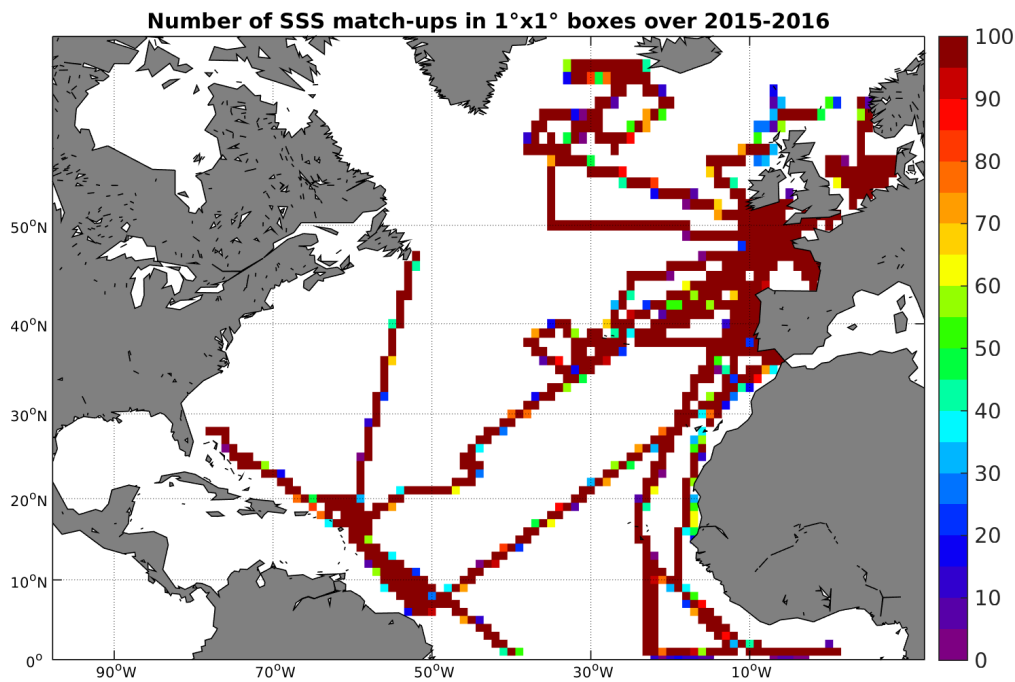
Figure 4: Number of SSS match-ups between TSG-GOSUD-Research-vessel SSS and the SMAP-L3-RSS-V2-MONTHLY-0.25DEG-40KM SSS product for the North Atlantic Ocean Pi-MEP region over 1^\circ \times 1^\circ boxes and for the full satellite product period.
