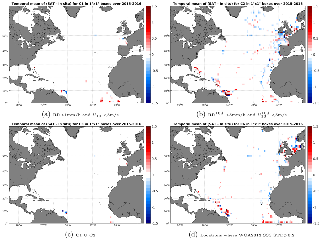
Figure 12: Temporal mean gridded over spatial boxes of size 1^\circ \times 1^\circ of \Delta SSS (SMAP-L3-RSS-V2-MONTHLY-0.25DEG-40KM - TSG-GOSUD-Research-vessel) for 4 different subdatasets corresponding to:RR >1 mm/h and U_{10} < 5 m/s (a), RR^{10d} > 5 mm/h and U_{10}^{10d} < 5 m/s (b), C1 U C2 (c),Locations where WOA2013 SSS STD >0.2 (d).
