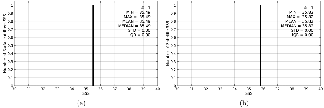
Figure 2: Histograms of SSS from Surface drifters (a) and SMAP-L3-RSS-V2-MONTHLY-0.25DEG-40KM (b) considering all match-up pairs per bins of 0.1 over the North Atlantic Ocean Pi-MEP region and for the full satellite product period.
