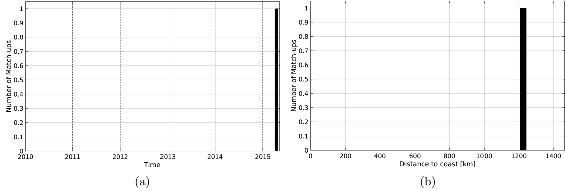
Figure 1: Number of match-ups between Surface drifters and SMAP-L3-RSS-V2-MONTHLY-0.25DEG-40KM SSS as a function of time (a) and as function of the distance to coast (b) over the North Atlantic Ocean Pi-MEP region and for the full satellite product period.
