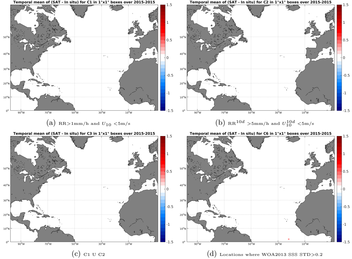
Figure 11: Temporal mean gridded over spatial boxes of size 1^\circ \times 1^\circ of \Delta SSS (SMAP-L3-RSS-V2-MONTHLY-0.25DEG-40KM - Surface drifters) for 4 different subdatasets corresponding to: RR > 1mm/h and U_{10} < 5 m/s (a), RR^{10d} > 5 mm/h and U_{10}^{10d} < 5 m/s (b), C1 U C2 (c), Locations where WOA2013 SSS STD > 0.2 (d).
