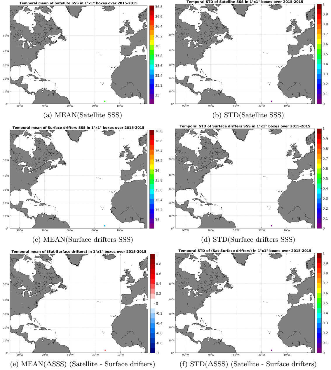
Figure 5: Temporal mean (left) and STD (right) of SSS from SMAP-L3-RSS-V2-MONTHLY-0.25DEG-40KM (top), Surface drifters (middle), and of \Delta SSS (Satellite - Surface drifters). Only match-up pairs are used to generate these maps.
