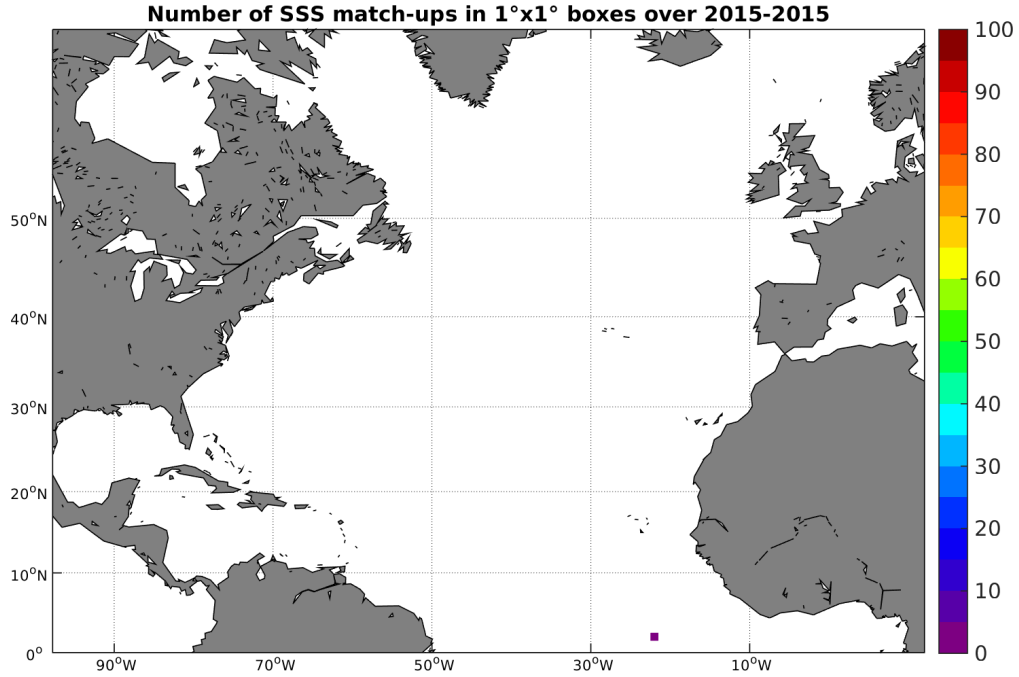
Figure 3: Number of SSS match-ups between Surface drifters SSS and the SMAP-L3-RSS-V2-MONTHLY-0.25DEG-40KM SSS product for the North Atlantic Ocean Pi-MEP region over 1^\circ \times 1^\circ boxes and for the full satellite product period.
