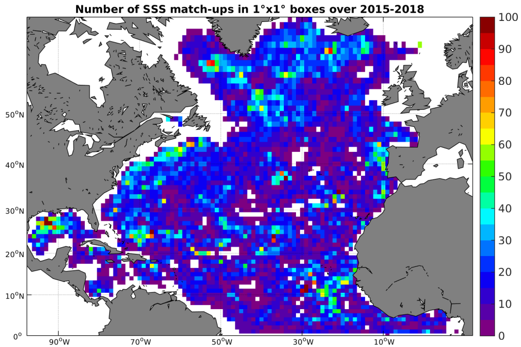
Figure 4: Number of SSS match-ups between Argo SSS and the SMAP-L3-RSS-V2-MONTHLY-0.25DEG-40KM SSS product for the North Atlantic Ocean Pi-MEP region over 1^\circ \times 1^\circ boxes and for the full satellite product period.
