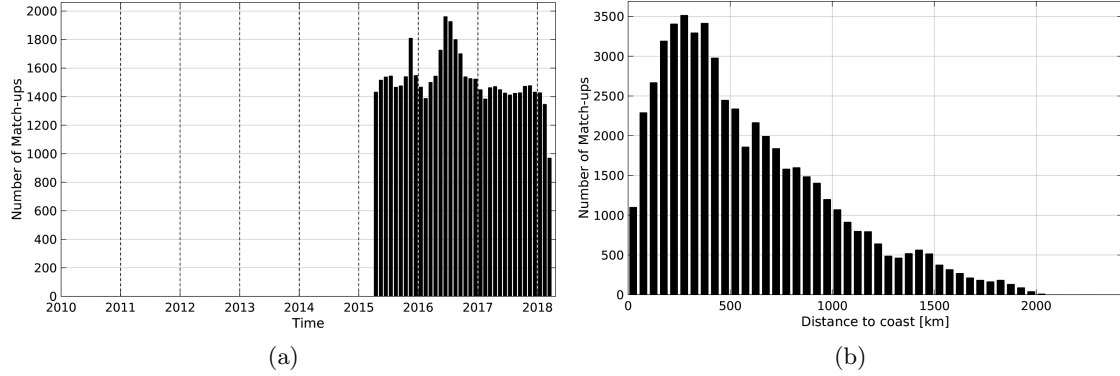
Figure 1: Number of match-ups between Argo and SMAP-L3-RSS-V2-MONTHLY-0.25DEG-40KM SSS as a function of time (a) and as function of the distance to coast (b) over the North Atlantic Ocean Pi-MEP region and for the full satellite product period.
