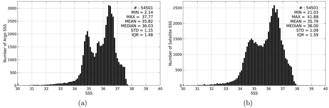
Figure 2: Histograms of SSS from Argo (a) and SMAP-L3-RSS-V2-MONTHLY-0.25DEG-40KM (b) considering all match-up pairs per bins of 0.1 over the North Atlantic Ocean Pi-MEP region and for the full satellite product period.
