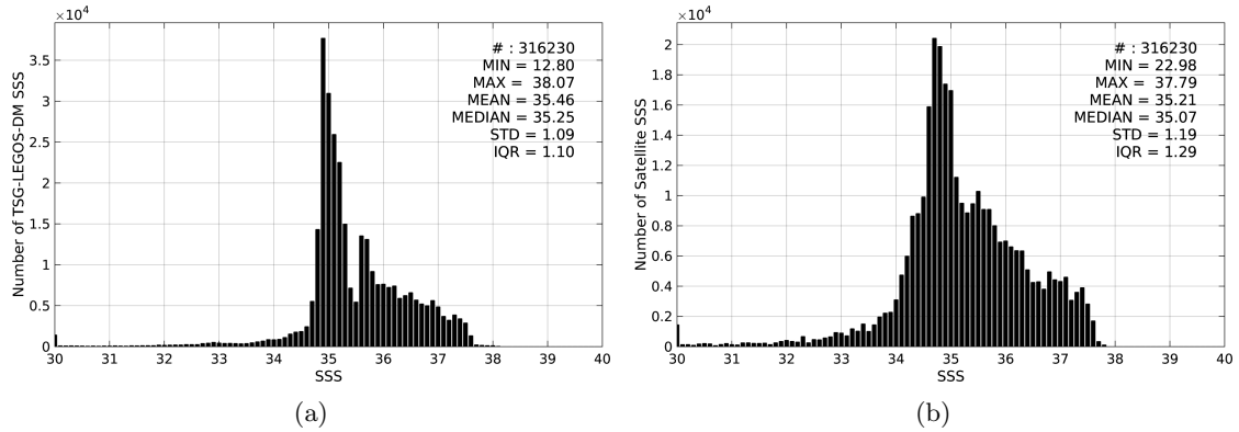
Figure 2: Histograms of SSS from TSG-LEGOS-DM (a) and SMAP-L3-RSS-V2-MONTHLY-70KM (b) considering all match-up pairs per bins of 0.1 over the North Atlantic Ocean Pi-MEP region and for the full satellite product period.
