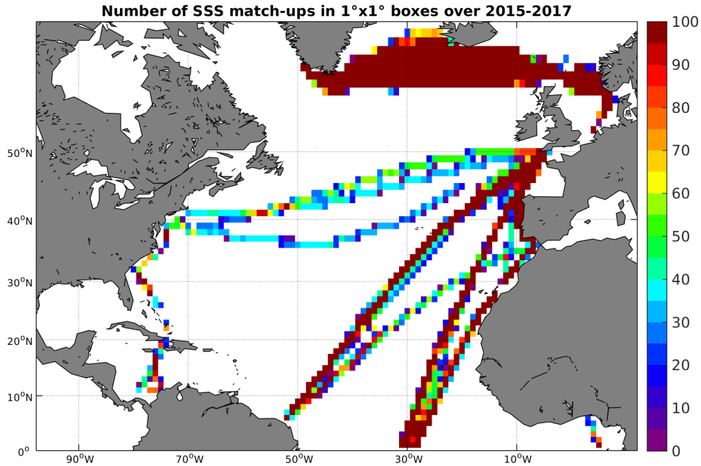
Figure 4: Number of SSS match-ups between TSG-LEGOS-DM SSS and the SMAP-L3-RSS-V2-MONTHLY-70KM SSS product for the North Atlantic Ocean Pi-MEP region over 1°x1° boxes and for the full satellite product period.
