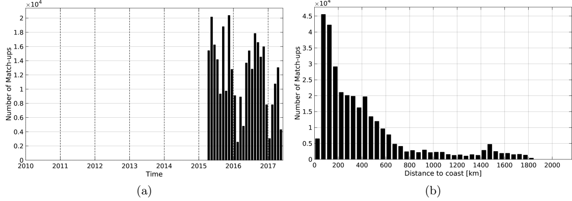
Figure 1: Number of match-ups between TSG-LEGOS-DM and SMAP-L3-RSS-V2-MONTHLY-70KM SSS as a function of time (a) and as function of the distance to coast (b) over the North Atlantic Ocean Pi-MEP region and for the full satellite product period.
