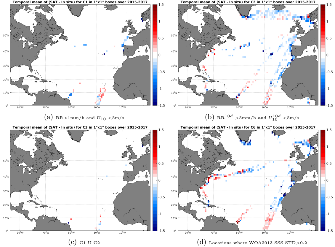
Figure 12: Temporal mean gridded over spatial boxes of size 1^\circ \times 1^\circ of \Delta SSS (SMAP-L3-RSS-V2-MONTHLY-70KM - TSG-LEGOS-DM) for 4 different subdatasets corresponding to: RR > 1mm/h and U_{10} < 5 m/s (a), RR^{10d} > 5 mm/h and U_{10}^{10d} < 5 m/s (b), C1 U C2 (c), Locations where WOA2013 SSS STD > 0.2 (d).
