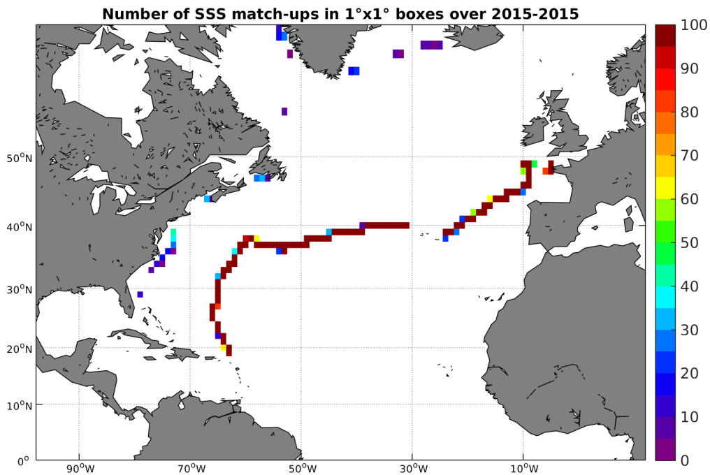
Figure 4: Number of SSS match-ups between TSG-GOSUD-Sailing-ship SSS and the SMAP-L3-RSS-V2-MONTHLY-70KM SSS product for the North Atlantic Ocean Pi-MEP region over 1^\circ \times 1^\circ boxes and for the full satellite product period.
