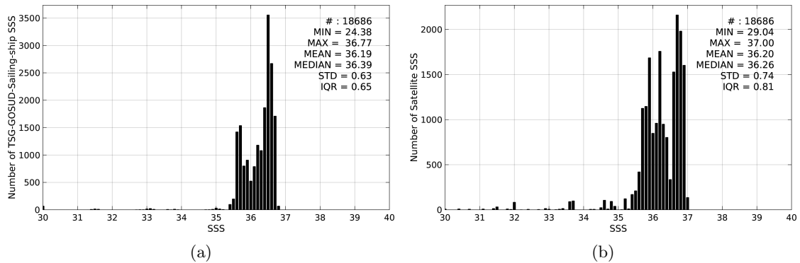
Figure 2: Histograms of SSS from TSG-GOSUD-Sailing-ship (a) and SMAP-L3-RSS-V2-MONTHLY-70KM (b) considering all match-up pairs per bins of 0.1 over the North Atlantic Ocean Pi-MEP region and for the full satellite product period.
