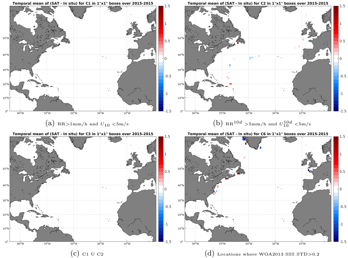
Figure 12: Temporal mean gridded over spatial boxes of size 1°x1° of \Delta SSS (SMAP-L3-RSS-V2-MONTHLY-70KM - TSG-GOSUD-Sailing-ship) for 4 different subdatasets corresponding to: RR > 1\text{mm/h} and U_{10} < 5\text{m/s} (a), RR^{10d} > 5\text{mm/h} and U_{10}^{10d} < 5\text{m/s} (b), C1 U C2 (c), Locations where WOA2013 SSS STD > 0.2 (d).
