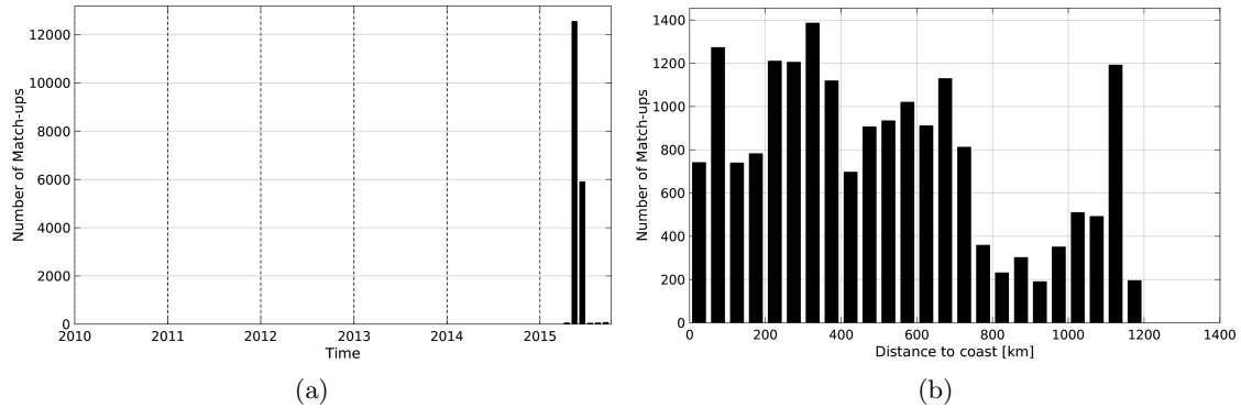
Figure 1: Number of match-ups between TSG-GOSUD-Sailing-ship and SMAP-L3-RSS-V2-MONTHLY-70KM SSS as a function of time (a) and as function of the distance to coast (b) over the North Atlantic Ocean Pi-MEP region and for the full satellite product period.
