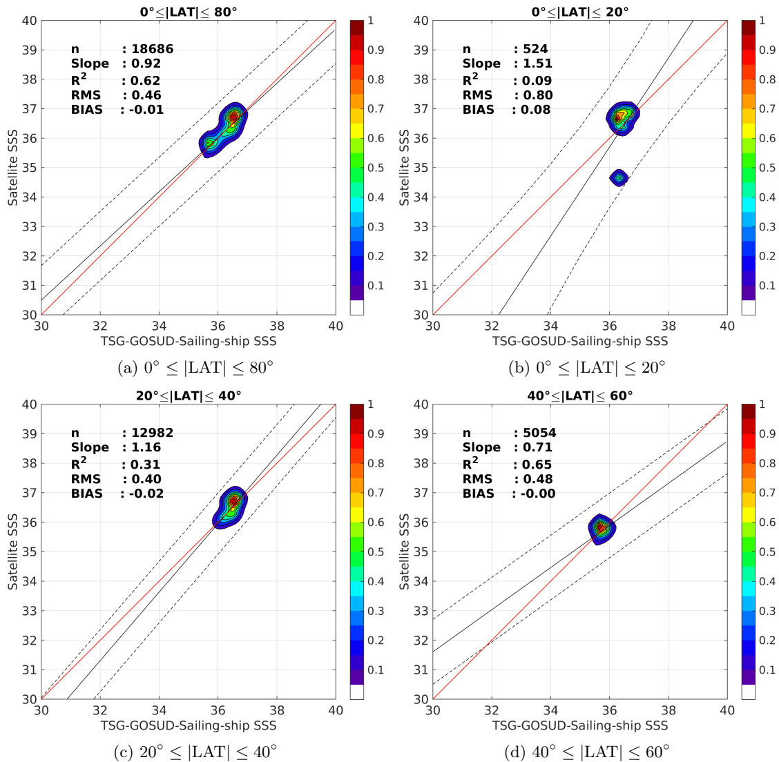
Figure 9: Contour maps of the concentration of SMAP-L3-RSS-V2-MONTHLY-70KM SSS (y-axis) versus TSG-GOSUD-Sailing-ship SSS (x-axis) at match-up pairs for different latitude bands. For each plot, the red line shows x=y . The black thin and dashed lines indicate a linear fit through the data cloud and the \pm 95\% confidence levels, respectively. The number match-up pairs n , the slope and R^2 coefficient of the linear fit, the root mean square (RMS) and the mean bias between satellite and in situ data are indicated for each latitude band in each plots.
