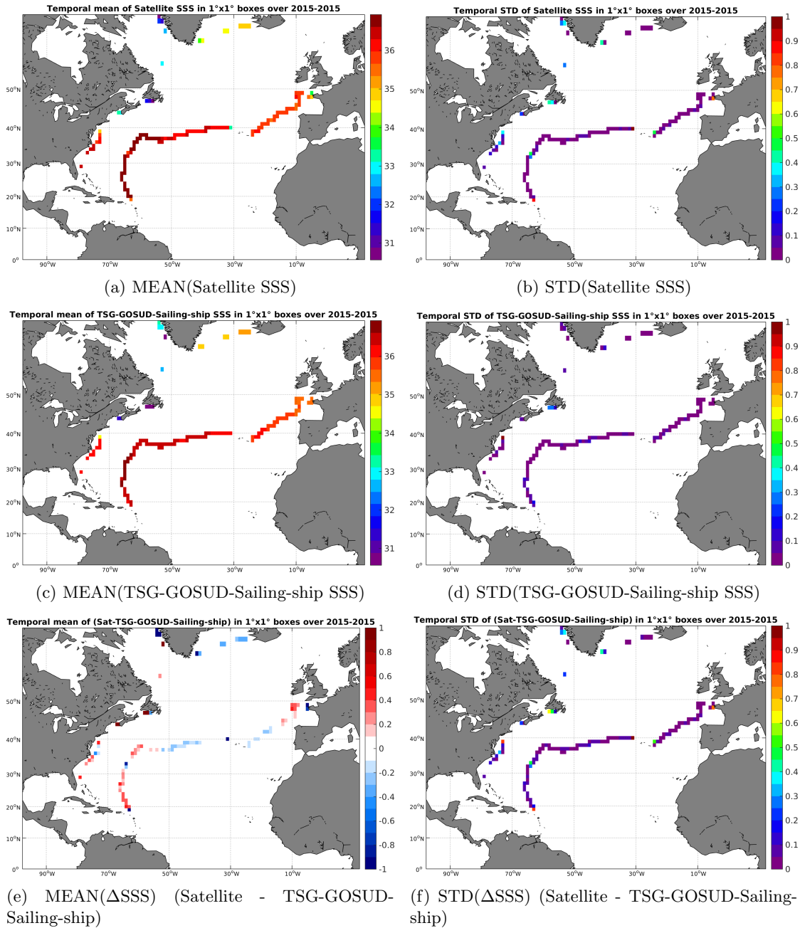
Figure 6: Temporal mean (left) and STD (right) of SSS from SMAP-L3-RSS-V2-MONTHLY-70KM (top), TSG-GOSUD-Sailing-ship (middle), and of \Delta SSS (Satellite - TSG-GOSUD-Sailing-ship). Only match-up pairs are used to generate these maps.
