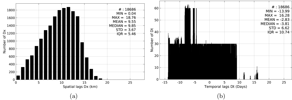
Figure 5: Histograms of the spatial (a) and temporal (b) lags between the time of the TSG-GOSUD-Sailing-ship measurements and the date of the corresponding SMAP-L3-RSS-V2-MONTHLY-70KM SSS product.
