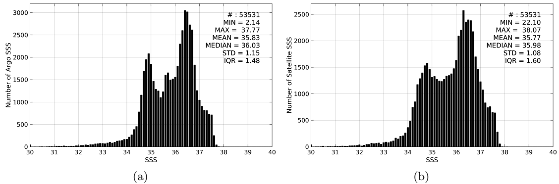
Figure 2: Histograms of SSS from Argo (a) and SMAP-L3-RSS-V2-MONTHLY-70KM (b) considering all match-up pairs per bins of 0.1 over the North Atlantic Ocean Pi-MEP region and for the full satellite product period.
