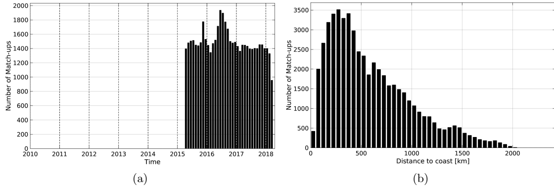
Figure 1: Number of match-ups between Argo and SMAP-L3-RSS-V2-MONTHLY-70KM SSS as a function of time (a) and as function of the distance to coast (b) over the North Atlantic Ocean Pi-MEP region and for the full satellite product period.
