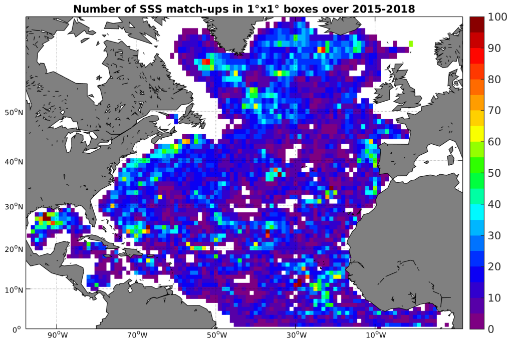
Figure 4: Number of SSS match-ups between Argo SSS and the SMAP-L3-RSS-V2-MONTHLY-70KM SSS product for the North Atlantic Ocean Pi-MEP region over 1^\circ \times 1^\circ boxes and for the full satellite product period.
