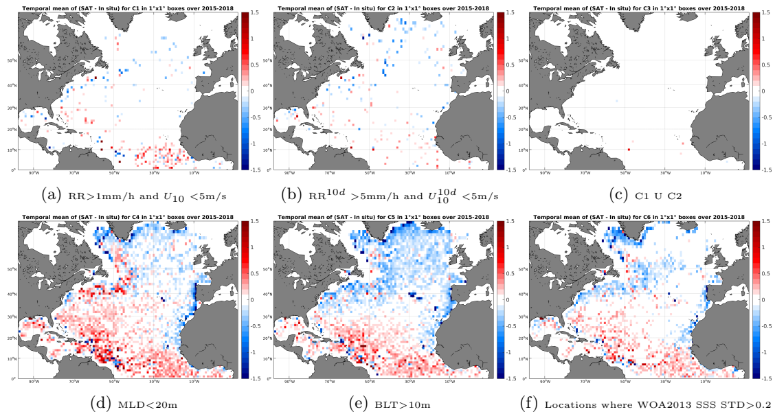
Figure 12: Temporal mean gridded over spatial boxes of size 1^\circ \times 1^\circ of \Delta SSS (SMAP-L3-RSS-V2-MONTHLY-70KM - Argo) for 6 different subdatasets corresponding to: RR > 1\text{mm/h} and U_{10} < 5\text{m/s} (a), RR^{10d} > 5\text{mm/h} and U_{10}^{10d} < 5\text{m/s} (b), C1 U C2 (c), MLD < 20\text{m} (d), BLT > 10\text{m} (e), Locations where WOA2013 SSS STD > 0.2 (f).
