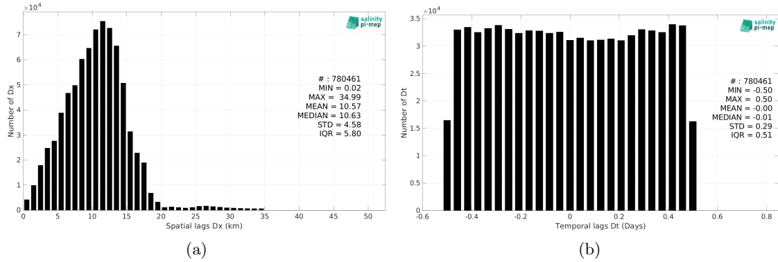
Figure 6: Histograms of the spatial (a) and temporal (b) lags between the location/time of the TSG (SAMOS) measurement and the date of the corresponding SMAP SSS L3 v5.0 - 8-Day running (JPL) SSS pixel.
