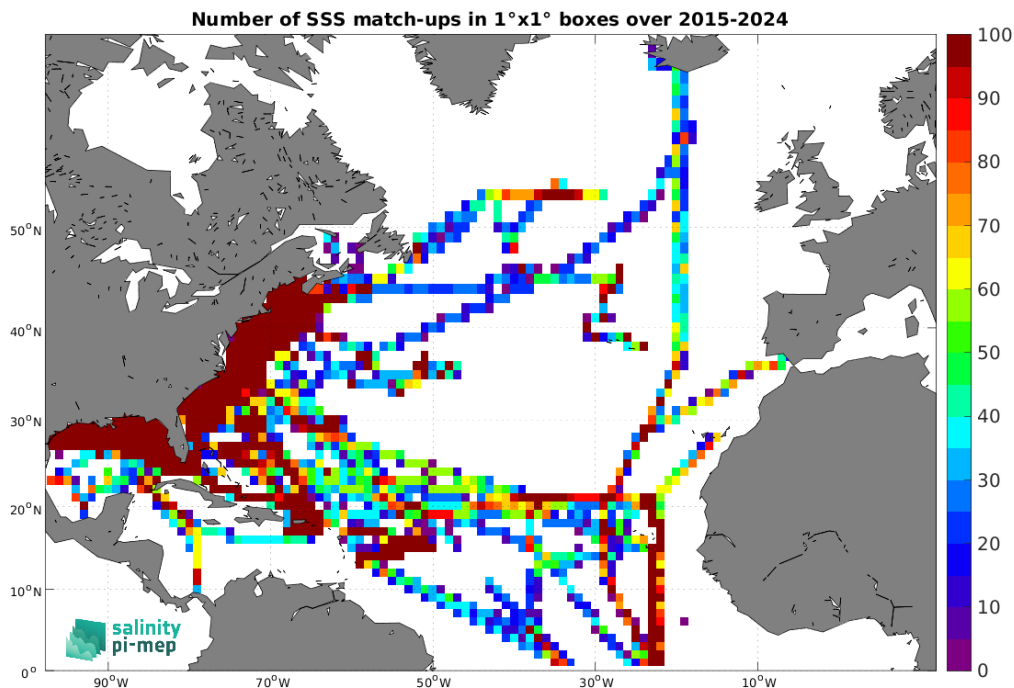
Figure 5: Number of SSS match-ups between TSG (SAMOS) SSS and the SMAP SSS L3 v5.0 - 8-Day running (JPL) SSS product for the North Atlantic Ocean Pi-MEP region over 1^\circ \times 1^\circ boxes and for the full satellite product period.
