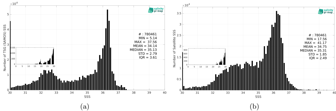
Figure 3: Histograms of SSS from TSG (SAMOS) (a) and SMAP SSS L3 v5.0 - 8-Day running (JPL) (b) considering all match-up pairs per bins of 0.1 over the North Atlantic Ocean Pi-MEP region and for the full satellite product period.
