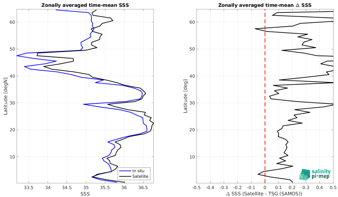
Figure 9: Left panel: Zonal mean SSS from SMAP SSS L3 v5.0 - 8-Day running (JPL) satellite product (black) and from TSG (SAMOS) (blue). Right panel: Zonal mean of \Delta SSS (Satellite - TSG (SAMOS)) for all the collected Pi-MEP match-up pairs estimated over the full satellite product period.
