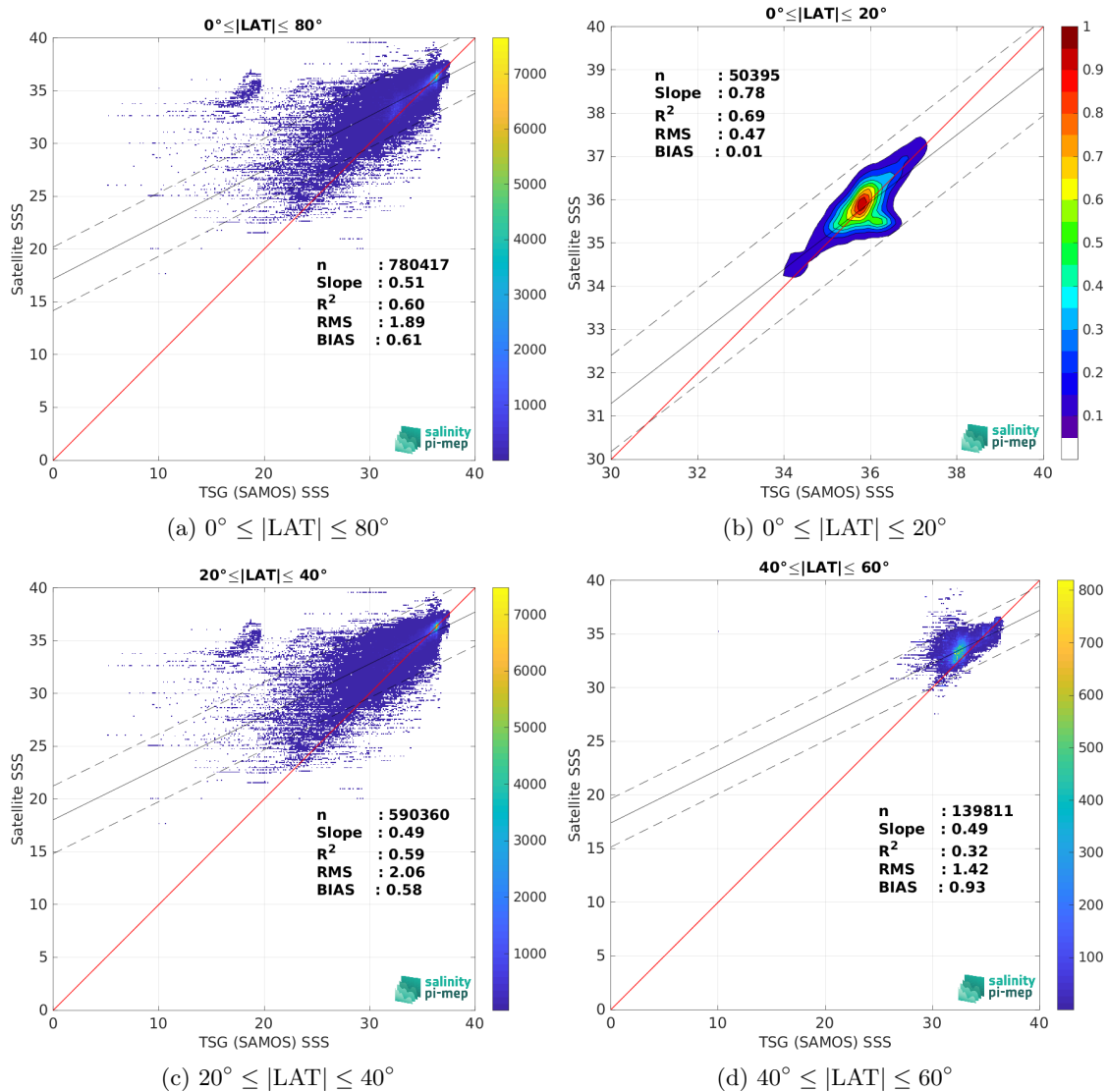
Figure 10: Contour maps of the concentration of SMAP SSS L3 v5.0 - 8-Day running (JPL) SSS (y-axis) versus TSG (SAMOS) SSS (x-axis) at match-up pairs for different latitude bands. For each plot, the red line shows x=y . The black thin and dashed lines indicate a linear fit through the data cloud and the \pm 95\% confidence levels, respectively. The number match-up pairs n , the slope and R^2 coefficient of the linear fit, the root mean square (RMS) and the mean bias between satellite and in situ data are indicated for each latitude band in each plots.
