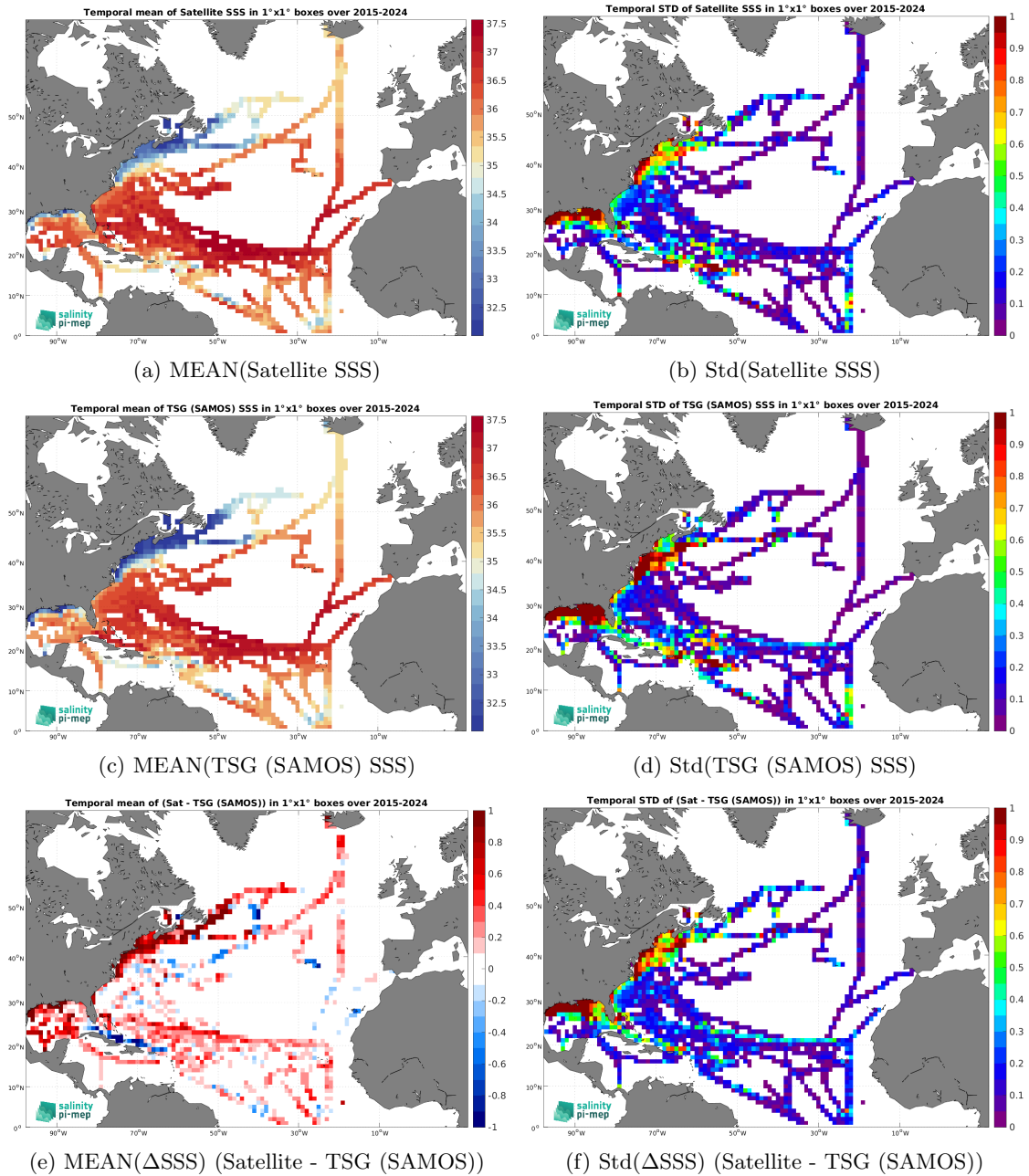
Figure 7: Temporal mean (left) and Std (right) of SSS from SMAP SSS L3 v5.0 - 8-Day running (JPL) (top), TSG (SAMOS) (middle), and of \Delta SSS (Satellite - TSG (SAMOS)). Only match-up pairs are used to generate these maps.
