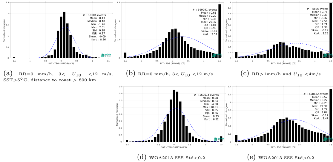
Figure 15: Normalized histogram of \Delta SSS (SMAP SSS L3 v5.0 - 8-Day running (JPL) - TSG (SAMOS)) for 5 different subdatasets corresponding to: RR=0 mm/h, 3 < U_{10} < 12 m/s, SST > 5°C, distance to coast > 800 km (a), RR=0 mm/h, 3 < U_{10} < 12 m/s (b), RR > 1mm/h and U_{10} < 4 m/s (c), WOA2013 SSS Std < 0.2 (d), WOA2013 SSS Std > 0.2 (e).
