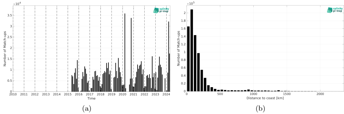
Figure 2: Number of match-ups between TSG (SAMOS) and SMAP SSS L3 v5.0 - 8-Day running (JPL) SSS as a function of time (a) and as function of the distance to coast (b) over the North Atlantic Ocean Pi-MEP region and for the full satellite product period.
