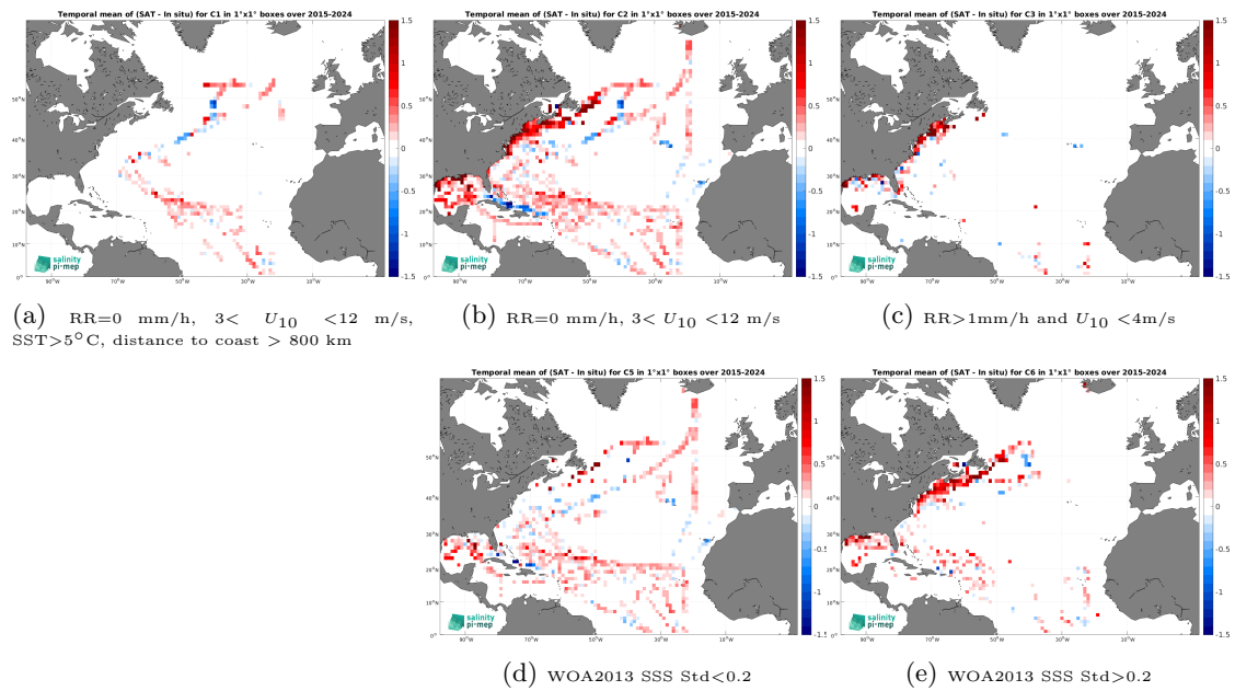
Figure 14: Temporal mean gridded over spatial boxes of size 1^\circ \times 1^\circ of \Delta\text{SSS} (SMAP SSS L3 v5.0 - 8-Day running (JPL) - TSG (SAMOS)) for 5 different subdatasets corresponding to:RR=0 mm/h, 3 < U_{10} < 12 m/s, SST > 5°C, distance to coast > 800 km (a), RR=0 mm/h, 3 < U_{10} < 12 m/s (b), RR > 1mm/h and U_{10} < 4 m/s (c), WOA2013 SSS Std < 0.2 (d), WOA2013 SSS Std > 0.2 (e).
