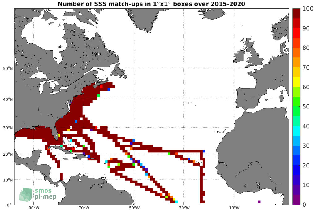
Figure 4: Number of SSS match-ups between TSG (SAMOS) SSS and the SMAP SSS L3 v5.0 - 8-Day running (JPL) SSS product for the North Atlantic Ocean Pi-MEP region over 1°x1° boxes and for the full satellite product period.
