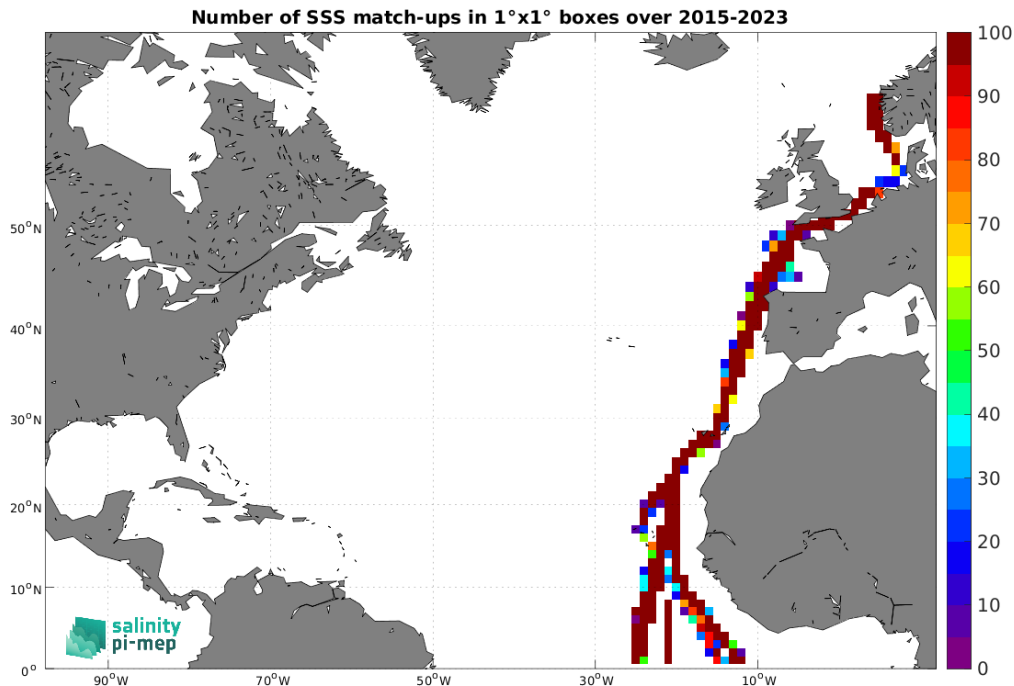
Figure 5: Number of SSS match-ups between TSG (Polarstern) SSS and the SMAP SSS L3 v5.0 - 8-Day running (JPL) SSS product for the North Atlantic Ocean Pi-MEP region over 1^\circ \times 1^\circ boxes and for the full satellite product period.
