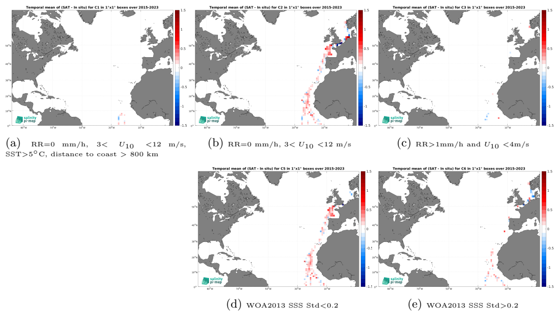
Figure 14: Temporal mean gridded over spatial boxes of size 1^\circ \times 1^\circ of \Delta\text{SSS} (SMAP SSS L3 v5.0 - 8-Day running (JPL) - TSG (Polarstern)) for 5 different subdatasets corresponding to:RR=0 mm/h, 3 < U_{10} < 12 m/s, SST > 5°C, distance to coast > 800 km (a), RR=0 mm/h, 3 < U_{10} < 12 m/s (b), RR > 1mm/h and U_{10} < 4 m/s (c), WOA2013 SSS Std < 0.2 (d), WOA2013 SSS Std > 0.2 (e).
