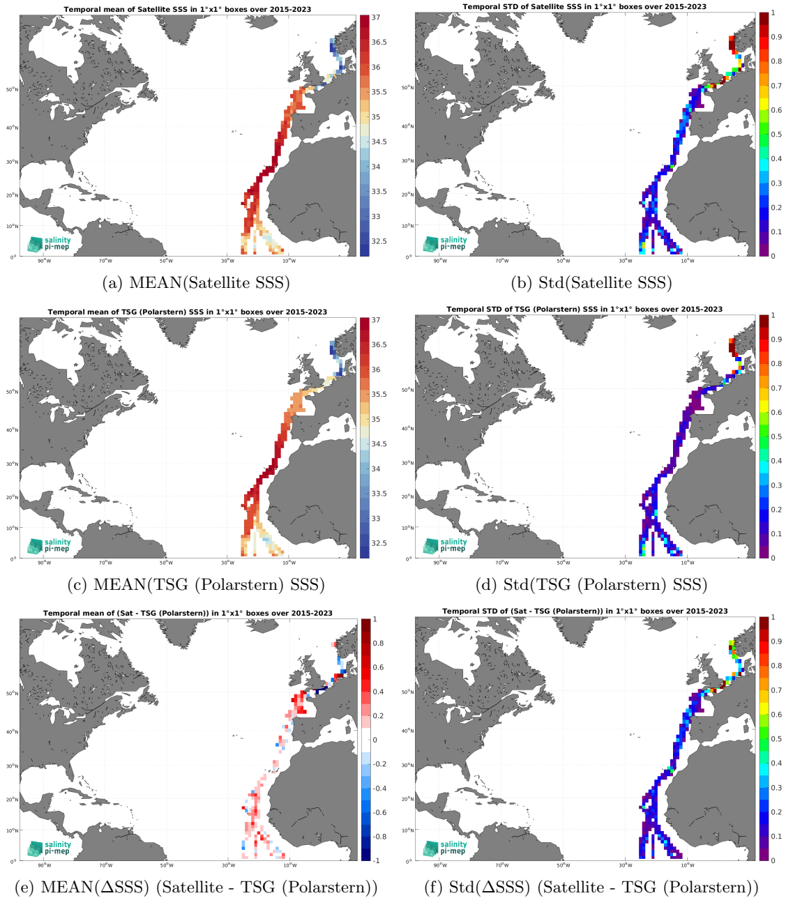
Figure 7: Temporal mean (left) and Std (right) of SSS from SMAP SSS L3 v5.0 - 8-Day running (JPL) (top), TSG (Polarstern) (middle), and of \Delta SSS (Satellite - TSG (Polarstern)). Only match-up pairs are used to generate these maps.
