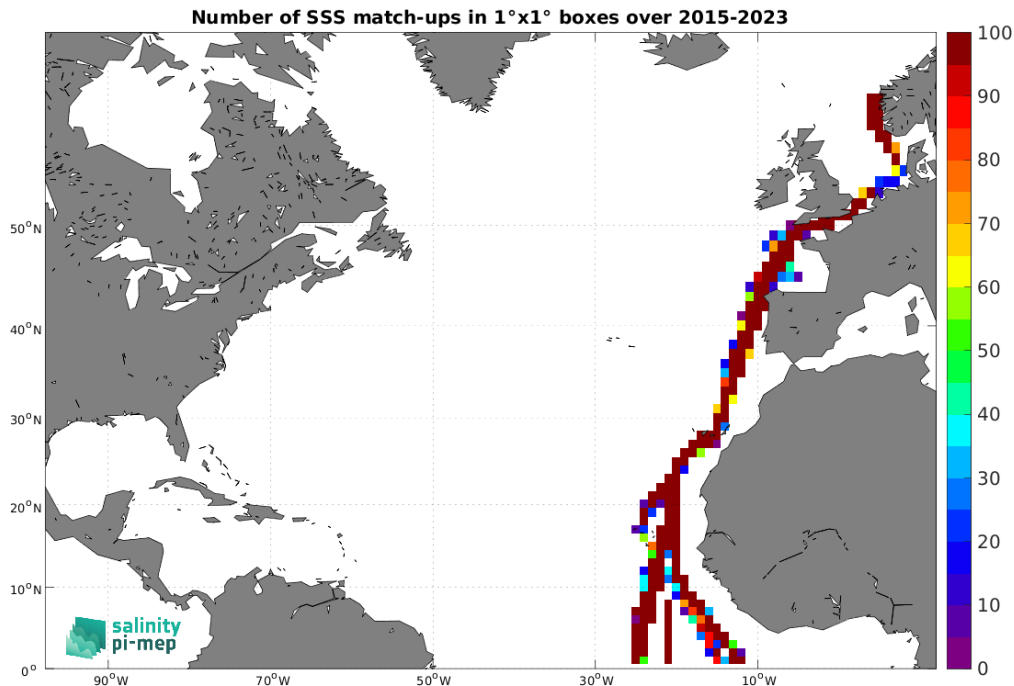
Figure 5: Number of SSS match-ups between TSG (Polarstern) SSS and the SMAP SSS L3 v5.0 - 8-Day running (JPL) SSS product for the North Atlantic Ocean Pi-MEP region over 1°×1° boxes and for the full satellite product period.
