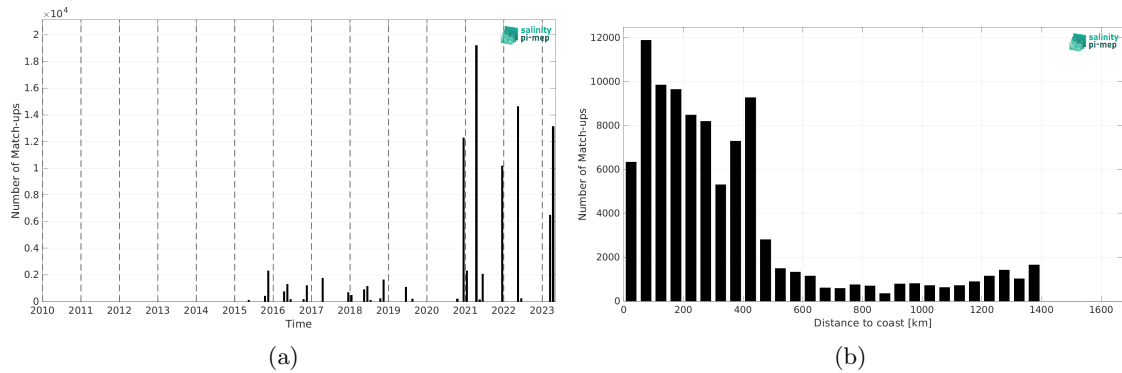
Figure 2: Number of match-ups between TSG (Polarstern) and SMAP SSS L3 v5.0 - 8-Day running (JPL) SSS as a function of time (a) and as function of the distance to coast (b) over the North Atlantic Ocean Pi-MEP region and for the full satellite product period.
