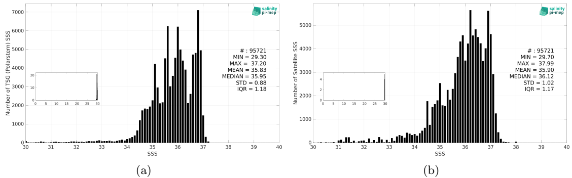
Figure 3: Histograms of SSS from TSG (Polarstern) (a) and SMAP SSS L3 v5.0 - 8-Day running (JPL) (b) considering all match-up pairs per bins of 0.1 over the North Atlantic Ocean Pi-MEP region and for the full satellite product period.
