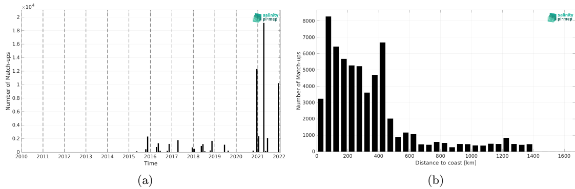
Figure 1: Number of match-ups between TSG (Polarstern) and SMAP SSS L3 v5.0 - 8-Day running (JPL) SSS as a function of time (a) and as function of the distance to coast (b) over the North Atlantic Ocean Pi-MEP region and for the full satellite product period.
