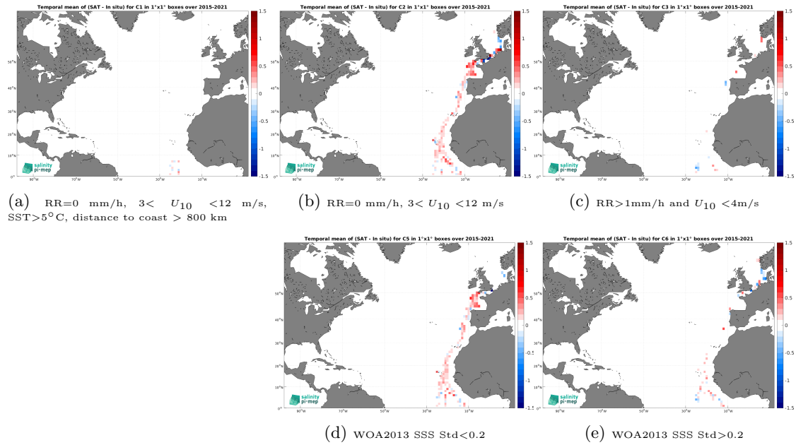
Figure 12: Temporal mean gridded over spatial boxes of size 1^\circ \times 1^\circ of \Delta\text{SSS} (SMAP SSS L3 v5.0 - 8-Day running (JPL) - TSG (Polarstern)) for 5 different subdatasets corresponding to:RR=0 mm/h, 3 < U_{10} < 12 m/s, SST >5^\circ\text{C} , distance to coast > 800 km (a), RR=0 mm/h, 3 < U_{10} < 12 m/s (b), RR >1 mm/h and U_{10} < 4 m/s (c), WOA2013 SSS Std <0.2 (d), WOA2013 SSS Std >0.2 (e).
