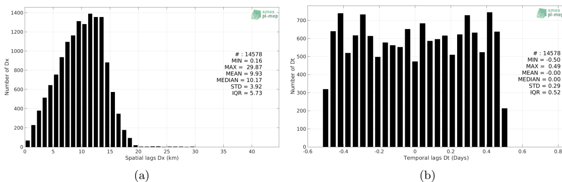
Figure 5: Histograms of the spatial (a) and temporal (b) lags between the time of the TSG (Polarstern) measurements and the date of the corresponding SMAP SSS L3 v5.0 - 8-Day running (JPL) SSS product.
