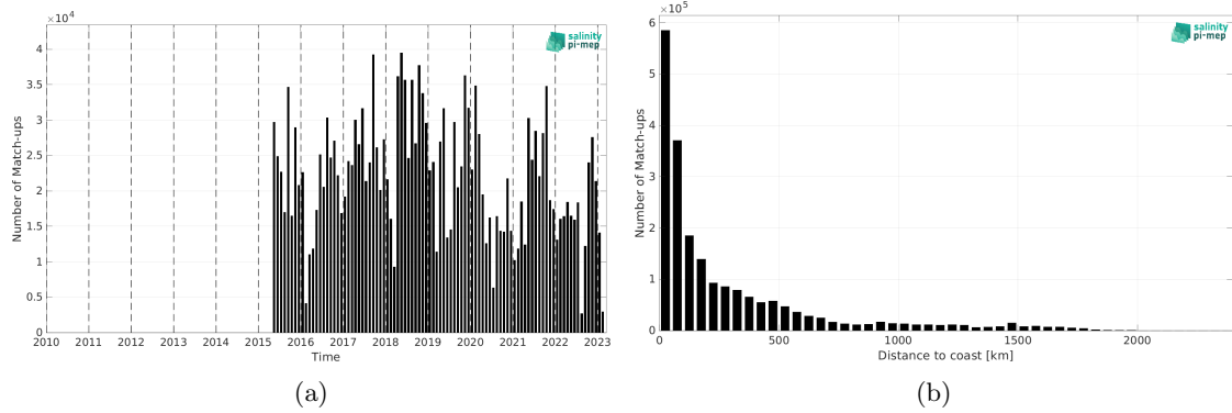
Figure 2: Number of match-ups between TSG (LEGOS-DM) and SMAP SSS L3 v5.0 - 8-Day running (JPL) SSS as a function of time (a) and as function of the distance to coast (b) over the North Atlantic Ocean Pi-MEP region and for the full satellite product period.
