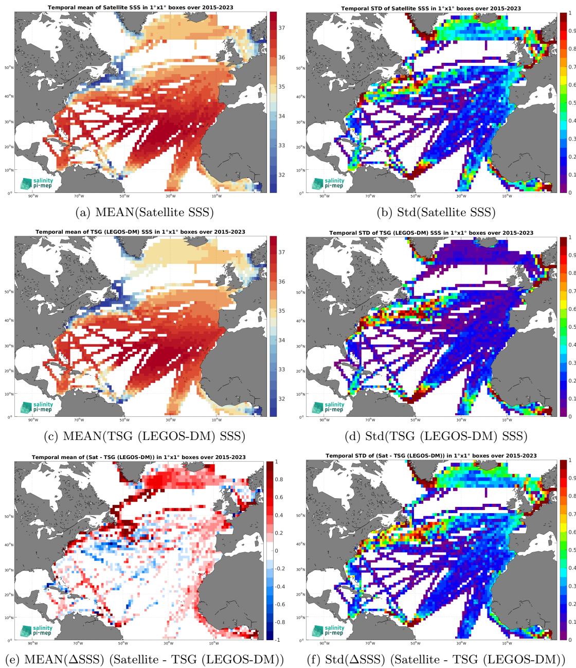
Figure 7: Temporal mean (left) and Std (right) of SSS from SMAP SSS L3 v5.0 - 8-Day running (JPL) (top), TSG (LEGOS-DM) (middle), and of \Delta SSS (Satellite - TSG (LEGOS-DM)). Only match-up pairs are used to generate these maps.
