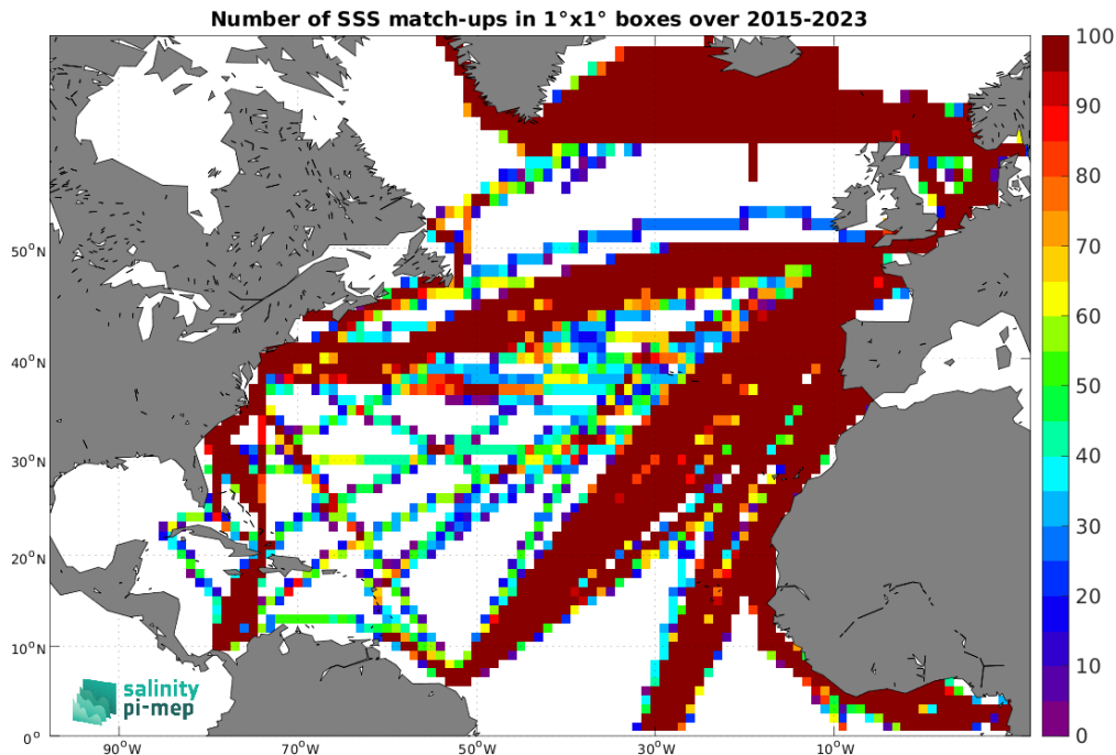
Figure 5: Number of SSS match-ups between TSG (LEGOS-DM) SSS and the SMAP SSS L3 v5.0 - 8-Day running (JPL) SSS product for the North Atlantic Ocean Pi-MEP region over 1°x1° boxes and for the full satellite product period.
