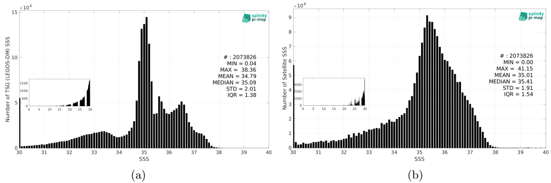
Figure 3: Histograms of SSS from TSG (LEGOS-DM) (a) and SMAP SSS L3 v5.0 - 8-Day running (JPL) (b) considering all match-up pairs per bins of 0.1 over the North Atlantic Ocean Pi-MEP region and for the full satellite product period.
