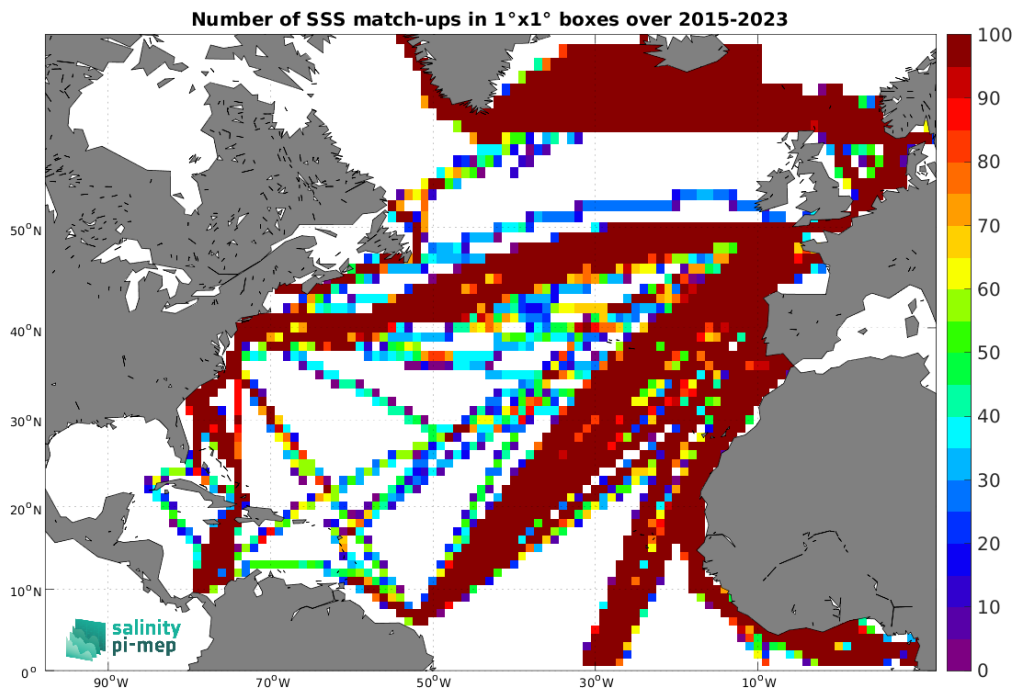
Figure 5: Number of SSS match-ups between TSG (LEGOS-DM) SSS and the SMAP SSS L3 v5.0 - 8-Day running (JPL) SSS product for the North Atlantic Ocean Pi-MEP region over 1^\circ \times 1^\circ boxes and for the full satellite product period.
