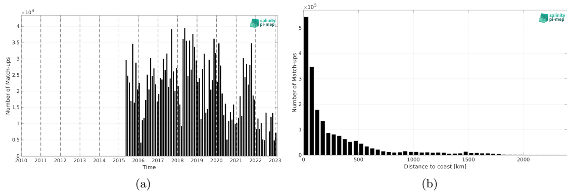
Figure 1: Number of match-ups between TSG (LEGOS-DM) and SMAP SSS L3 v5.0 - 8-Day running (JPL) SSS as a function of time (a) and as function of the distance to coast (b) over the North Atlantic Ocean Pi-MEP region and for the full satellite product period.
