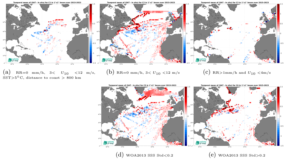
Figure 12: Temporal mean gridded over spatial boxes of size 1^\circ \times 1^\circ of \Delta\text{SSS} (SMAP SSS L3 v5.0 - 8-Day running (JPL) - TSG (LEGOS-DM)) for 5 different subdatasets corresponding to:RR=0 mm/h, 3 < U_{10} < 12 m/s, SST >5^\circ\text{C} , distance to coast > 800 km (a), RR=0 mm/h, 3 < U_{10} < 12 m/s (b), RR >1 mm/h and U_{10} < 4 m/s (c), WOA2013 SSS Std <0.2 (d), WOA2013 SSS Std >0.2 (e).
