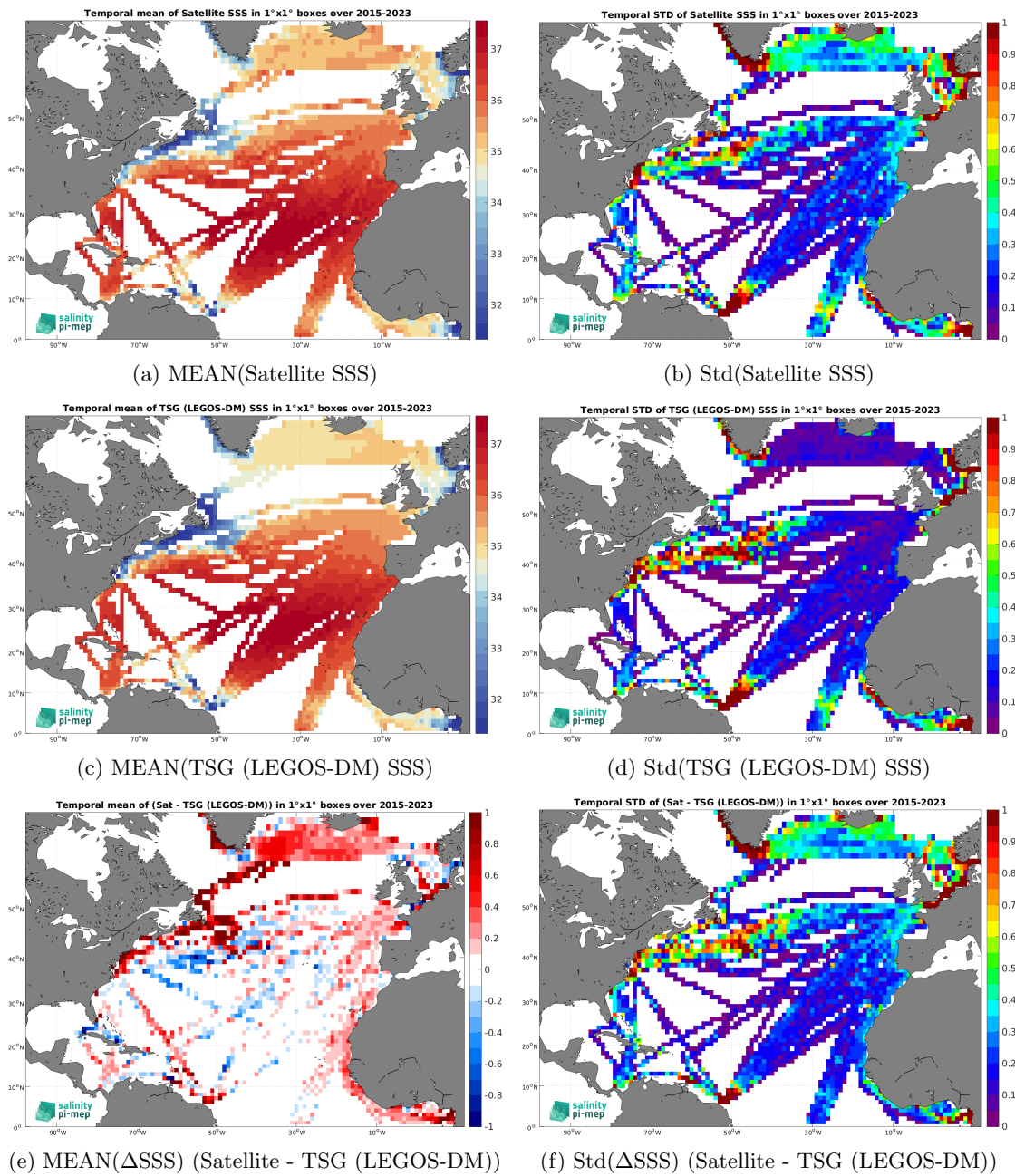
Figure 6: Temporal mean (left) and Std (right) of SSS from SMAP SSS L3 v5.0 - 8-Day running (JPL) (top), TSG (LEGOS-DM) (middle), and of \Delta SSS (Satellite - TSG (LEGOS-DM)). Only match-up pairs are used to generate these maps.
