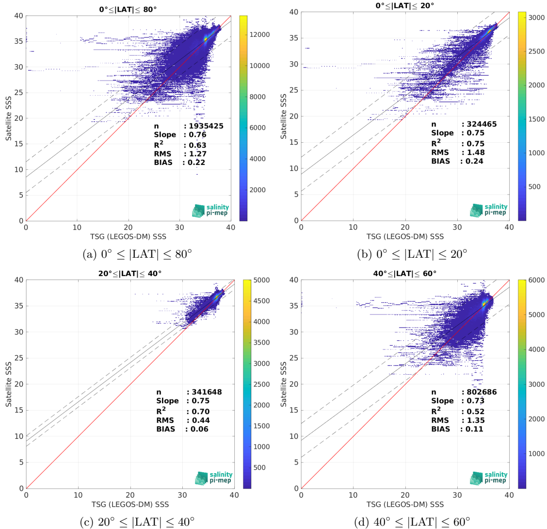
Figure 9: Contour maps of the concentration of SMAP SSS L3 v5.0 - 8-Day running (JPL) SSS (y-axis) versus TSG (LEGOS-DM) SSS (x-axis) at match-up pairs for different latitude bands. For each plot, the red line shows x=y . The black thin and dashed lines indicate a linear fit through the data cloud and the \pm 95\% confidence levels, respectively. The number match-up pairs n , the slope and R^2 coefficient of the linear fit, the root mean square (RMS) and the mean bias between satellite and in situ data are indicated for each latitude band in each plots.
