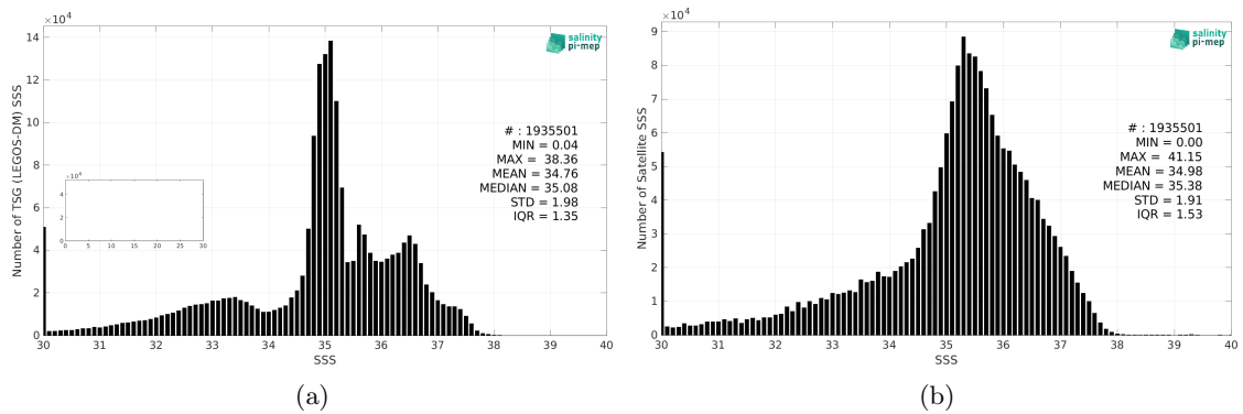
Figure 2: Histograms of SSS from TSG (LEGOS-DM) (a) and SMAP SSS L3 v5.0 - 8-Day running (JPL) (b) considering all match-up pairs per bins of 0.1 over the North Atlantic Ocean Pi-MEP region and for the full satellite product period.
