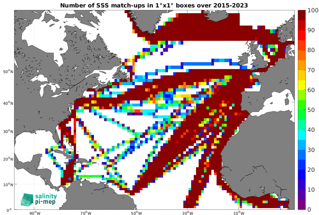
Figure 4: Number of SSS match-ups between TSG (LEGOS-DM) SSS and the SMAP SSS L3 v5.0 - 8-Day running (JPL) SSS product for the North Atlantic Ocean Pi-MEP region over 1°x1° boxes and for the full satellite product period.
