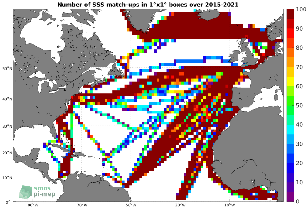
Figure 4: Number of SSS match-ups between TSG (LEGOS-DM) SSS and the SMAP SSS L3 v5.0 - 8-Day running (JPL) SSS product for the North Atlantic Ocean Pi-MEP region over 1^\circ \times 1^\circ boxes and for the full satellite product period.
