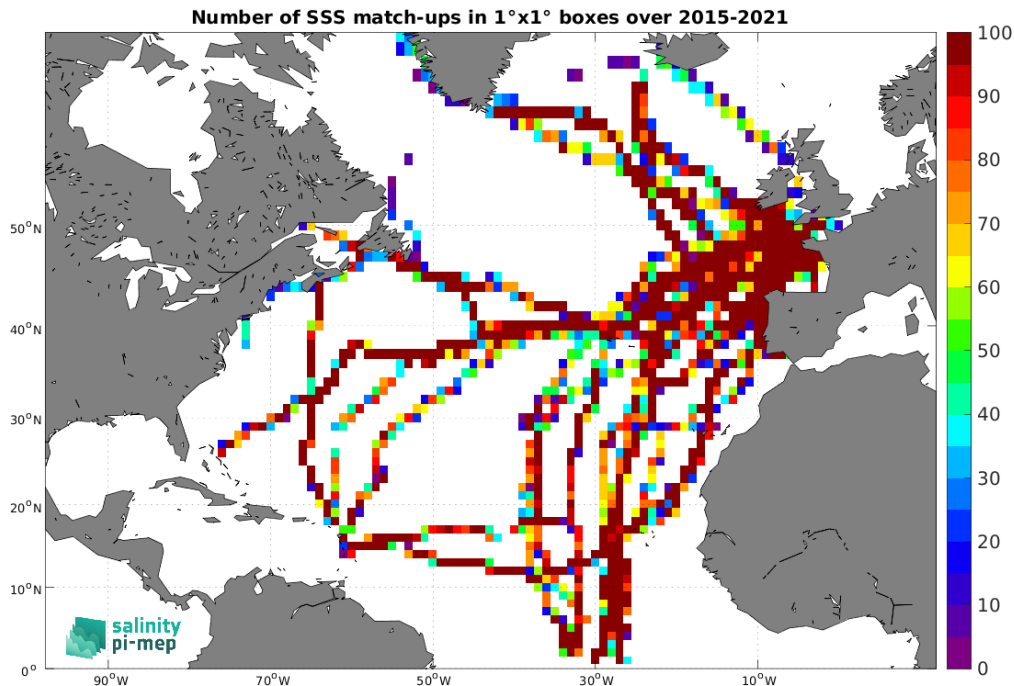
Figure 5: Number of SSS match-ups between TSG (GOSUD-Sailing-ship) SSS and the SMAP SSS L3 v5.0 - 8-Day running (JPL) SSS product for the North Atlantic Ocean Pi-MEP region over 1^\circ \times 1^\circ boxes and for the full satellite product period.
