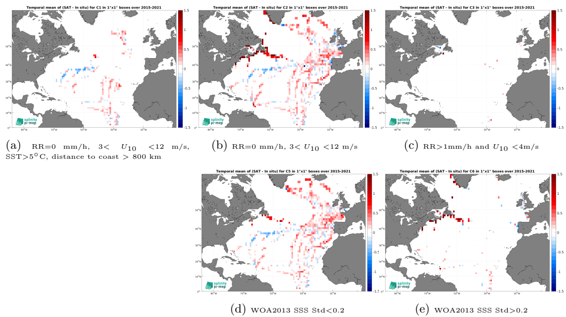
Figure 14: Temporal mean gridded over spatial boxes of size 1^\circ \times 1^\circ of \Delta\text{SSS} (SMAP SSS L3 v5.0 - 8-Day running (JPL) - TSG (GOSUD-Sailing-ship)) for 5 different subdatasets corresponding to:RR=0 mm/h, 3 < U_{10} < 12 m/s, SST >5^\circ\text{C} , distance to coast > 800 km (a), RR=0 mm/h, 3 < U_{10} < 12 m/s (b), RR >1 mm/h and U_{10} < 4 m/s (c), WOA2013 SSS Std <0.2 (d), WOA2013 SSS Std >0.2 (e).
