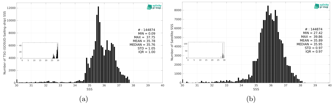
Figure 3: Histograms of SSS from TSG (GOSUD-Sailing-ship) (a) and SMAP SSS L3 v5.0 - 8-Day running (JPL) (b) considering all match-up pairs per bins of 0.1 over the North Atlantic Ocean Pi-MEP region and for the full satellite product period.
