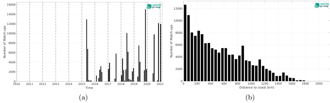
Figure 2: Number of match-ups between TSG (GOSUD-Sailing-ship) and SMAP SSS L3 v5.0 - 8-Day running (JPL) SSS as a function of time (a) and as function of the distance to coast (b) over the North Atlantic Ocean Pi-MEP region and for the full satellite product period.
