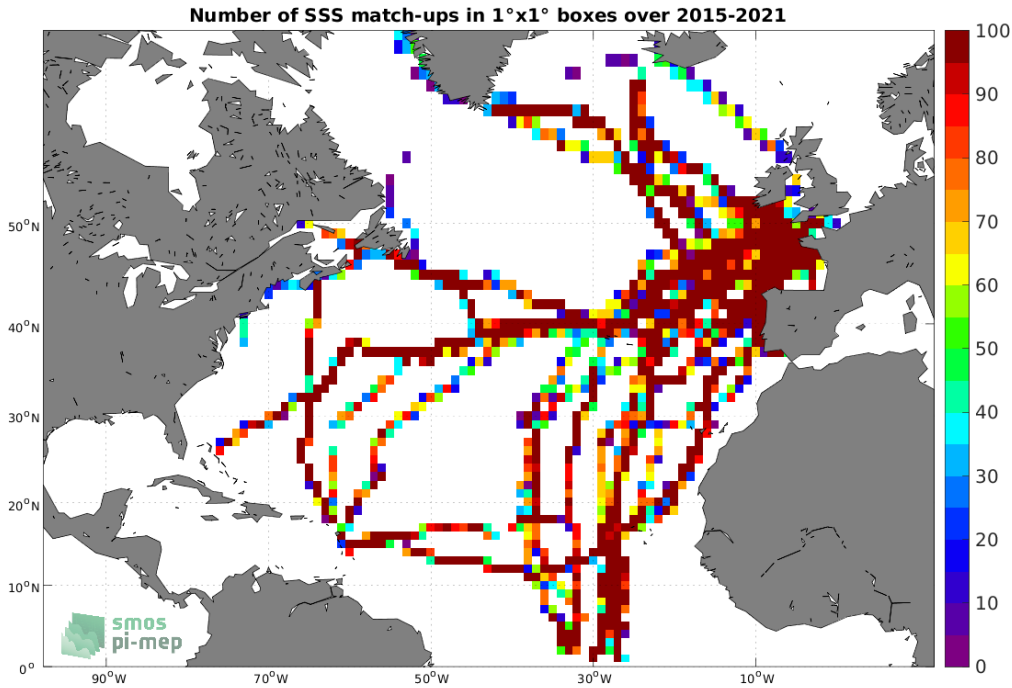
Figure 4: Number of SSS match-ups between TSG (GOSUD-Sailing-ship) SSS and the SMAP SSS L3 v5.0 - 8-Day running (JPL) SSS product for the North Atlantic Ocean Pi-MEP region over 1^\circ \times 1^\circ boxes and for the full satellite product period.
