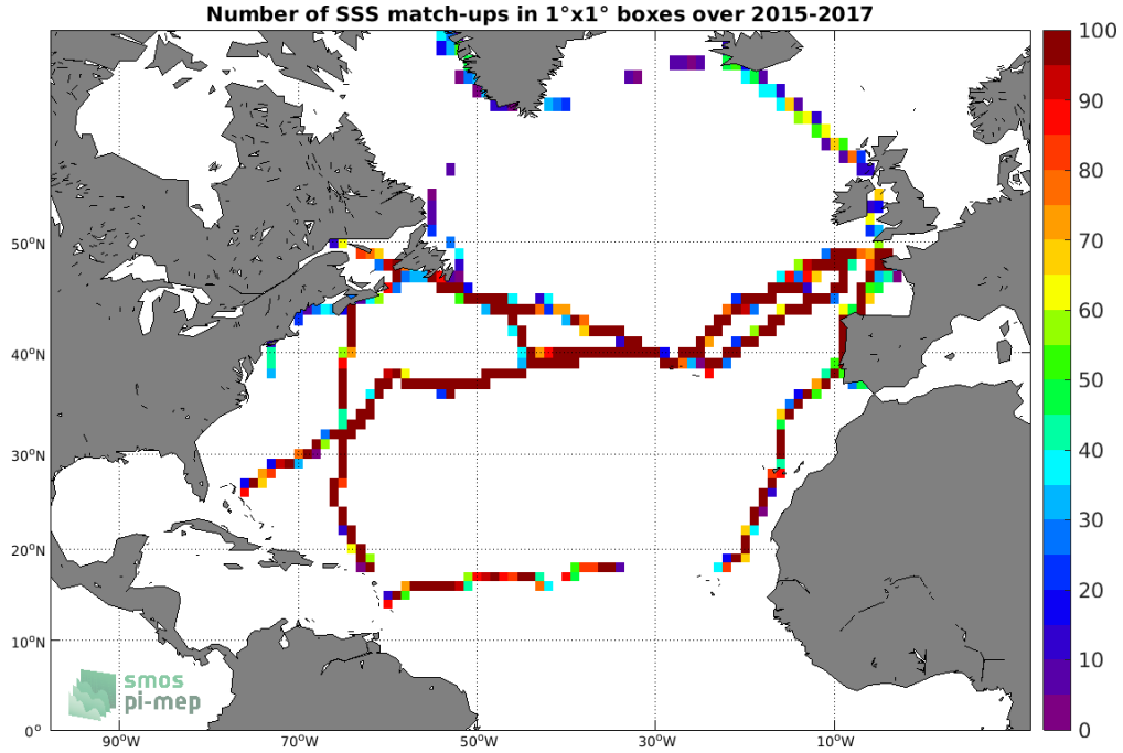
Figure 4: Number of SSS match-ups between TSG (GOSUD-Sailing-ship) SSS and the SMAP SSS L3 v5.0 - 8-Day running (JPL) SSS product for the North Atlantic Ocean Pi-MEP region over 1°x1° boxes and for the full satellite product period.
