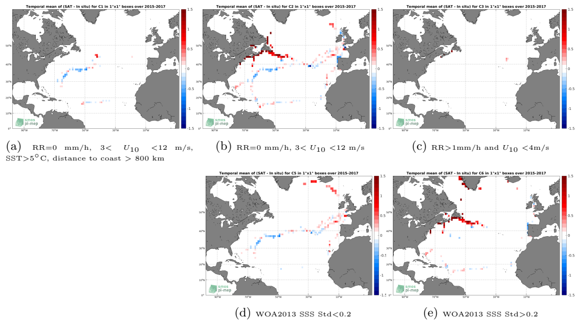
Figure 12: Temporal mean gridded over spatial boxes of size 1^\circ \times 1^\circ of \Delta\text{SSS} (SMAP SSS L3 v5.0 - 8-Day running (JPL) - TSG (GOSUD-Sailing-ship)) for 5 different subdatasets corresponding to: RR=0 mm/h, 3 < U_{10} < 12 m/s, SST > 5°C, distance to coast > 800 km (a), RR=0 mm/h, 3 < U_{10} < 12 m/s (b), RR > 1mm/h and U_{10} < 4 m/s (c), WOA2013 SSS Std < 0.2 (d), WOA2013 SSS Std > 0.2 (e).
