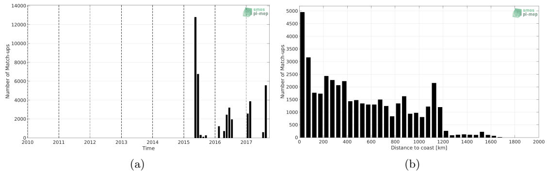
Figure 1: Number of match-ups between TSG (GOSUD-Sailing-ship) and SMAP SSS L3 v5.0 - 8-Day running (JPL) SSS as a function of time (a) and as function of the distance to coast (b) over the North Atlantic Ocean Pi-MEP region and for the full satellite product period.
