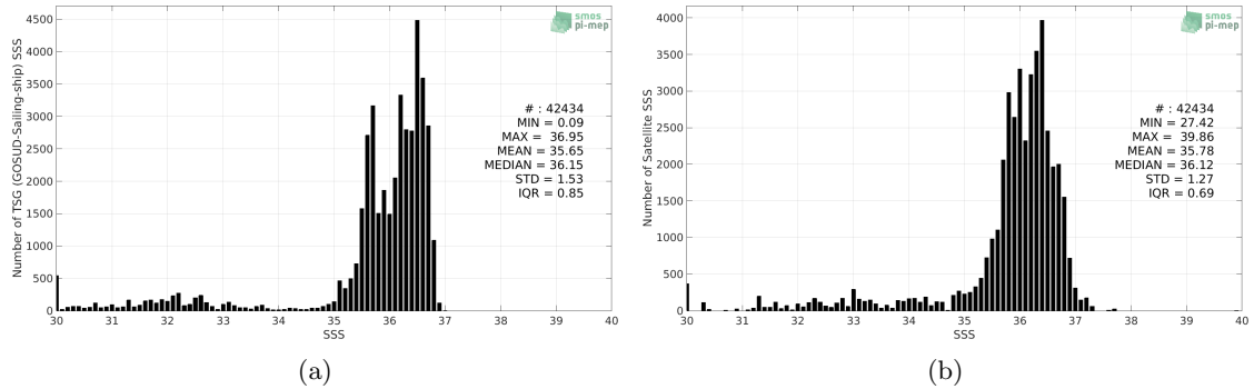
Figure 2: Histograms of SSS from TSG (GOSUD-Sailing-ship) (a) and SMAP SSS L3 v5.0 - 8-Day running (JPL) (b) considering all match-up pairs per bins of 0.1 over the North Atlantic Ocean Pi-MEP region and for the full satellite product period.
