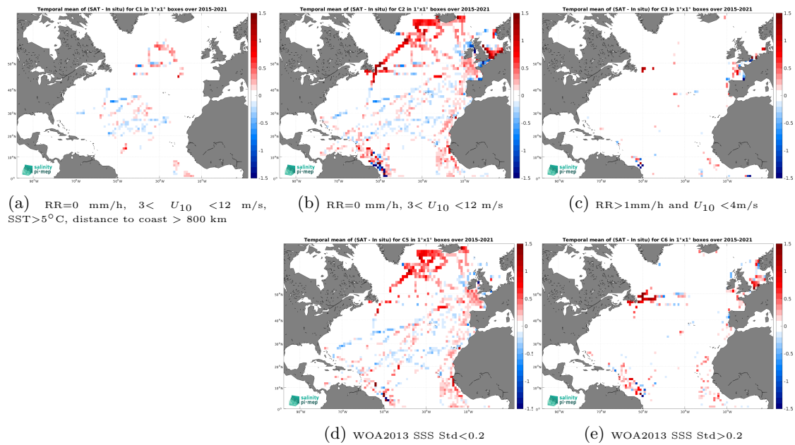
Figure 14: Temporal mean gridded over spatial boxes of size 1^\circ \times 1^\circ of \Delta\text{SSS} (SMAP SSS L3 v5.0 - 8-Day running (JPL) - TSG (GOSUD-Research-vessel)) for 5 different subdatasets corresponding to:RR=0 mm/h, 3 < U_{10} < 12 m/s, SST>5°C, distance to coast > 800 km (a), RR=0 mm/h, 3 < U_{10} < 12 m/s (b), RR>1mm/h and U_{10} < 4 m/s (c), WOA2013 SSS Std<0.2 (d), WOA2013 SSS Std>0.2 (e).
