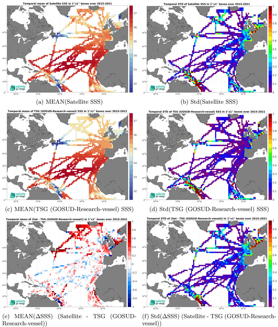
Figure 7: Temporal mean (left) and Std (right) of SSS from SMAP SSS L3 v5.0 - 8-Day running (JPL) (top), TSG (GOSUD-Research-vessel) (middle), and of \Delta SSS (Satellite - TSG (GOSUD-Research-vessel)). Only match-up pairs are used to generate these maps.
