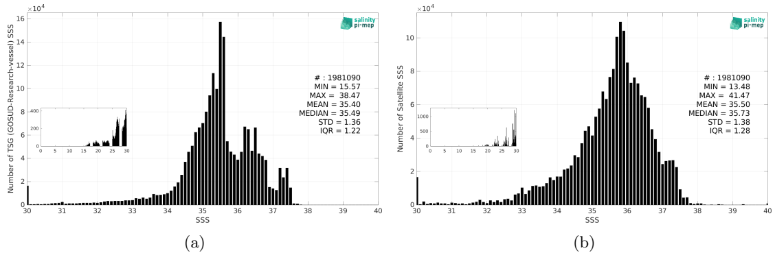
Figure 3: Histograms of SSS from TSG (GOSUD-Research-vessel) (a) and SMAP SSS L3 v5.0 - 8-Day running (JPL) (b) considering all match-up pairs per bins of 0.1 over the North Atlantic Ocean Pi-MEP region and for the full satellite product period.
