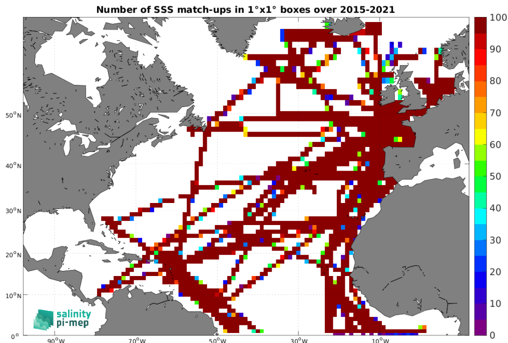
Figure 5: Number of SSS match-ups between TSG (GOSUD-Research-vessel) SSS and the SMAP SSS L3 v5.0 - 8-Day running (JPL) SSS product for the North Atlantic Ocean Pi-MEP region over 1^\circ \times 1^\circ boxes and for the full satellite product period.
