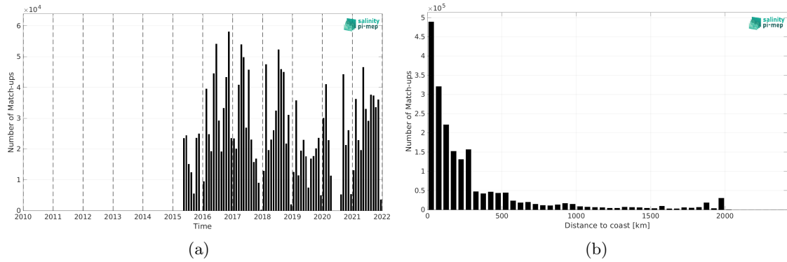
Figure 2: Number of match-ups between TSG (GOSUD-Research-vessel) and SMAP SSS L3 v5.0 - 8-Day running (JPL) SSS as a function of time (a) and as function of the distance to coast (b) over the North Atlantic Ocean Pi-MEP region and for the full satellite product period.
