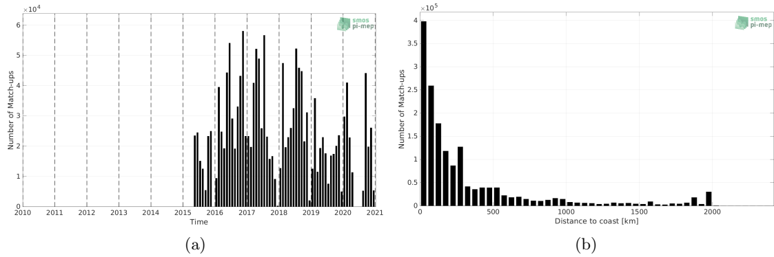
Figure 1: Number of match-ups between TSG (GOSUD-Research-vessel) and SMAP SSS L3 v5.0 - 8-Day running (JPL) SSS as a function of time (a) and as function of the distance to coast (b) over the North Atlantic Ocean Pi-MEP region and for the full satellite product period.
