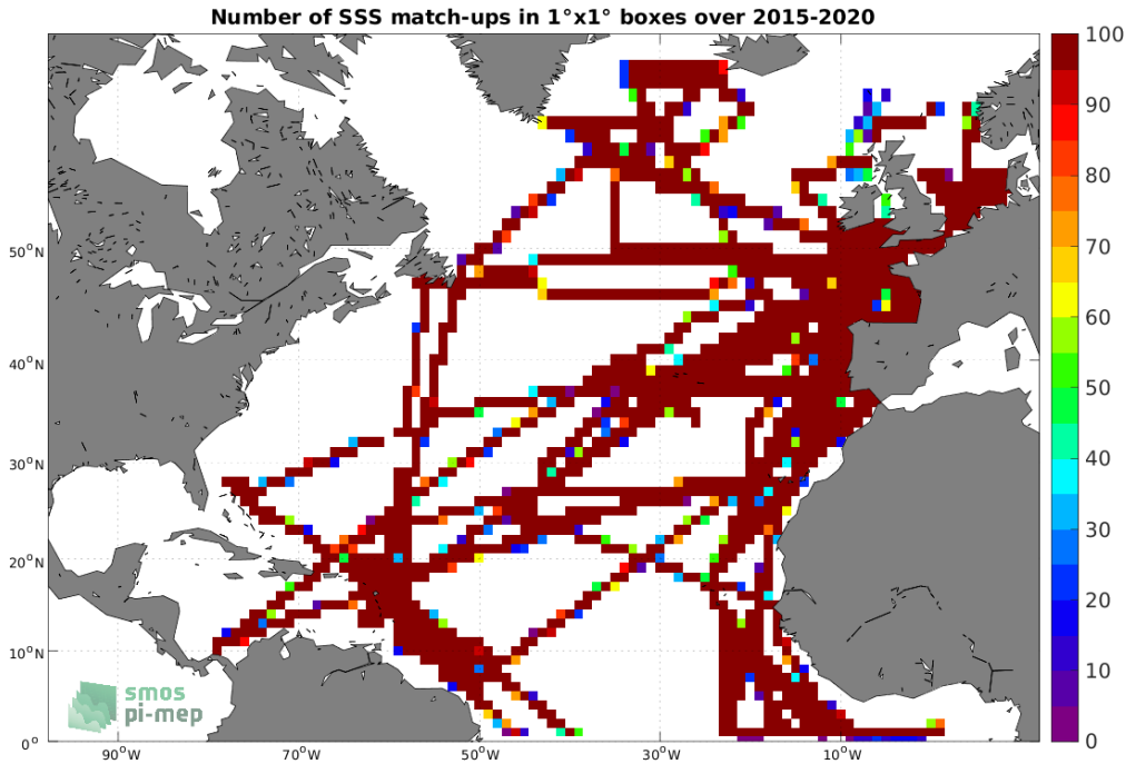
Figure 4: Number of SSS match-ups between TSG (GOSUD-Research-vessel) SSS and the SMAP SSS L3 v5.0 - 8-Day running (JPL) SSS product for the North Atlantic Ocean Pi-MEP region over 1°×1° boxes and for the full satellite product period.
