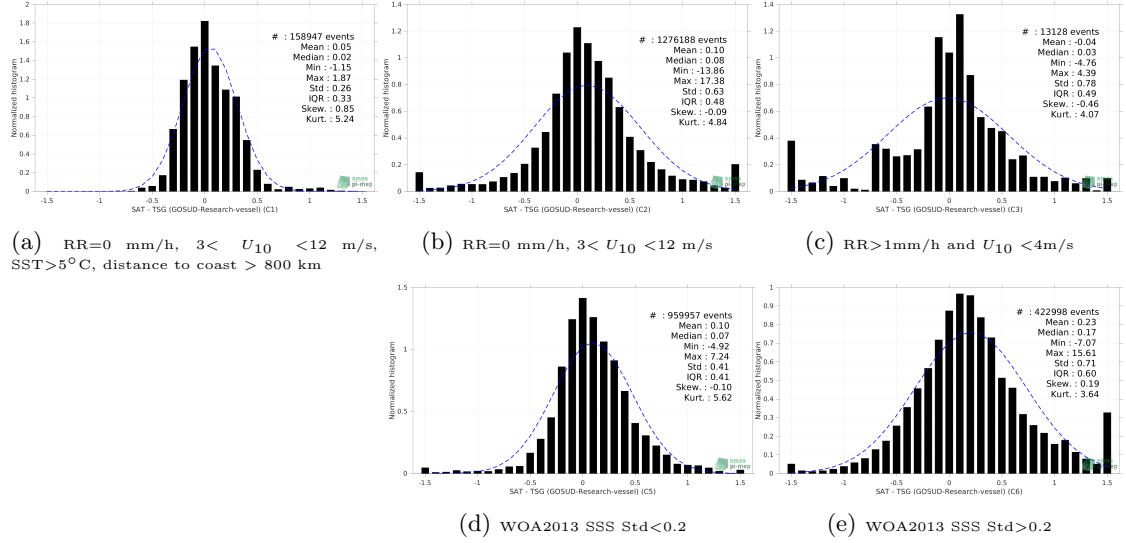
Figure 13: Normalized histogram of \Delta SSS (SMAP SSS L3 v5.0 - 8-Day running (JPL) - TSG (GOSUD-Research-vessel)) for 5 different subdatasets corresponding to: RR=0 mm/h, 3 < U_{10} < 12 m/s, SST > 5°C, distance to coast > 800 km (a), RR=0 mm/h, 3 < U_{10} < 12 m/s (b), RR > 1mm/h and U_{10} < 4 m/s (c), WOA2013 SSS Std < 0.2 (d), WOA2013 SSS Std > 0.2 (e).
