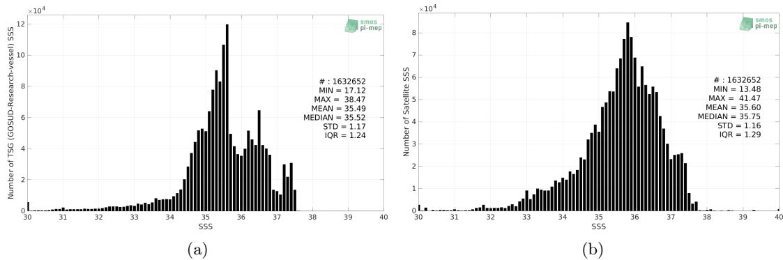
Figure 2: Histograms of SSS from TSG (GOSUD-Research-vessel) (a) and SMAP SSS L3 v5.0 - 8-Day running (JPL) (b) considering all match-up pairs per bins of 0.1 over the North Atlantic Ocean Pi-MEP region and for the full satellite product period.
