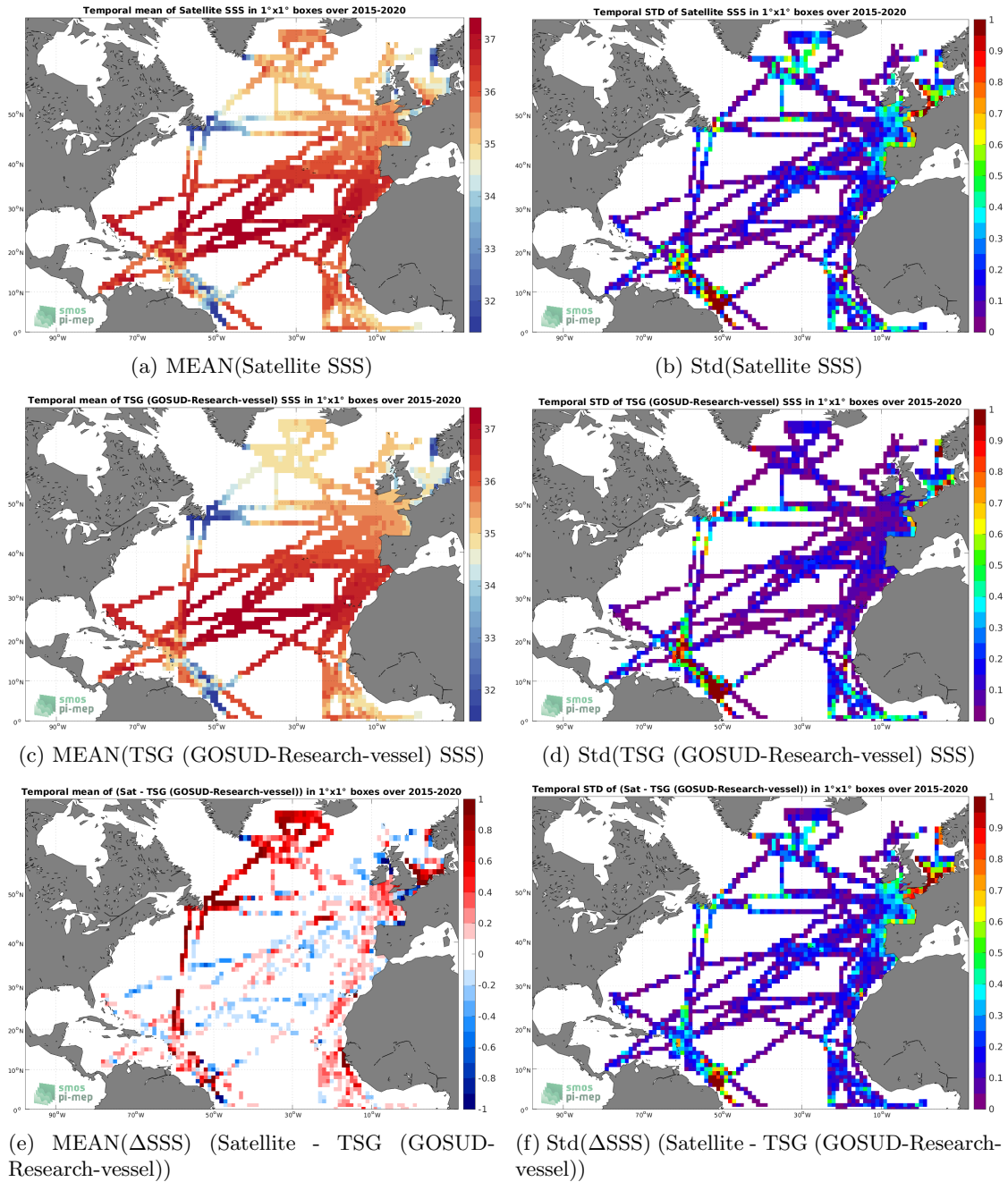
Figure 6: Temporal mean (left) and Std (right) of SSS from SMAP SSS L3 v5.0 - 8-Day running (JPL) (top), TSG (GOSUD-Research-vessel) (middle), and of \Delta SSS (Satellite - TSG (GOSUD-Research-vessel)). Only match-up pairs are used to generate these maps.
