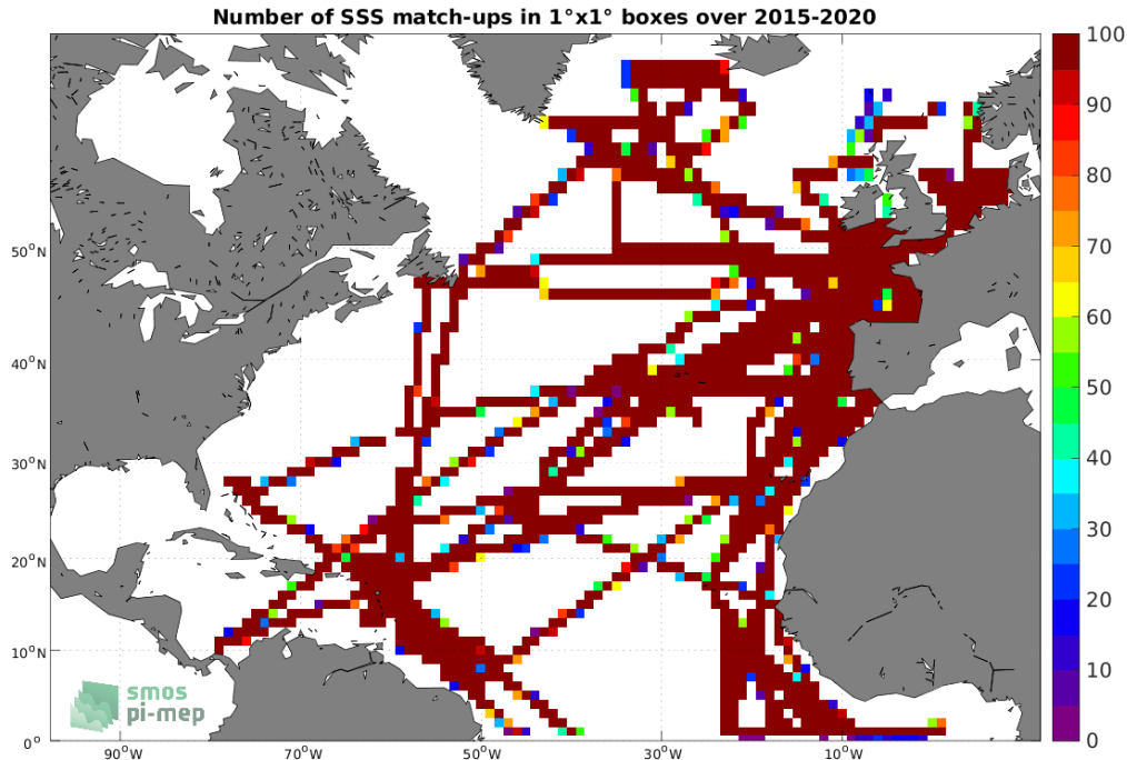
Figure 4: Number of SSS match-ups between TSG (GOSUD-Research-vessel) SSS and the SMAP SSS L3 v5.0 - 8-Day running (JPL) SSS product for the North Atlantic Ocean Pi-MEP region over 1^\circ \times 1^\circ boxes and for the full satellite product period.
