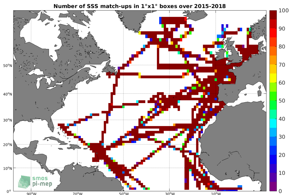
Figure 4: Number of SSS match-ups between TSG (GOSUD-Research-vessel) SSS and the SMAP SSS L3 v5.0 - 8-Day running (JPL) SSS product for the North Atlantic Ocean Pi-MEP region over 1°x1° boxes and for the full satellite product period.
