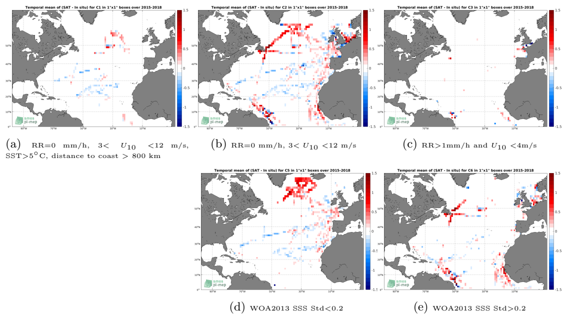
Figure 12: Temporal mean gridded over spatial boxes of size 1^\circ \times 1^\circ of \Delta\text{SSS} (SMAP SSS L3 v5.0 - 8-Day running (JPL) - TSG (GOSUD-Research-vessel)) for 5 different subdatasets corresponding to: RR=0 mm/h, 3 < U_{10} < 12 m/s, SST > 5°C, distance to coast > 800 km (a), RR=0 mm/h, 3 < U_{10} < 12 m/s (b), RR > 1mm/h and U_{10} < 4 m/s (c), WOA2013 SSS Std < 0.2 (d), WOA2013 SSS Std > 0.2 (e).
