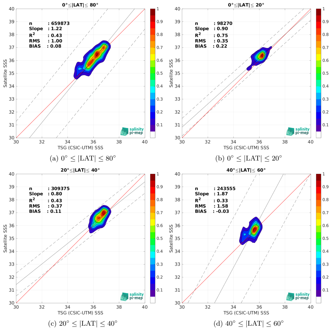
Figure 10: Contour maps of the concentration of SMAP SSS L3 v5.0 - 8-Day running (JPL) SSS (y-axis) versus TSG (CSIC-UTM) SSS (x-axis) at match-up pairs for different latitude bands. For each plot, the red line shows x=y . The black thin and dashed lines indicate a linear fit through the data cloud and the \pm 95\% confidence levels, respectively. The number match-up pairs n , the slope and R^2 coefficient of the linear fit, the root mean square (RMS) and the mean bias between satellite and in situ data are indicated for each latitude band in each plots.
