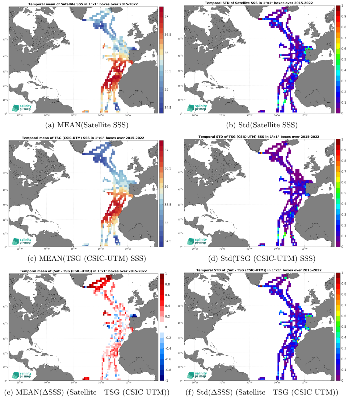
Figure 7: Temporal mean (left) and Std (right) of SSS from SMAP SSS L3 v5.0 - 8-Day running (JPL) (top), TSG (CSIC-UTM) (middle), and of \Delta SSS (Satellite - TSG (CSIC-UTM)). Only match-up pairs are used to generate these maps.
