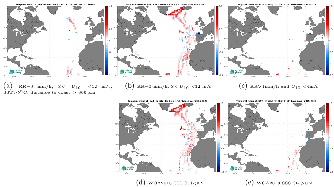
Figure 14: Temporal mean gridded over spatial boxes of size 1^\circ \times 1^\circ of \Delta\text{SSS} (SMAP SSS L3 v5.0 - 8-Day running (JPL) - TSG (CSIC-UTM)) for 5 different subdatasets corresponding to:RR=0 mm/h, 3 < U_{10} < 12 m/s, SST >5^\circ\text{C} , distance to coast > 800 km (a), RR=0 mm/h, 3 < U_{10} < 12 m/s (b), RR >1 mm/h and U_{10} < 4 m/s (c), WOA2013 SSS Std <0.2 (d), WOA2013 SSS Std >0.2 (e).
