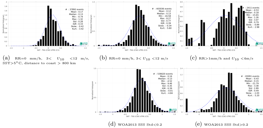
Figure 15: Normalized histogram of \Delta\text{SSS} (SMAP SSS L3 v5.0 - 8-Day running (JPL) - TSG (CSIC-UTM)) for 5 different subdatasets corresponding to: RR=0 mm/h, 3 < U_{10} < 12 m/s, SST>5°C, distance to coast > 800 km (a), RR=0 mm/h, 3 < U_{10} < 12 m/s (b), RR>1mm/h and U_{10} < 4 m/s (c), WOA2013 SSS Std<0.2 (d), WOA2013 SSS Std>0.2 (e).
