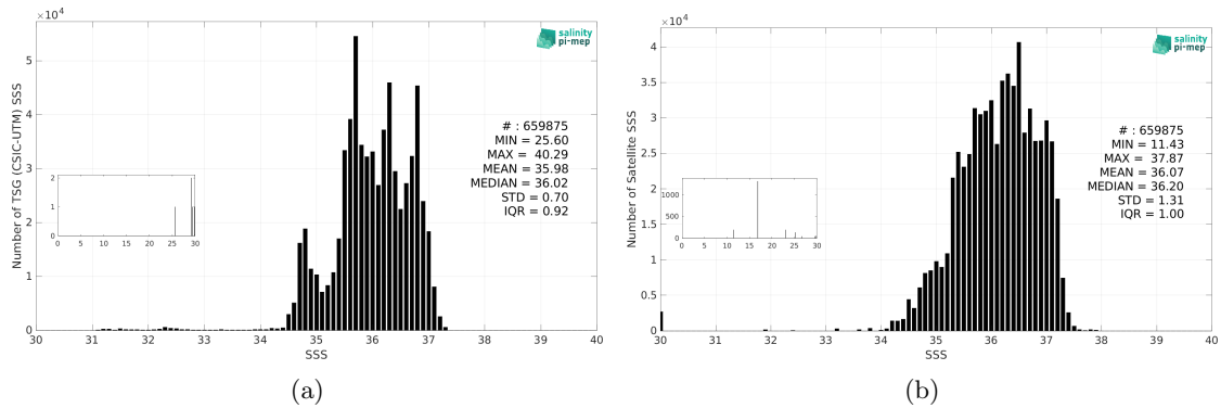
Figure 3: Histograms of SSS from TSG (CSIC-UTM) (a) and SMAP SSS L3 v5.0 - 8-Day running (JPL) (b) considering all match-up pairs per bins of 0.1 over the North Atlantic Ocean Pi-MEP region and for the full satellite product period.
