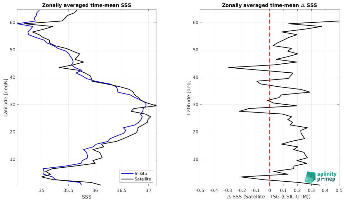
Figure 9: Left panel: Zonal mean SSS from SMAP SSS L3 v5.0 - 8-Day running (JPL) satellite product (black) and from TSG (CSIC-UTM) (blue). Right panel: Zonal mean of \Delta SSS (Satellite - TSG (CSIC-UTM)) for all the collected Pi-MEP match-up pairs estimated over the full satellite product period.
