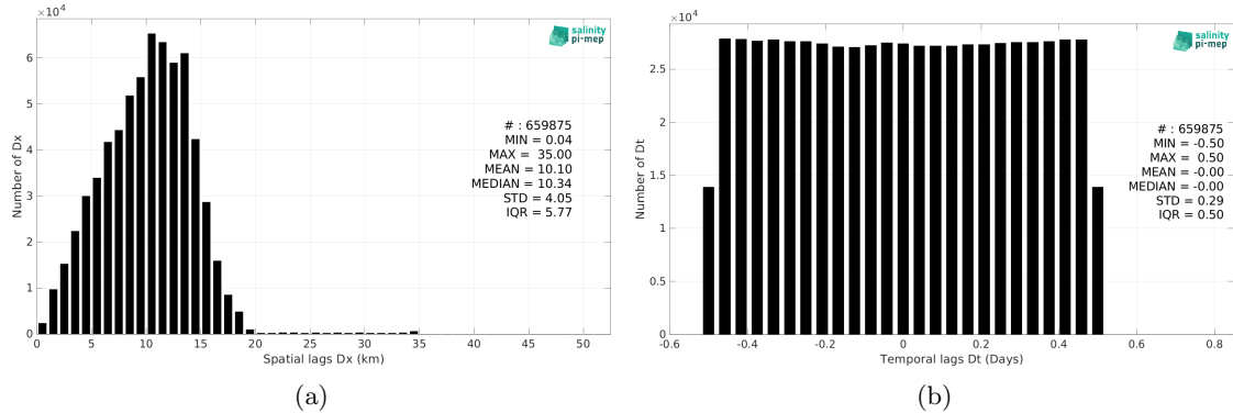
Figure 6: Histograms of the spatial (a) and temporal (b) lags between the location/time of the TSG (CSIC-UTM) measurement and the date of the corresponding SMAP SSS L3 v5.0 - 8-Day running (JPL) SSS pixel.
