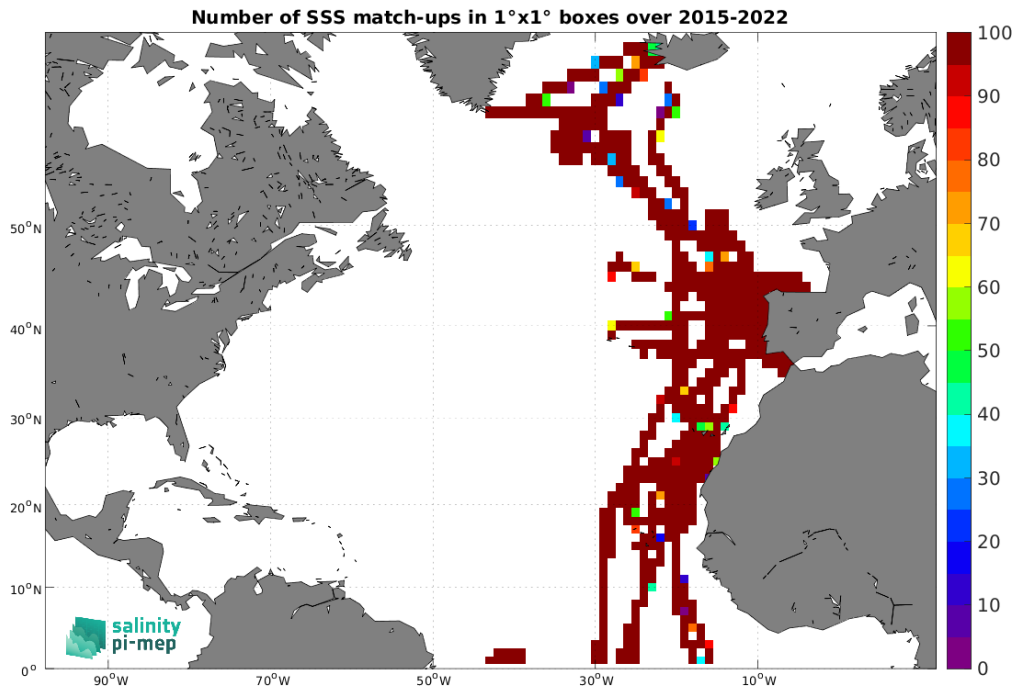
Figure 5: Number of SSS match-ups between TSG (CSIC-UTM) SSS and the SMAP SSS L3 v5.0 - 8-Day running (JPL) SSS product for the North Atlantic Ocean Pi-MEP region over 1^\circ \times 1^\circ boxes and for the full satellite product period.
