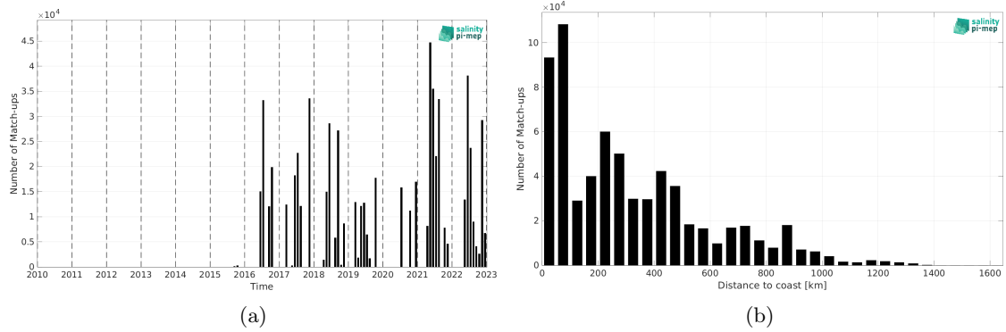
Figure 2: Number of match-ups between TSG (CSIC-UTM) and SMAP SSS L3 v5.0 - 8-Day running (JPL) SSS as a function of time (a) and as function of the distance to coast (b) over the North Atlantic Ocean Pi-MEP region and for the full satellite product period.
