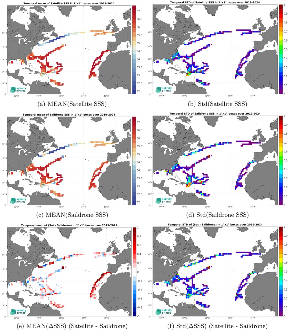
Figure 7: Temporal mean (left) and Std (right) of SSS from SMAP SSS L3 v5.0 - 8-Day running (JPL) (top), Saildrone (middle), and of \Delta SSS (Satellite - Saildrone). Only match-up pairs are used to generate these maps.
