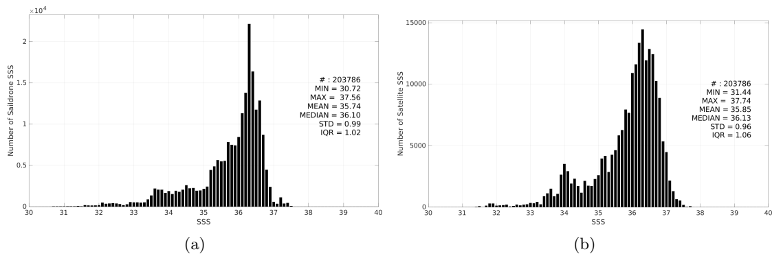
Figure 3: Histograms of SSS from Sairdrone (a) and SMAP SSS L3 v5.0 - 8-Day running (JPL) (b) considering all match-up pairs per bins of 0.1 over the North Atlantic Ocean Pi-MEP region and for the full satellite product period.
