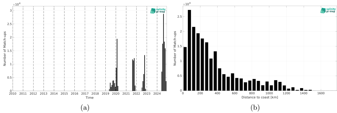
Figure 2: Number of match-ups between Sairdrone and SMAP SSS L3 v5.0 - 8-Day running (JPL) SSS as a function of time (a) and as function of the distance to coast (b) over the North Atlantic Ocean Pi-MEP region and for the full satellite product period.
