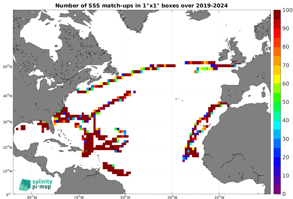
Figure 5: Number of SSS match-ups between Saildrone SSS and the SMAP SSS L3 v5.0 - 8-Day running (JPL) SSS product for the North Atlantic Ocean Pi-MEP region over 1^\circ \times 1^\circ boxes and for the full satellite product period.
