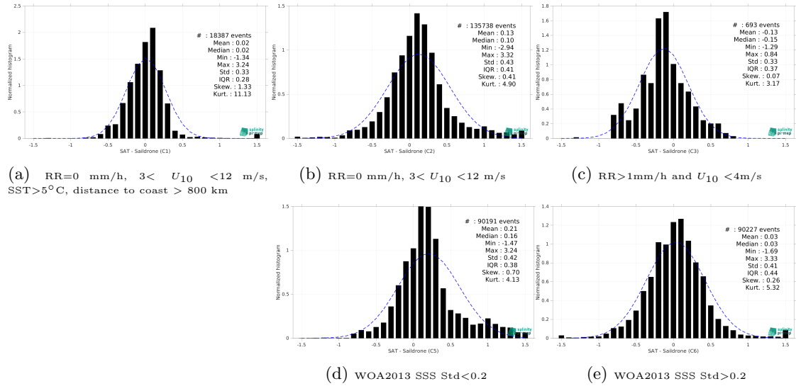
Figure 15: Normalized histogram of \Delta SSS (SMAP SSS L3 v5.0 - 8-Day running (JPL) - Saiclone) for 5 different subdatasets corresponding to: RR=0 mm/h, 3 < U_{10} < 12 m/s, SST>5°C, distance to coast > 800 km (a), RR=0 mm/h, 3 < U_{10} < 12 m/s (b), RR>1mm/h and U_{10} < 4 m/s (c), WOA2013 SSS Std<0.2 (d), WOA2013 SSS Std>0.2 (e).
