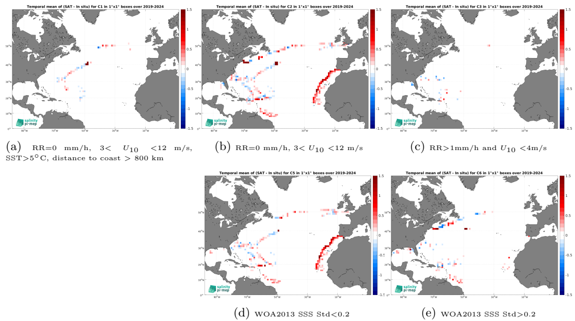
Figure 14: Temporal mean gridded over spatial boxes of size 1^\circ \times 1^\circ of \Delta\text{SSS} (SMAP SSS L3 v5.0 - 8-Day running (JPL) - Saildrone) for 5 different subdatasets corresponding to:RR=0 mm/h, 3 < U_{10} < 12 m/s, SST>5°C, distance to coast > 800 km (a), RR=0 mm/h, 3 < U_{10} < 12 m/s (b), RR>1mm/h and U_{10} < 4 m/s (c), WOA2013 SSS Std<0.2 (d), WOA2013 SSS Std>0.2 (e).
