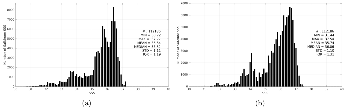
Figure 3: Histograms of SSS from Sairdrone (a) and SMAP SSS L3 v5.0 - 8-Day running (JPL) (b) considering all match-up pairs per bins of 0.1 over the North Atlantic Ocean Pi-MEP region and for the full satellite product period.
