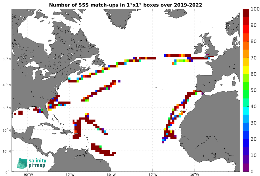
Figure 5: Number of SSS match-ups between Saildrone SSS and the SMAP SSS L3 v5.0 - 8-Day running (JPL) SSS product for the North Atlantic Ocean Pi-MEP region over 1°×1° boxes and for the full satellite product period.
