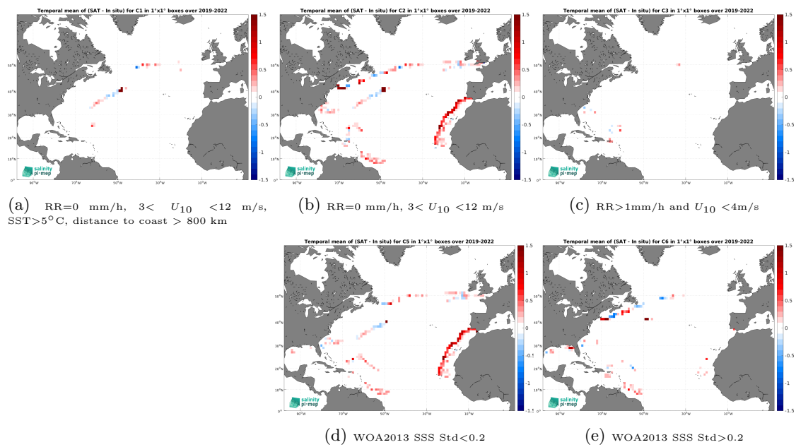
Figure 14: Temporal mean gridded over spatial boxes of size 1^\circ \times 1^\circ of \Delta\text{SSS} (SMAP SSS L3 v5.0 - 8-Day running (JPL) - Saifdrone) for 5 different subdatasets corresponding to:RR=0 mm/h, 3 < U_{10} < 12 m/s, SST >5^\circ\text{C} , distance to coast > 800 km (a), RR=0 mm/h, 3 < U_{10} < 12 m/s (b), RR >1 mm/h and U_{10} < 4 m/s (c), WOA2013 SSS Std <0.2 (d), WOA2013 SSS Std >0.2 (e).
