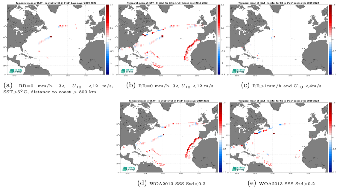
Figure 12: Temporal mean gridded over spatial boxes of size 1^\circ \times 1^\circ of \Delta\text{SSS} (SMAP SSS L3 v5.0 - 8-Day running (JPL) - Saifdrone) for 5 different subdatasets corresponding to:RR=0 mm/h, 3 < U_{10} < 12 m/s, SST >5^\circ\text{C} , distance to coast > 800 km (a), RR=0 mm/h, 3 < U_{10} < 12 m/s (b), RR >1 mm/h and U_{10} < 4 m/s (c), WOA2013 SSS Std <0.2 (d), WOA2013 SSS Std >0.2 (e).
