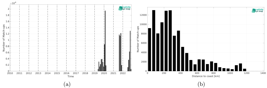
Figure 1: Number of match-ups between Sairdrone and SMAP SSS L3 v5.0 - 8-Day running (JPL) SSS as a function of time (a) and as function of the distance to coast (b) over the North Atlantic Ocean Pi-MEP region and for the full satellite product period.
