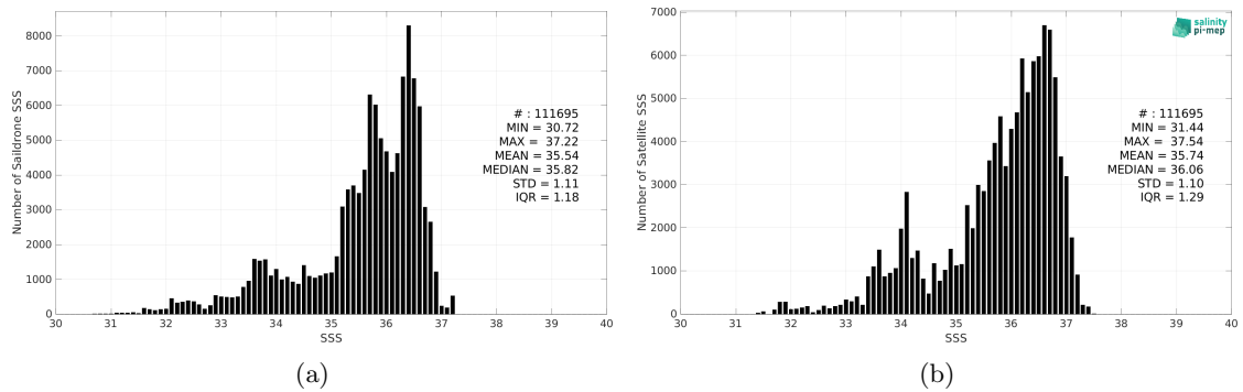
Figure 2: Histograms of SSS from Sairdrone (a) and SMAP SSS L3 v5.0 - 8-Day running (JPL) (b) considering all match-up pairs per bins of 0.1 over the North Atlantic Ocean Pi-MEP region and for the full satellite product period.
