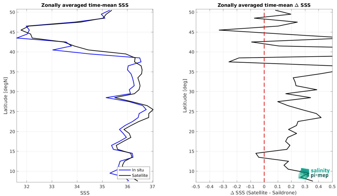
Figure 8: Left panel: Zonal mean SSS from SMAP SSS L3 v5.0 - 8-Day running (JPL) satellite product (black) and from Sairdronne (blue). Right panel: Zonal mean of \Delta SSS (Satellite - Sairdronne) for all the collected Pi-MEP match-up pairs estimated over the full satellite product period.
