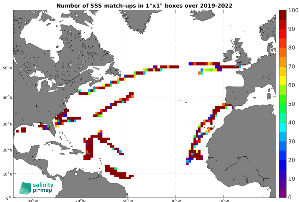
Figure 4: Number of SSS match-ups between Saildrone SSS and the SMAP SSS L3 v5.0 - 8-Day running (JPL) SSS product for the North Atlantic Ocean Pi-MEP region over 1°×1° boxes and for the full satellite product period.
