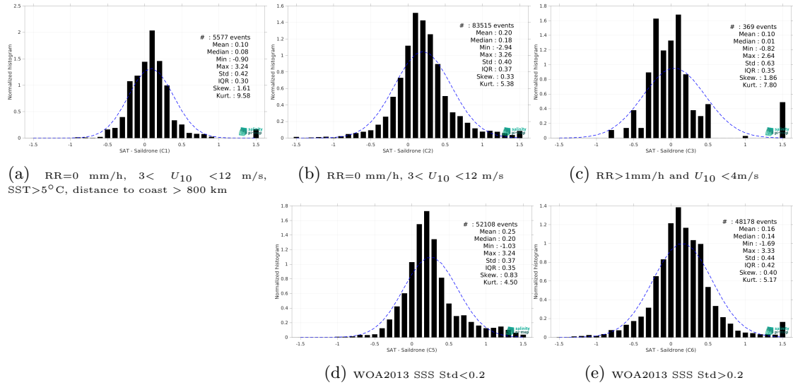
Figure 13: Normalized histogram of \Delta SSS (SMAP SSS L3 v5.0 - 8-Day running (JPL) - Saiclone) for 5 different subdatasets corresponding to: RR=0 mm/h, 3 < U_{10} < 12 m/s, SST>5°C, distance to coast > 800 km (a), RR=0 mm/h, 3 < U_{10} < 12 m/s (b), RR>1mm/h and U_{10} < 4 m/s (c), WOA2013 SSS Std<0.2 (d), WOA2013 SSS Std>0.2 (e).
